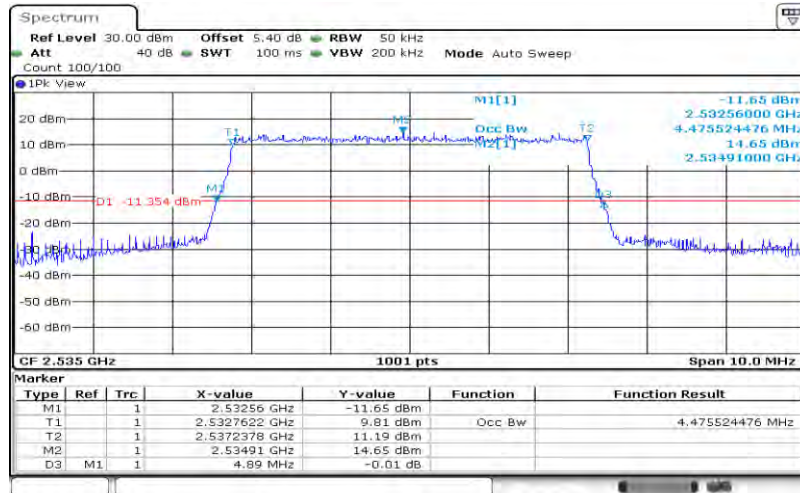
Band7-5MHz-QPSK-21100-25RB#0-4.476
