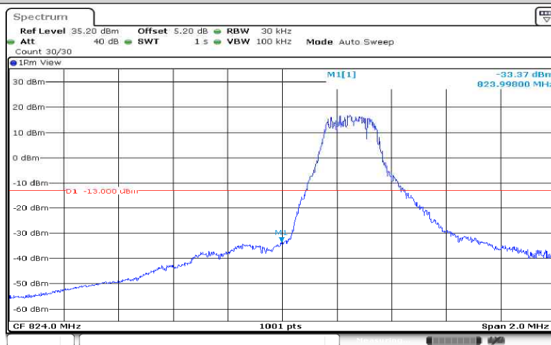
Band26-1.4MHz-QPSK-26797-1RB#0
