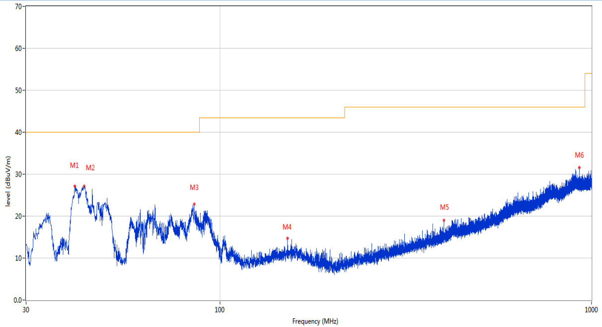
30 MHz to 1 GHz, ANT Vertical
