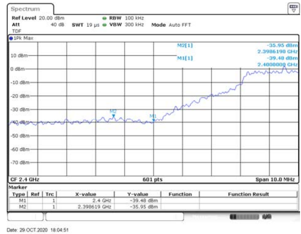
802.11ac-20 MHz LOW CHANNEL, Reference level
