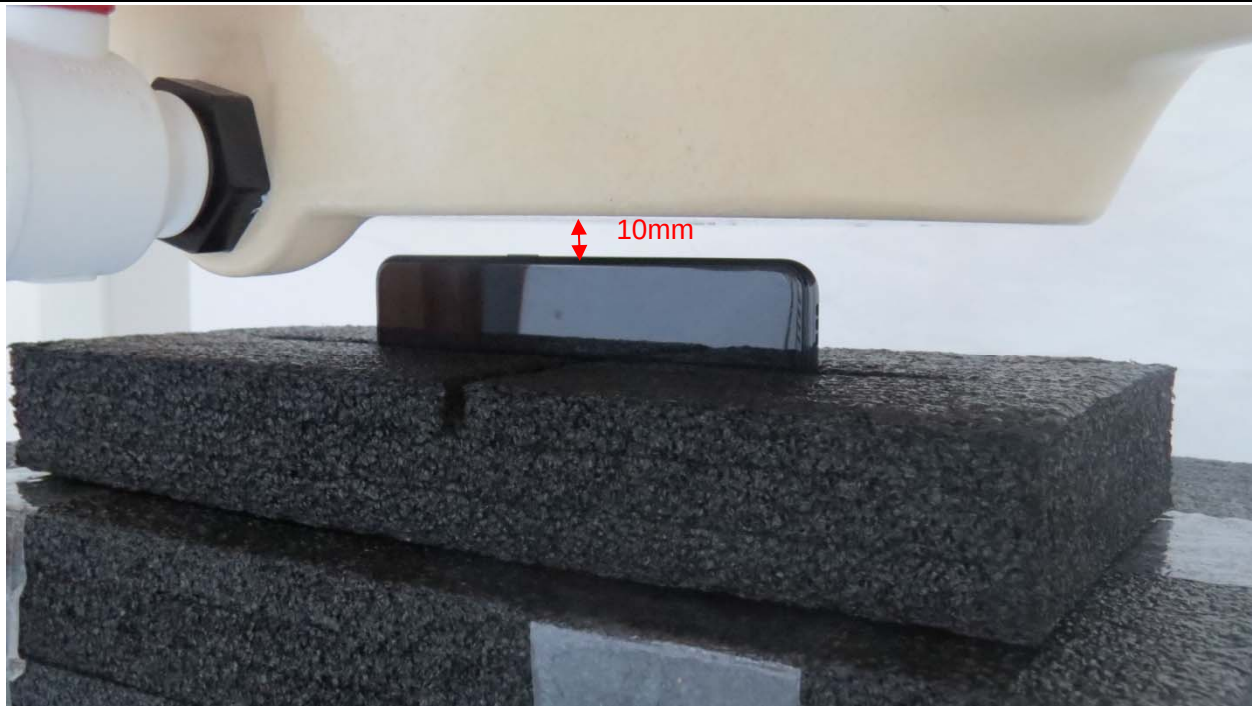
Picture 13: Right Side, the distance from handset to the bottom of the Phantom is 10mm
