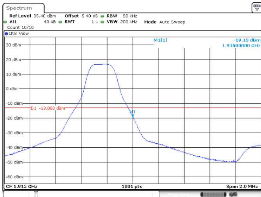
Band25-3MHz-64QAM-26675-1RB#14
