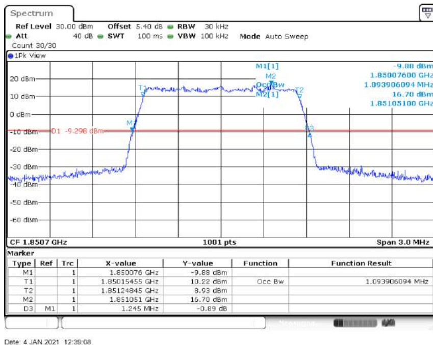
Band25-1.4MHz-64QAM-26365-6RB#0-1.094
