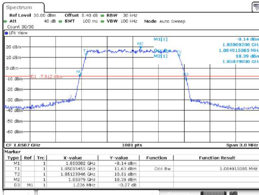
Band25-1.4MHz-QPSK-26047-6RB#0-1.085
