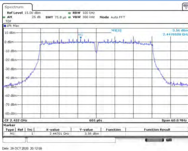
802.11ac-40 MHz HIGH CHANNEL, Carrier level
