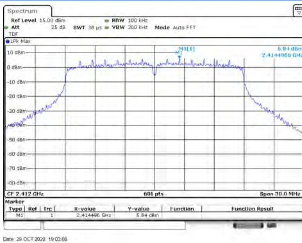
802.11ac-20 MHz LOW CHANNEL, Carrier level
