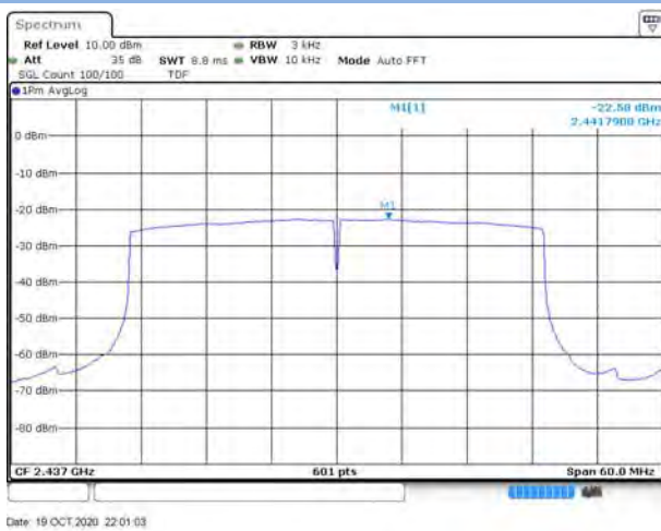
802.11ax-40 MHz (SU) MIDDLE CHANNEL
