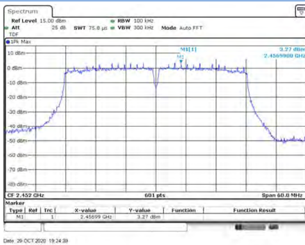
802.11ac-40 MHz HIGH CHANNEL, Carrier level
