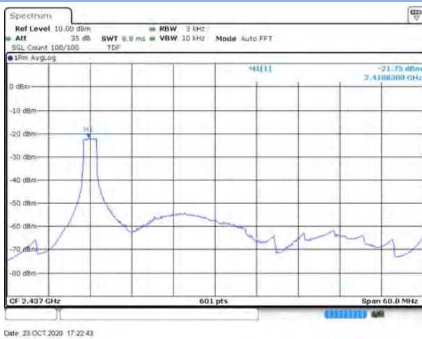
802.11ax-40 MHz (RU26) MIDDLE CHANNEL
