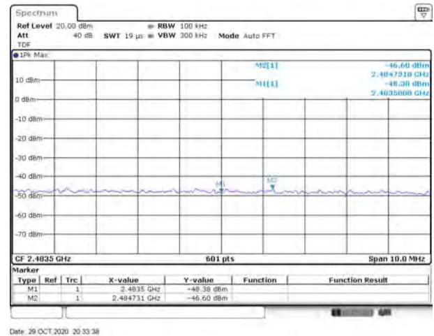
802.11ac-40 MHz HIGH CHANNEL, Reference level
