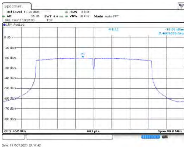
802.11ax-20 MHz (SU) HIGH CHANNEL
