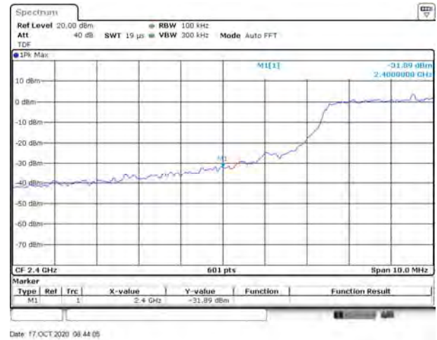
802.11ax-20 MHz (SU) MHz LOW CHANNEL, Reference level
