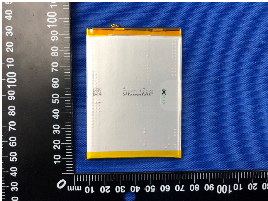
Battery Photo (BLP839 (Dongguan NVT Technology Co., Ltd.)) (REAR)
