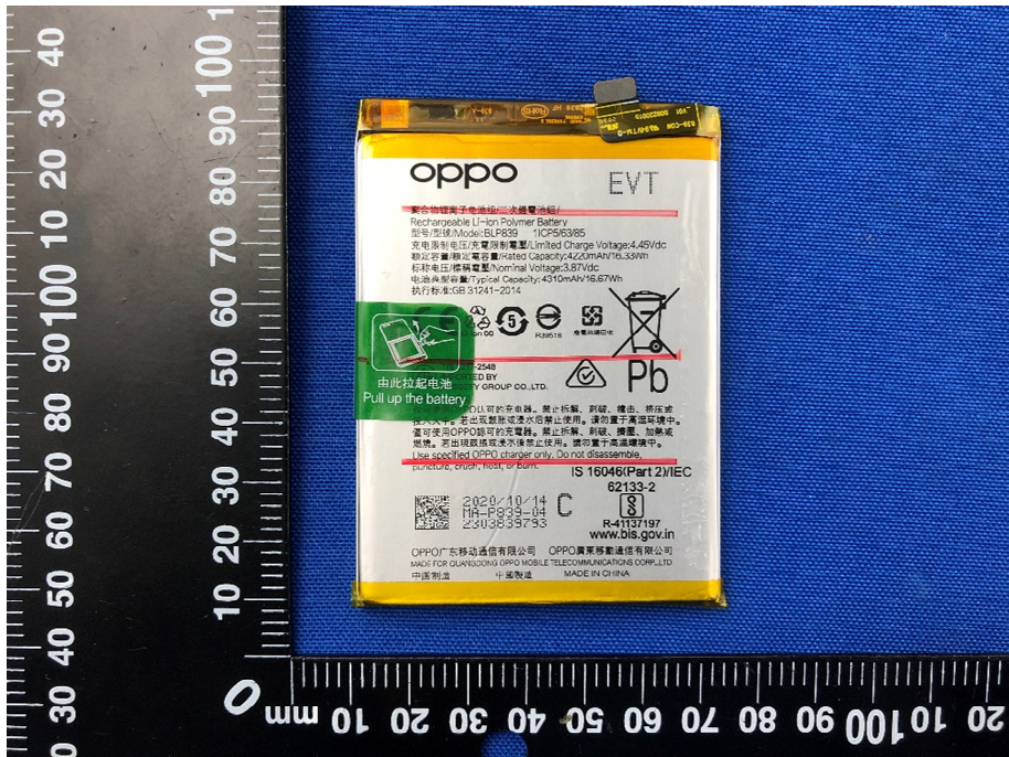
Battery Photo (BLP839 (Dongguan NVT Technology Co., Ltd.)) (FRONT)
