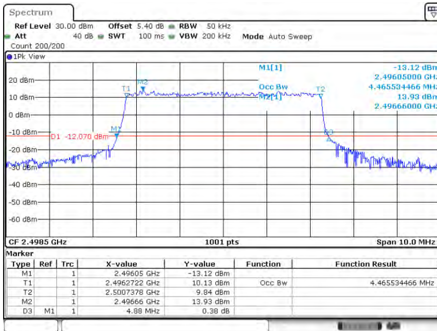
Band41-5MHz-QPSK-39675-25RB#0-4.466
