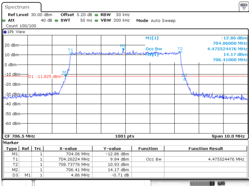
Band17-5MHz-QPSK-23755-25RB#0-4.476
