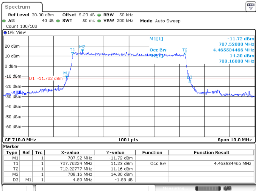
Band17-5MHz-QPSK-23790-25RB#0-4.466
