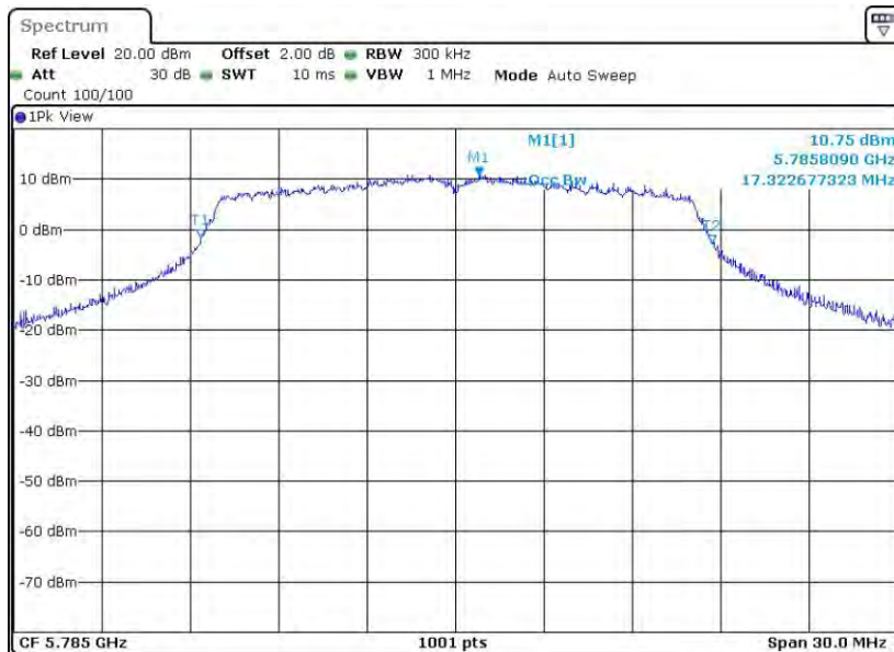
11A_Ant8_5785
