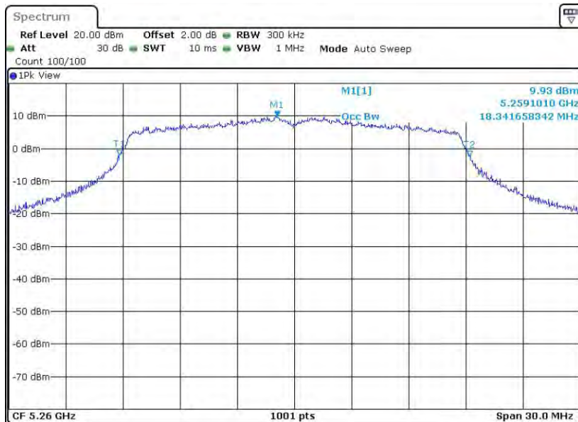
11N20SISO_Ant8_5260
