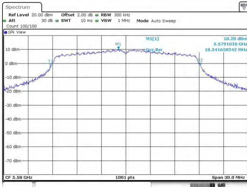
11N20SISO_Ant8_5580
