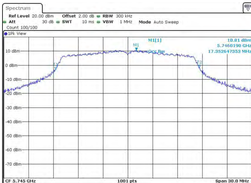
11A_Ant8_5745
