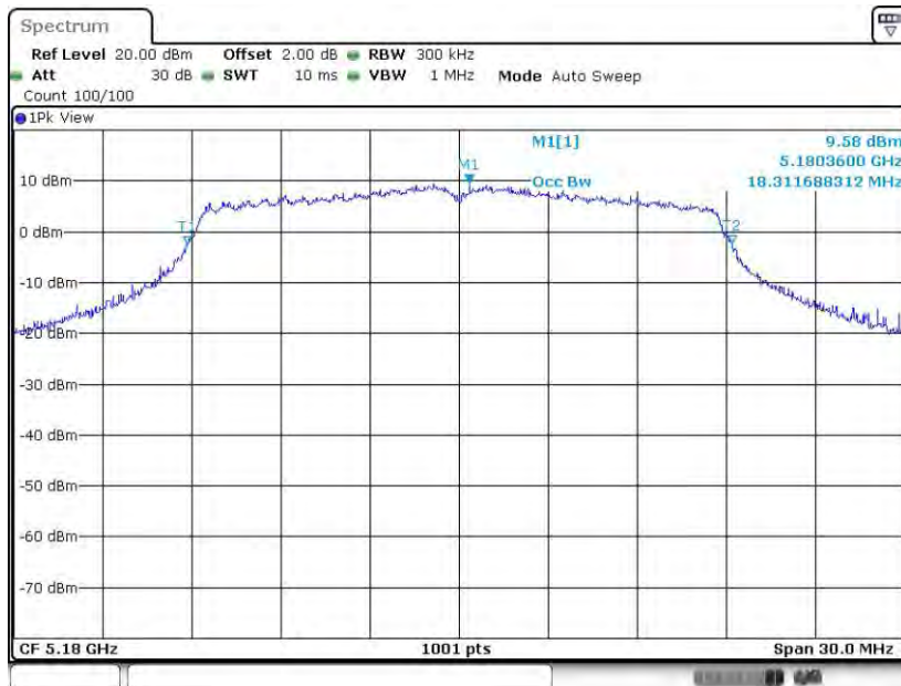
11N20SISO_Ant8_5180
