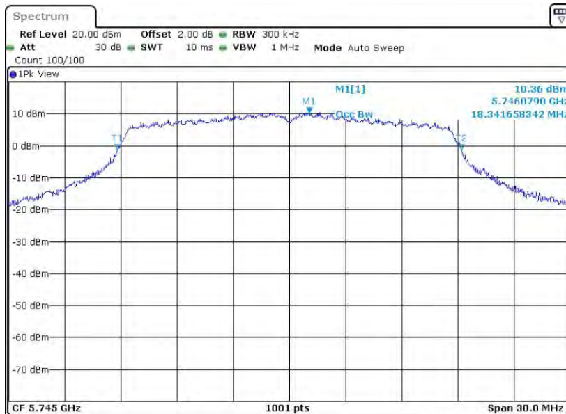
11N20SISO_Ant8_5745
