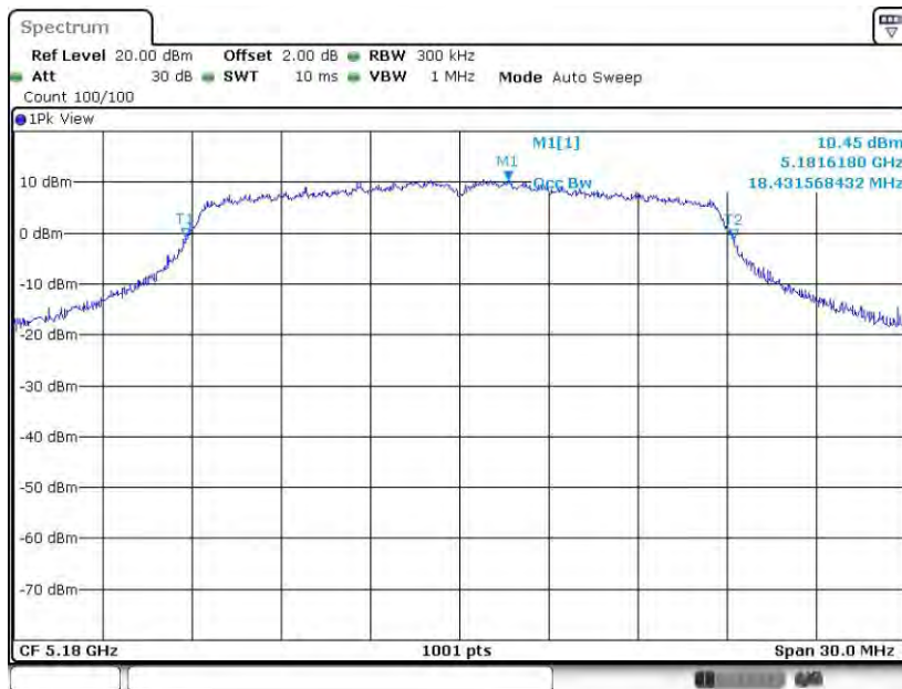
11N20SISO_Ant2_5180
