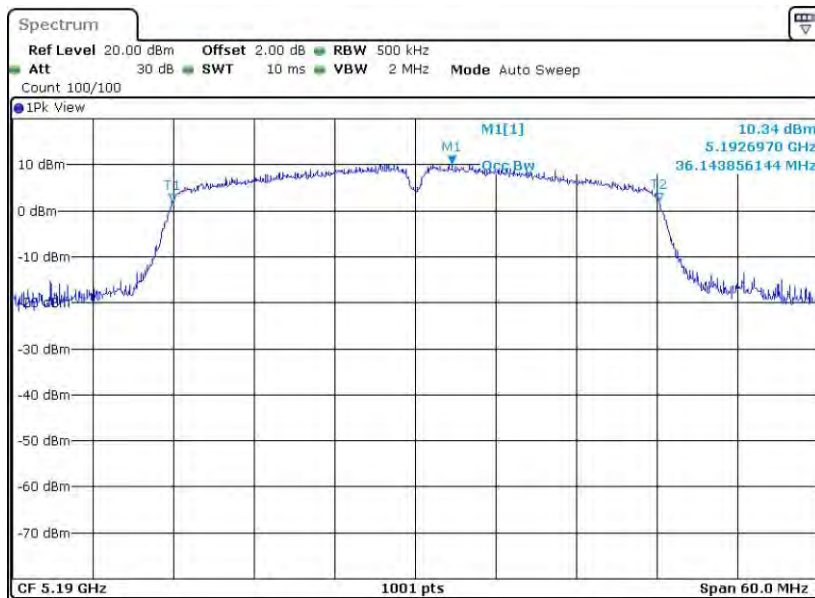
11AC40SISO_Ant2_5190
