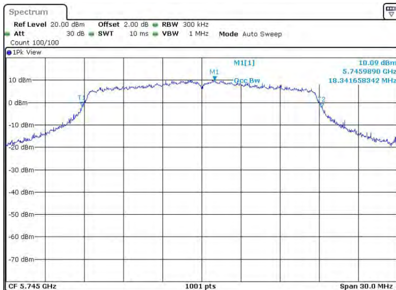
11AC20SISO_Ant2_5745
