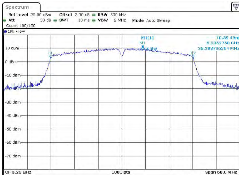
11AC40SISO_Ant2_5230
