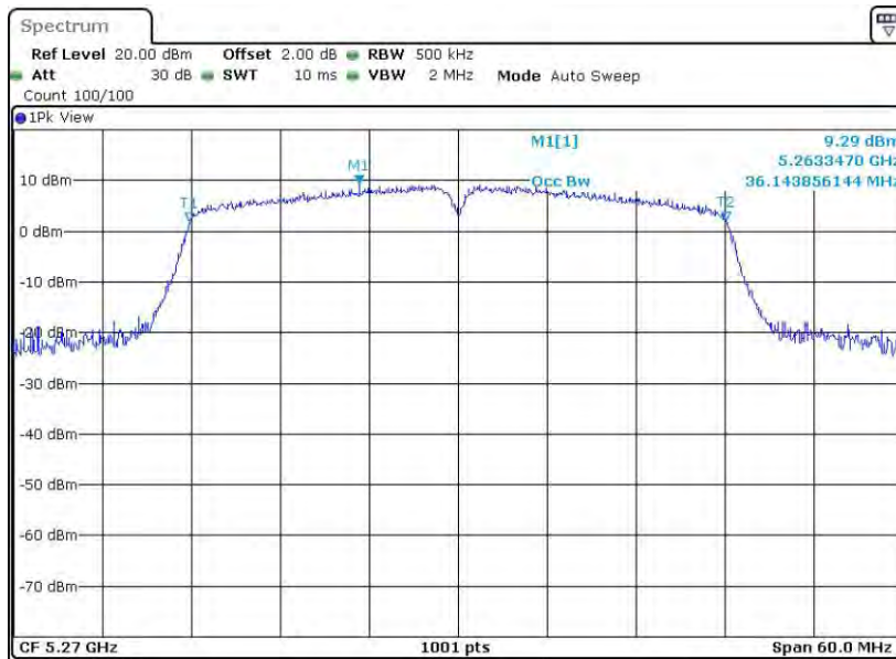
11AC40SISO_Ant8_5270
