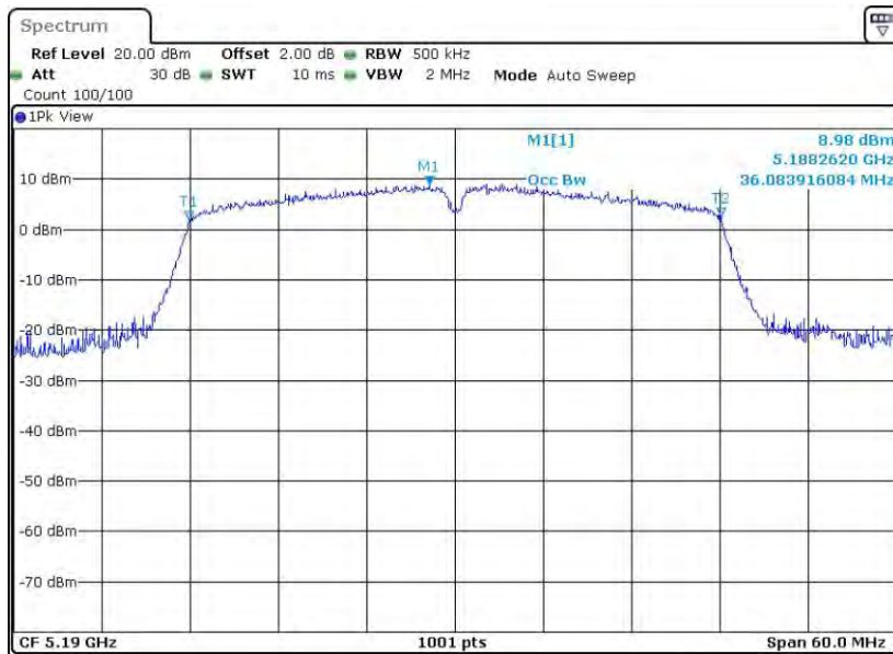
11AC40SISO_Ant8_5190
