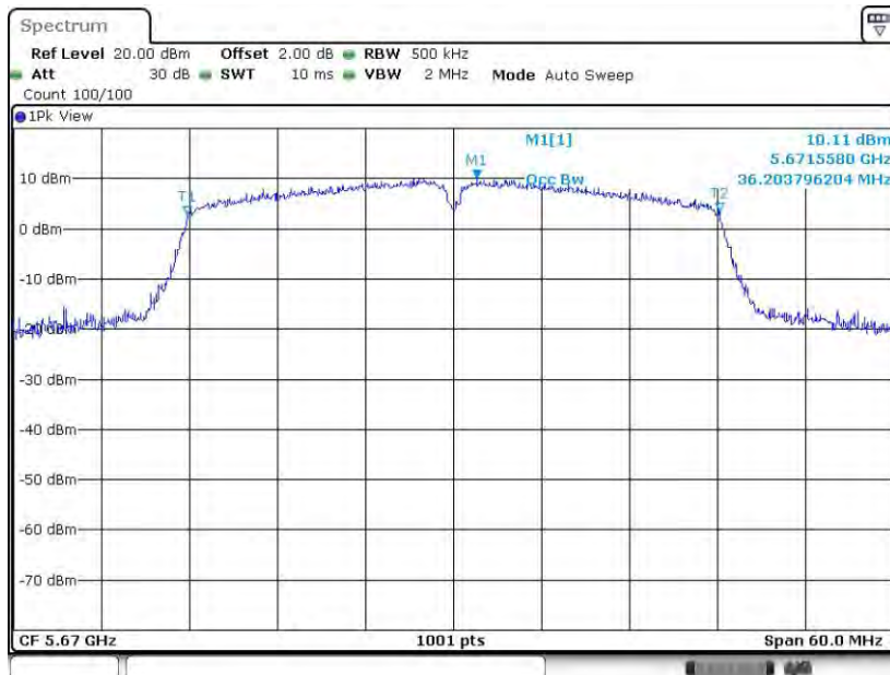
11AC40SISO_Ant8_5670
