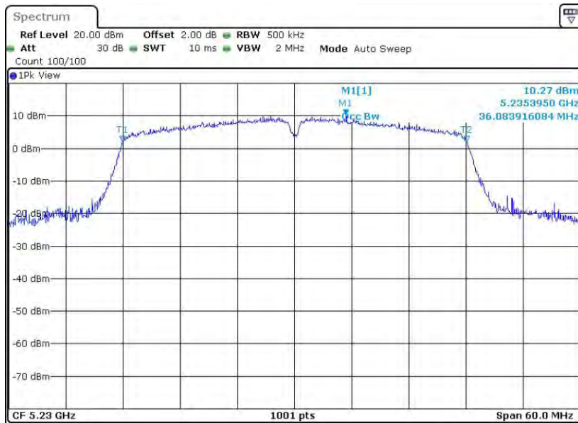
11AC40SISO_Ant8_5230
