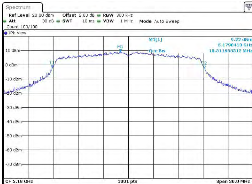
11AC20SISO_Ant8_5180
