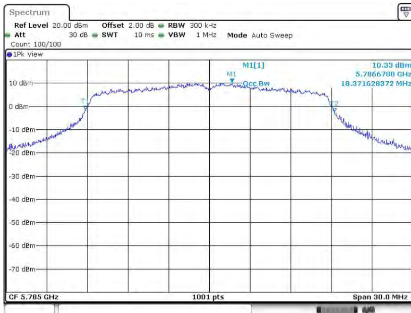
11AC20SISO_Ant2_5785
