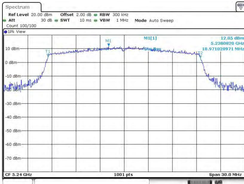
11AX20SISO_Ant8_5240
