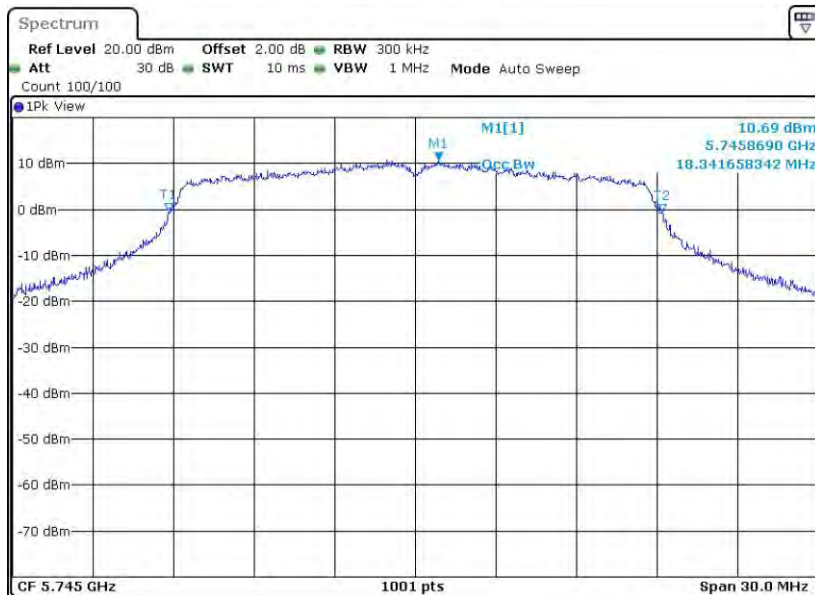
11AC20SISO_Ant8_5745
