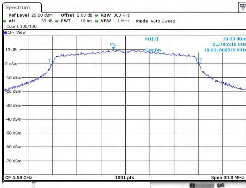
11AC20SISO_Ant2_5580
