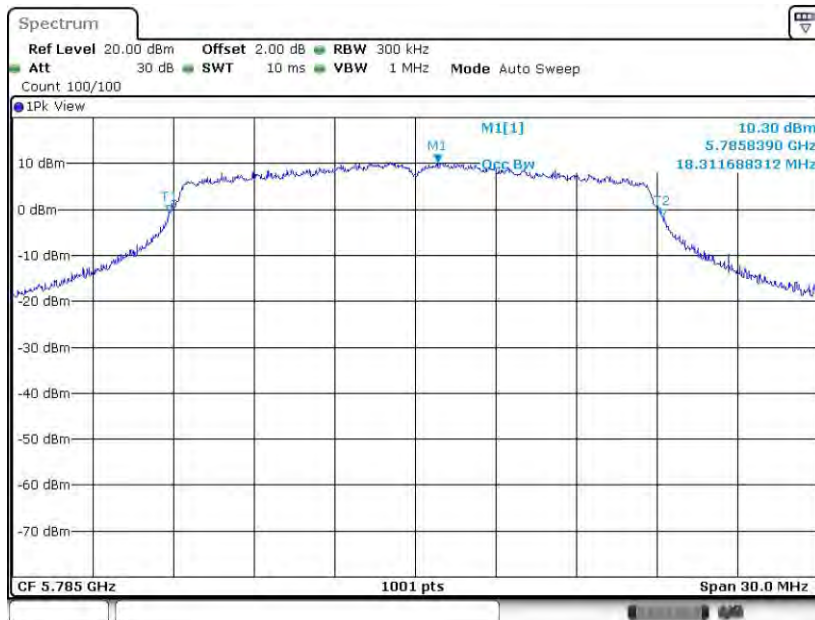
11AC20SISO_Ant8_5785
