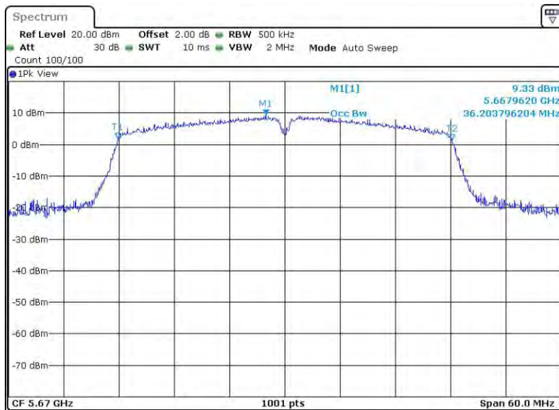
11AC40SISO_Ant2_5670
