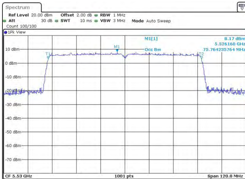
11AC80SISO_Ant2_5530
