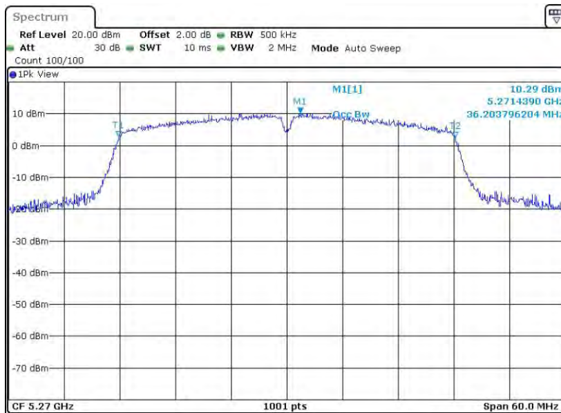
11AC40SISO_Ant2_5270
