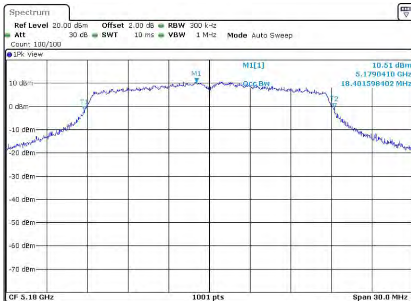
11AC20SISO_Ant2_5180
