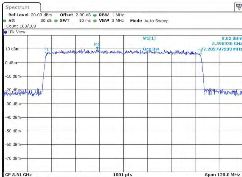
11AX80SISO_Ant2_5610
