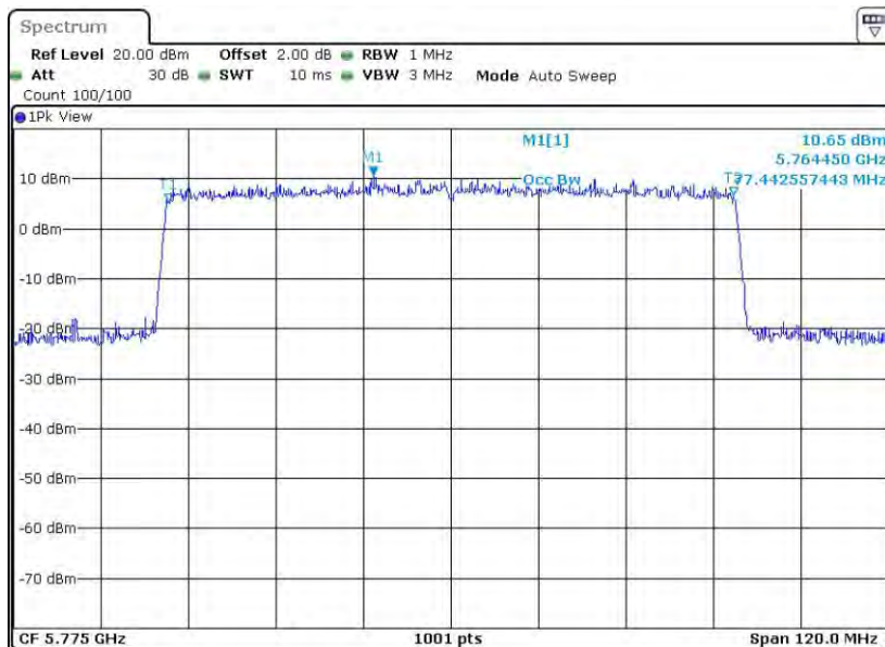
11AX80SISO_Ant2_5775
