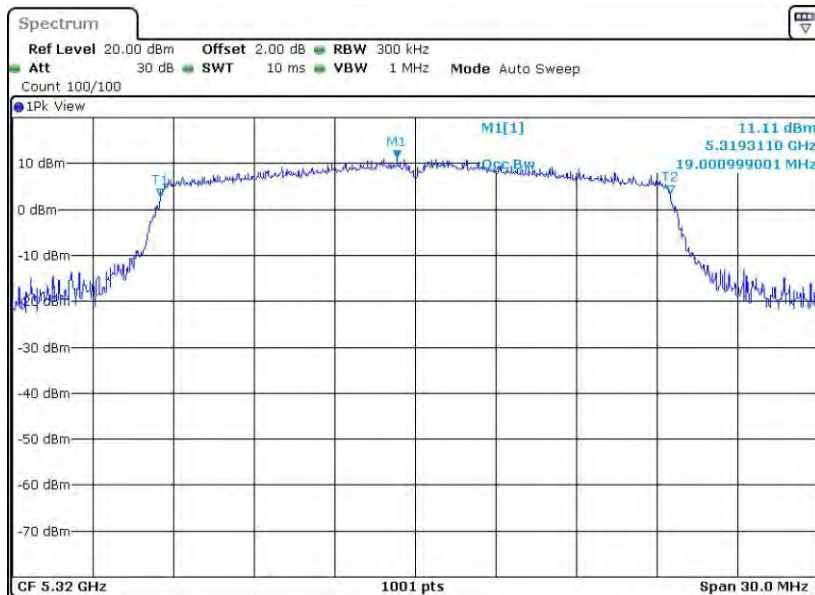
11AX20SISO_Ant8_5320
