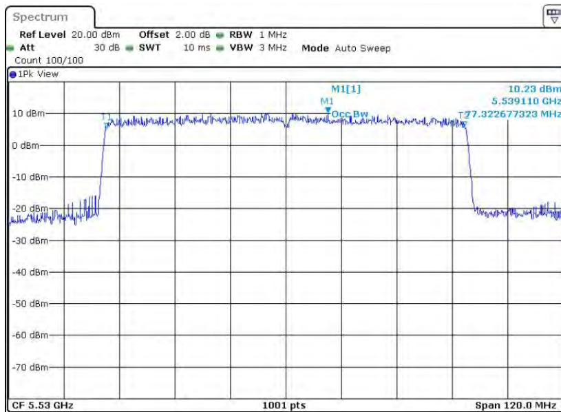
11AX80SISO_Ant2_5530
