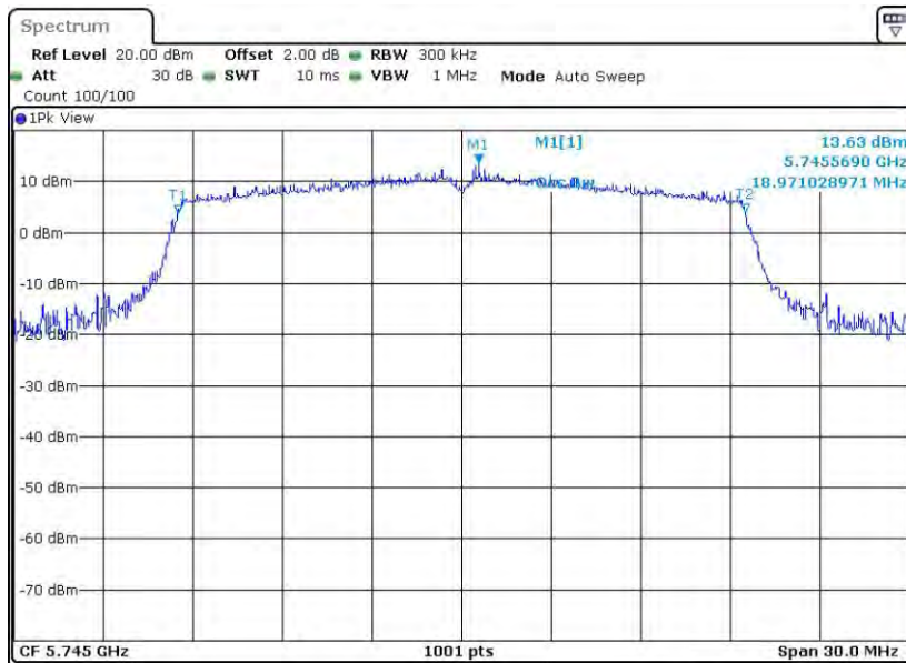
11AX20SISO_Ant8_5745
