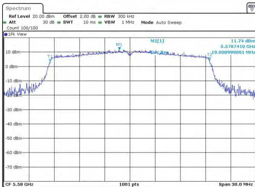
11AX20SISO_Ant8_5580
