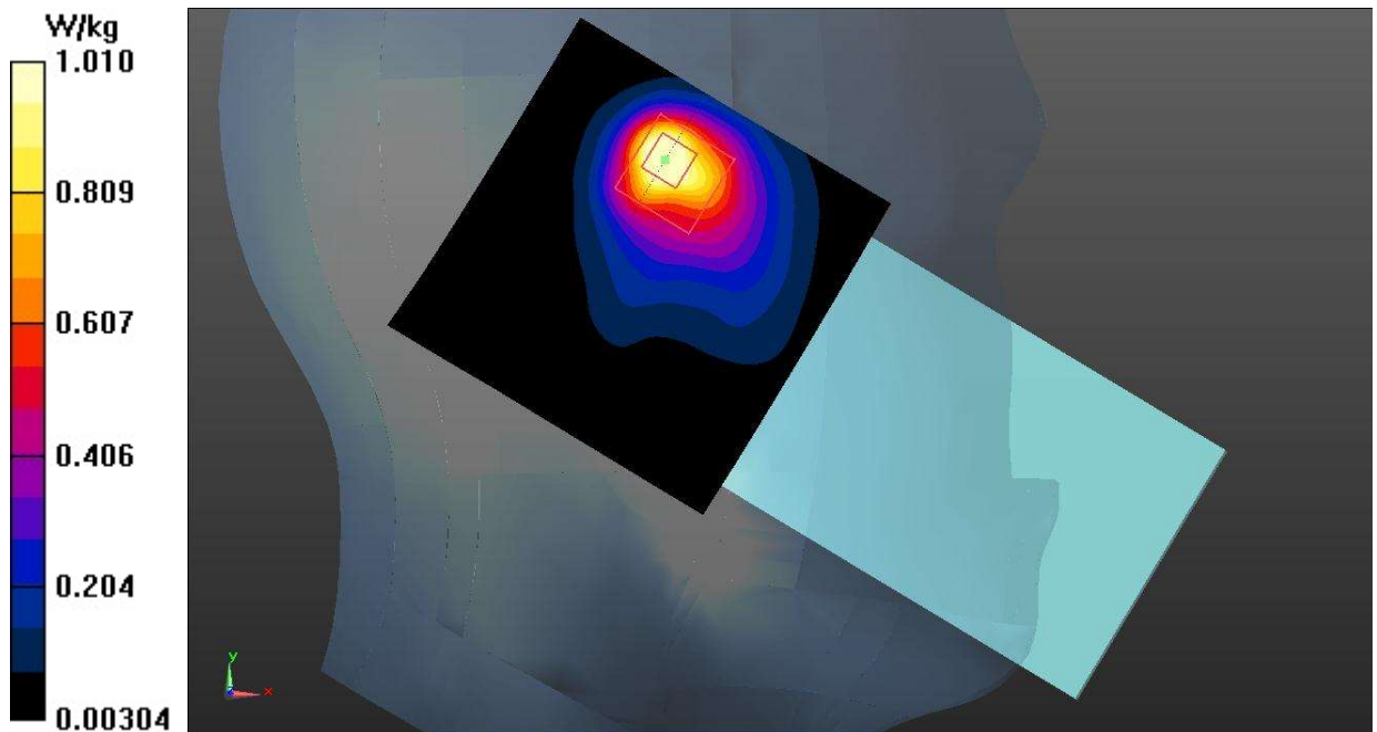
Fig.28 WLAN 2.4G
