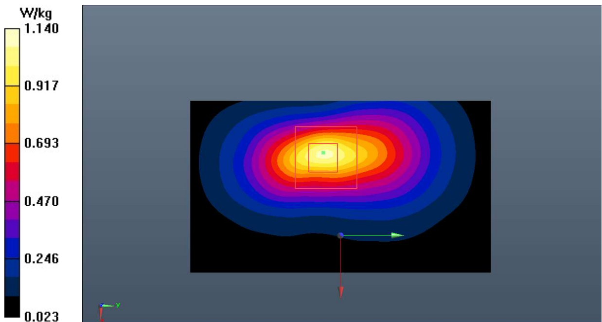
Fig.26 LTE Band 66
