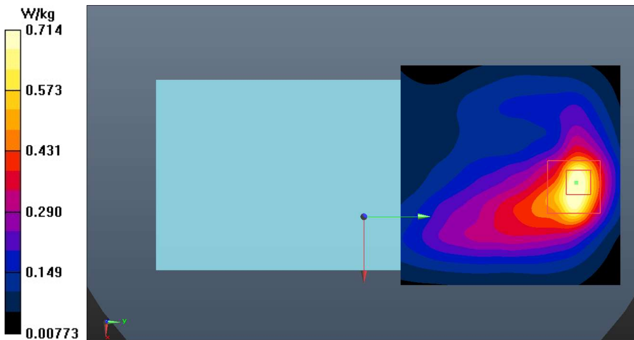
Fig.24 LTE Band 41
