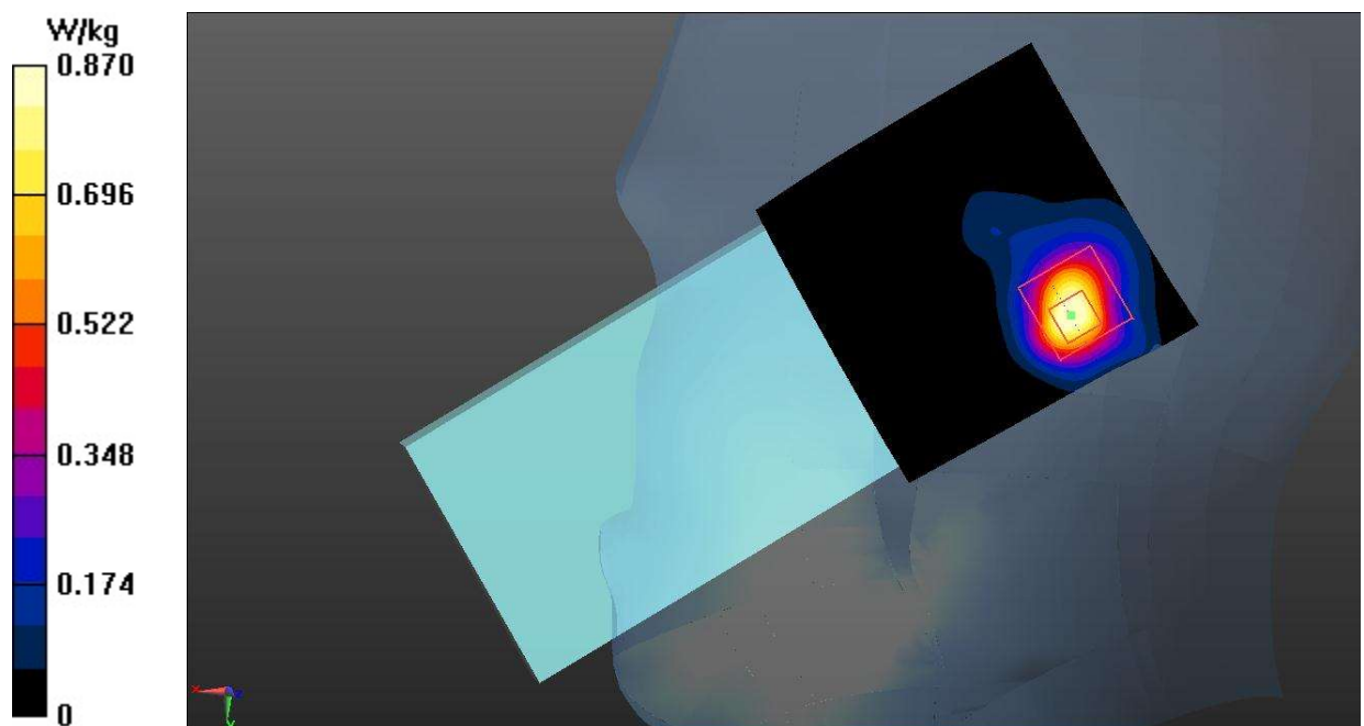
Fig.30 WLAN 5G
