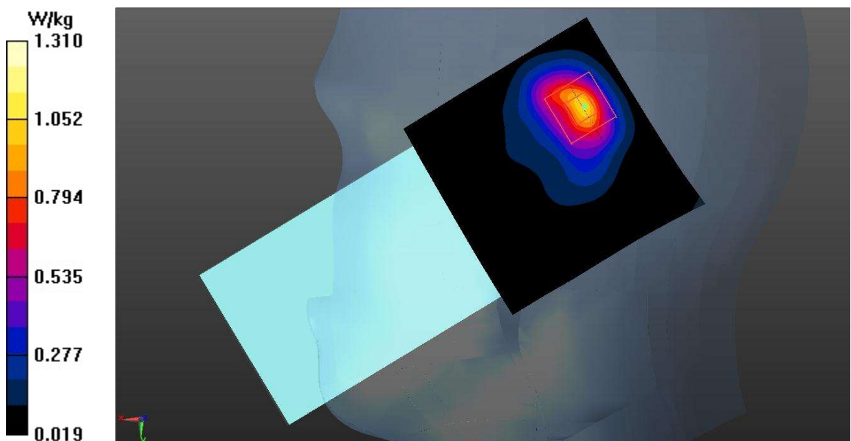
Fig.27 LTE Band 66
