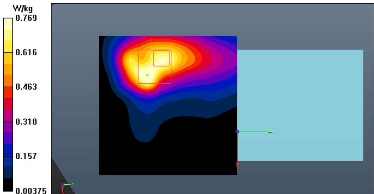
Fig.26 LTE Band 41
