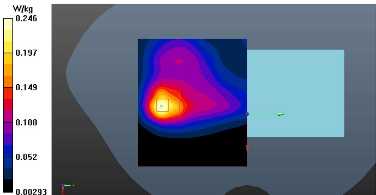
Fig.31 WLAN 2.4G
