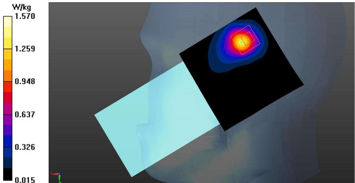
Fig.23 LTE Band 38
