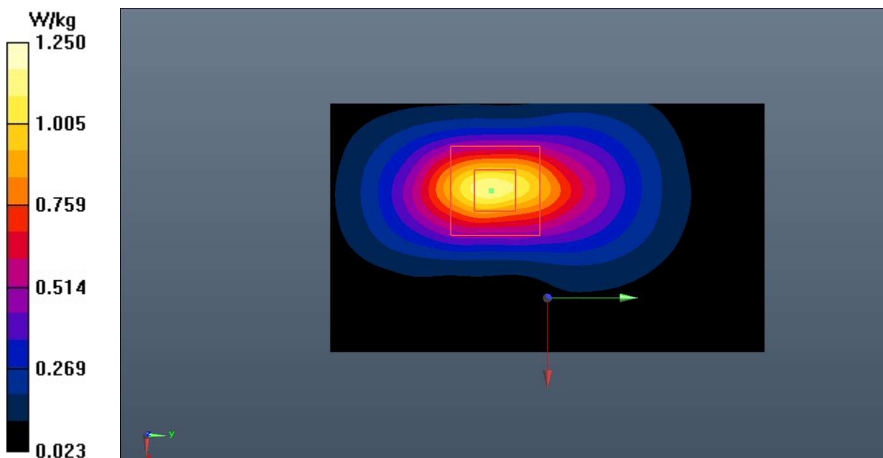
Fig.28 LTE Band 66
