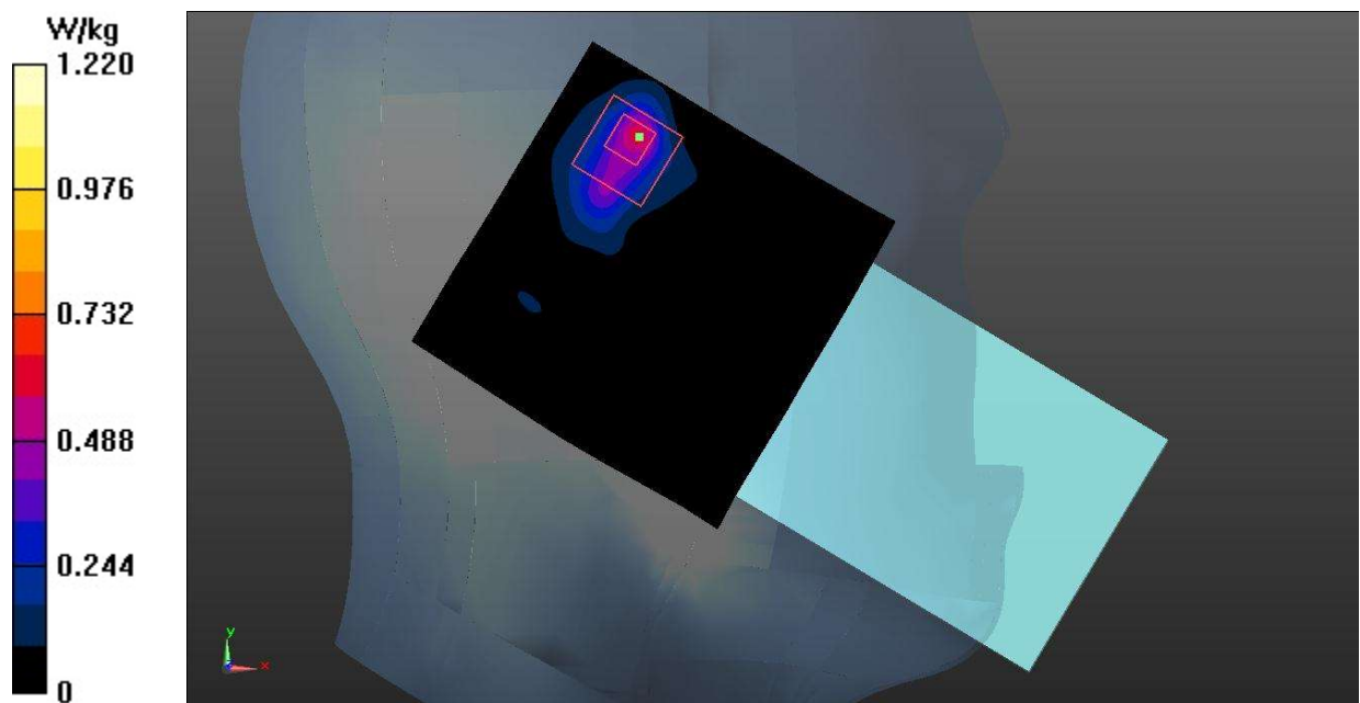
Fig.32 WLAN 5G
