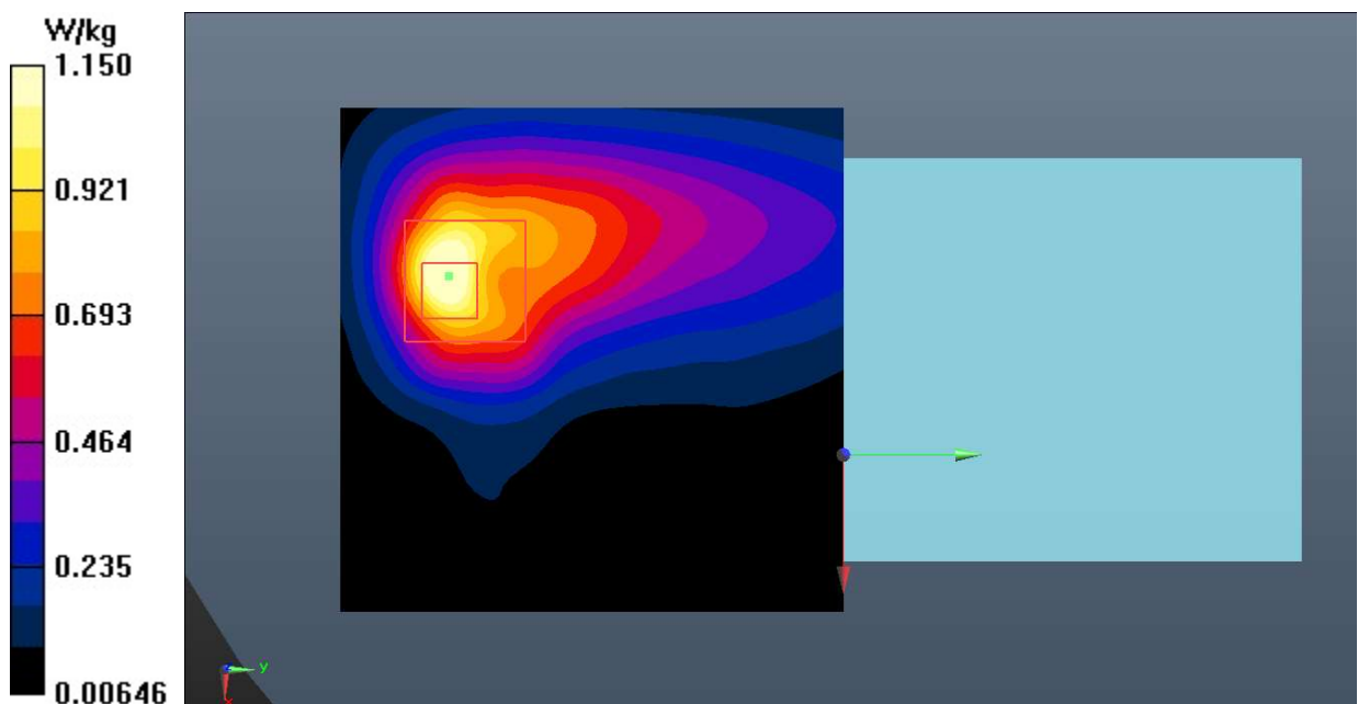
Fig.24 LTE Band 38
