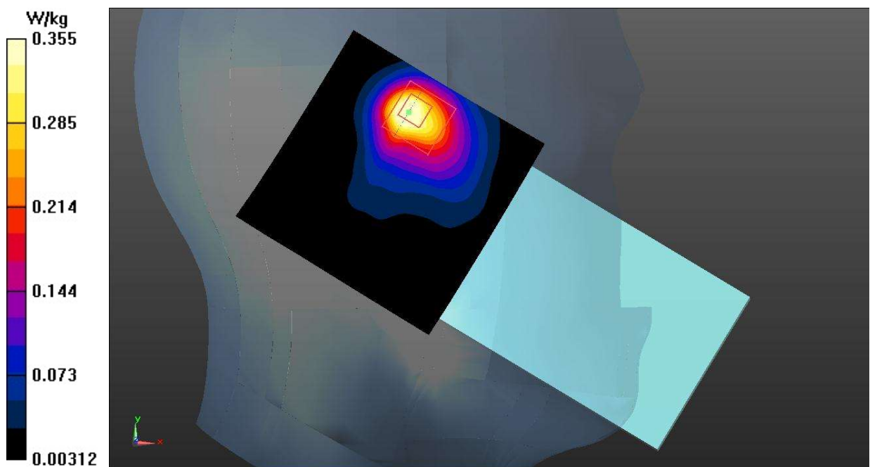
Fig.29 Bluetooth
