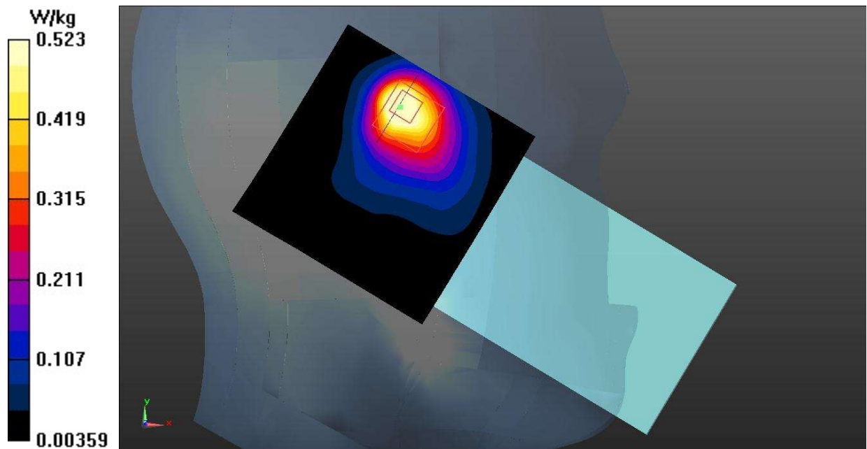
Fig.30 WLAN 2.4G
