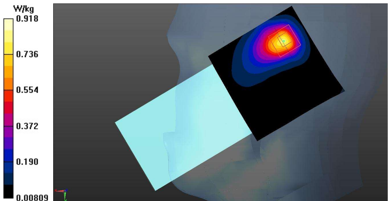
Fig.25 LTE Band 41
