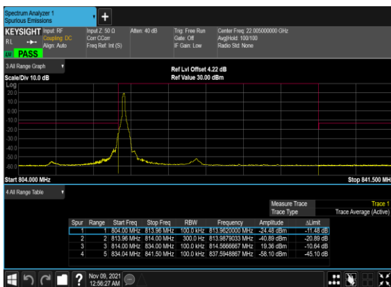
N26(20M)_DFT-s-OFDM_QPSK_Edge_1RB_Left _Low_CH
