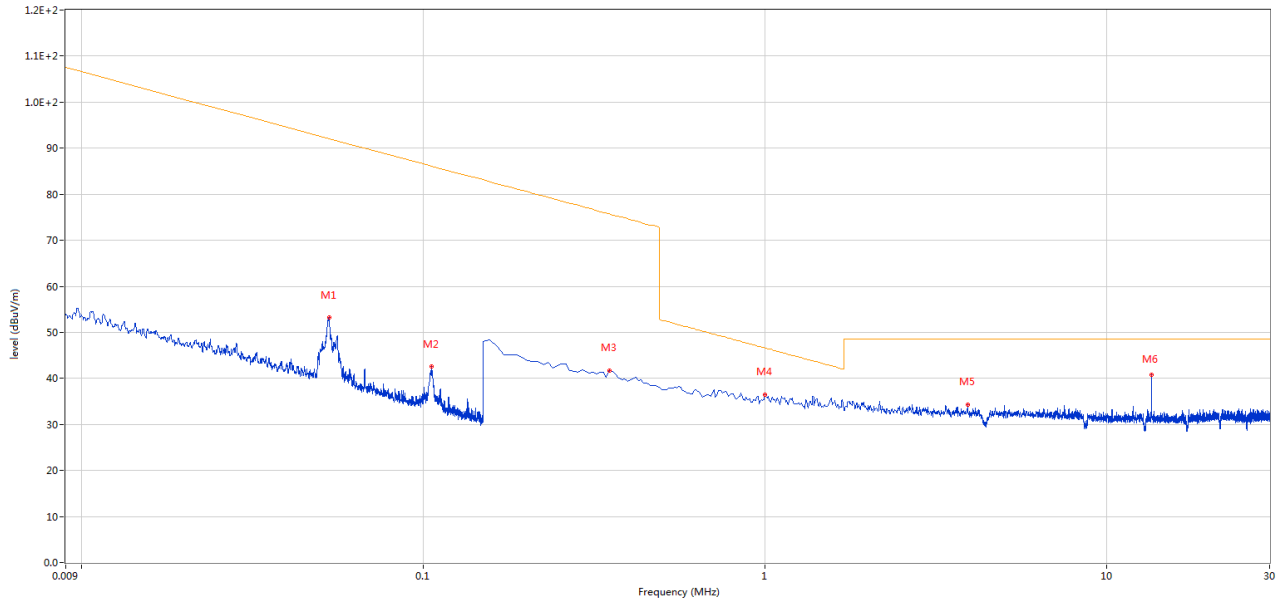
Below 30 MHz ANT Vertical
