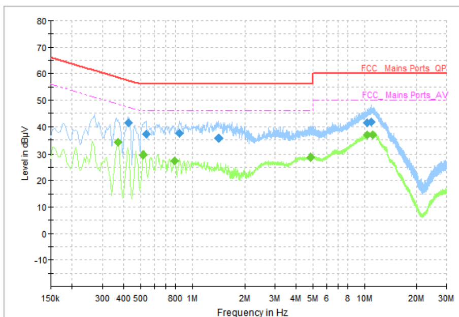
Fig.58 AC Power line Conducted Emission (Idle), LE 1M
