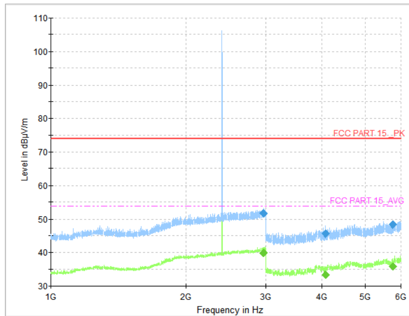
Fig. 40 Radiated Spurious Emission (GFSK, CH0, 1 GHz ~6 GHz)
