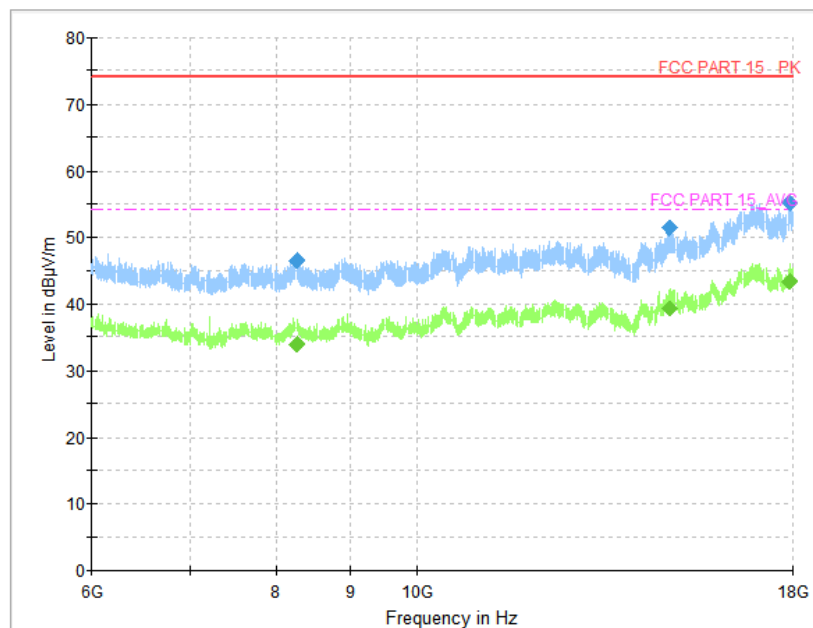
Fig. 57 Radiated Spurious Emission (8DPSK, CH0, 6 GHz ~18 GHz)
