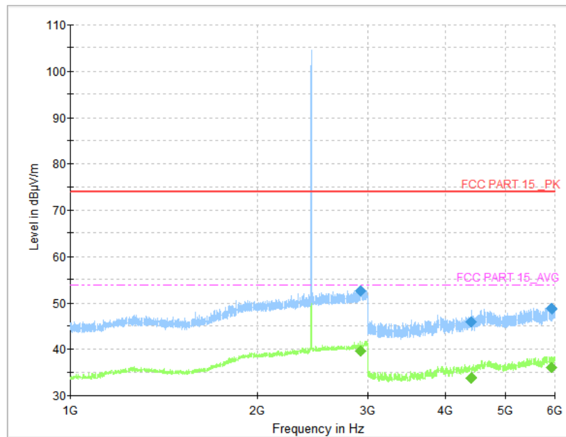
Fig. 58 Radiated Spurious Emission (8DPSK, CH39, 1 GHz ~6 GHz)
