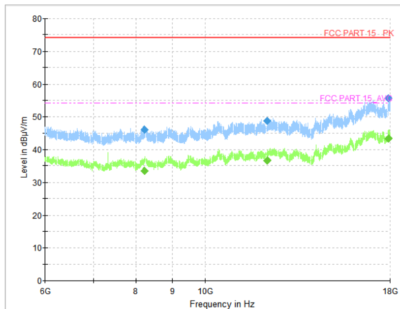
Fig. 59 Radiated Spurious Emission (8DPSK, CH39, 6 GHz ~18 GHz)
