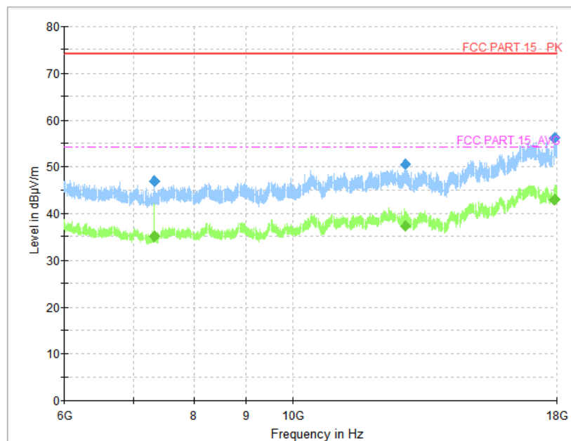
Fig. 43 Radiated Spurious Emission (GFSK, CH39, 6 GHz ~18 GHz)
