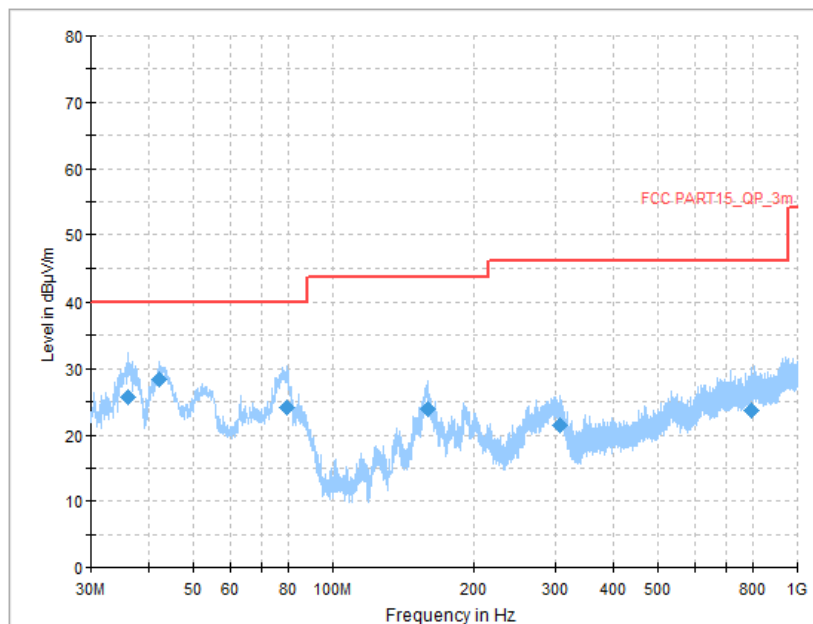
Fig. 65 Radiated Spurious Emission (All Channels, 30 MHz ~1 GHz)
