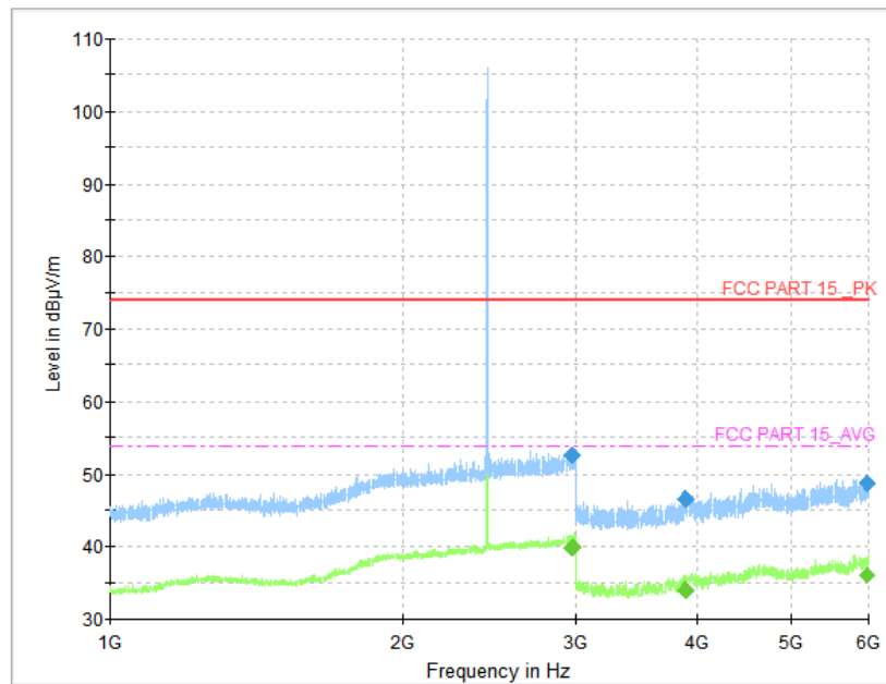
Fig. 42 Radiated Spurious Emission (GFSK, CH39, 1 GHz ~6 GHz)
