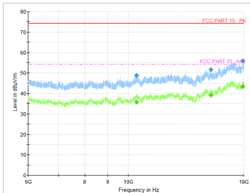
Fig. 45 Radiated Spurious Emission (GFSK, CH78, 6 GHz ~18 GHz)
