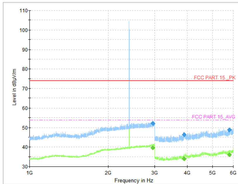
Fig. 56 Radiated Spurious Emission (8DPSK, CH0, 1 GHz ~6 GHz)
