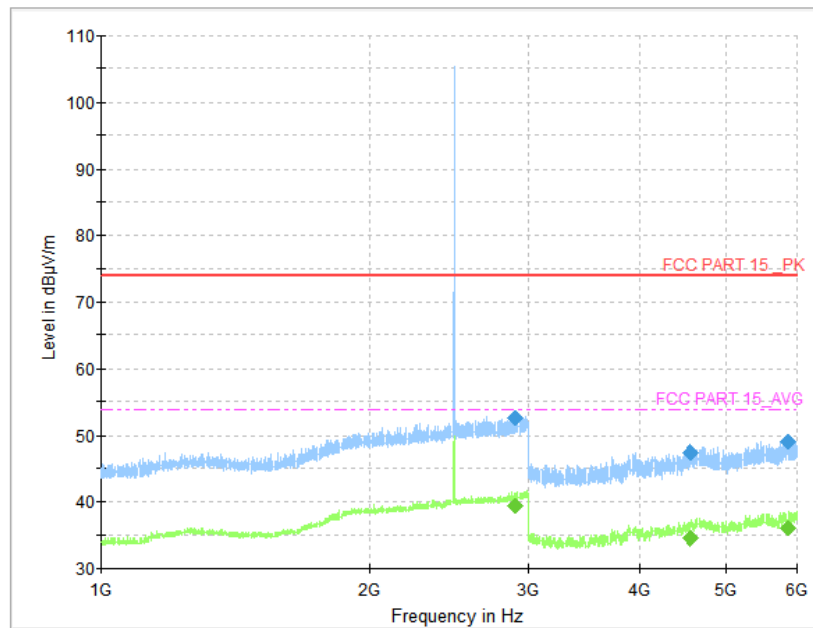
Fig. 44 Radiated Spurious Emission (GFSK, CH78, 1 GHz ~6 GHz)
