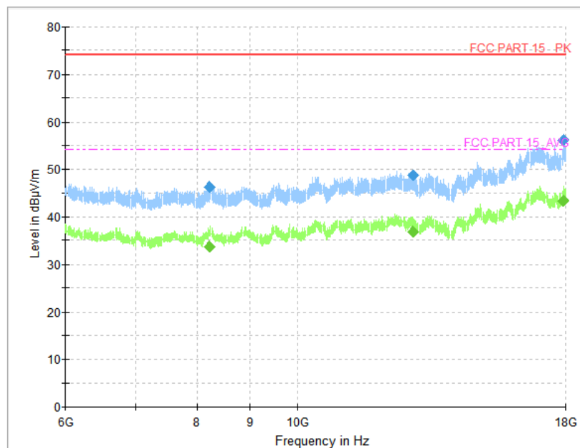
Fig. 61 Radiated Spurious Emission (8DPSK, CH78, 6 GHz ~18 GHz)
