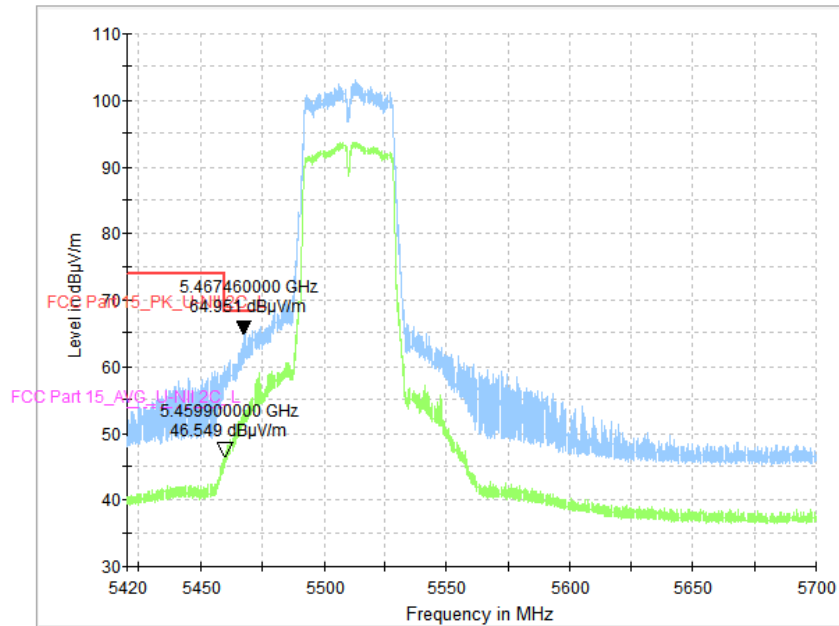
Fig. 71 Band Edges (802.11ac-VHT40, CH102 5510MHz)
