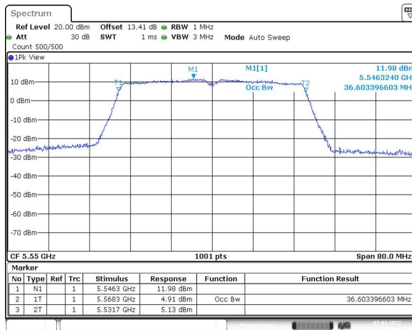
Fig. 50 99% Occupied Bandwidth (802.11ac-VHT40, 5550MHz)
