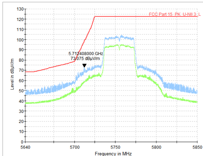
Fig. 73 Band Edges (802.11ac-VHT40, CH151 5755MHz)
