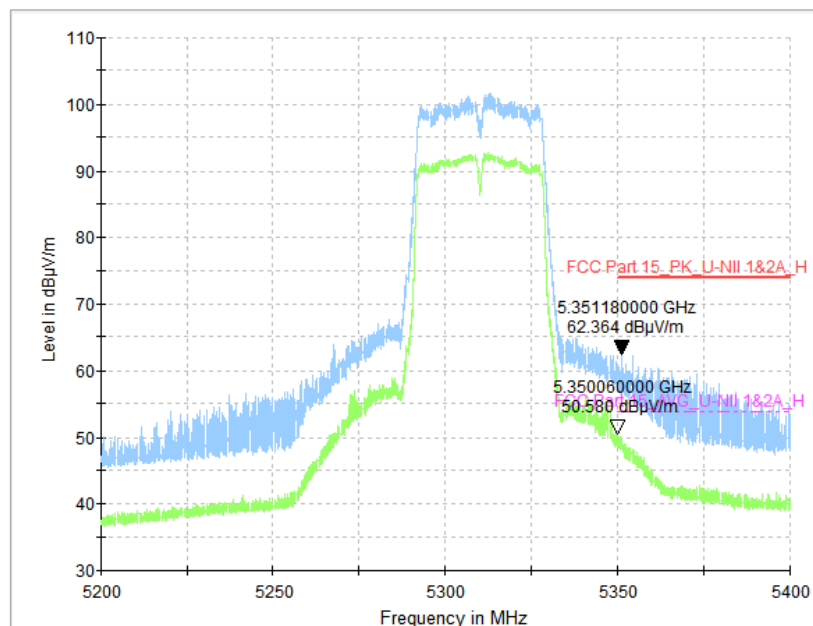
Fig. 70 Band Edges (802.11ac-VHT40, CH62 5310MHz)
