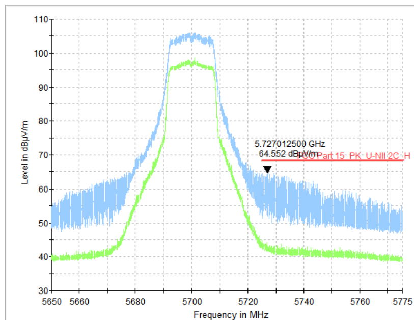
Fig. 66 Band Edges (802.11a, CH140 5700MHz)
