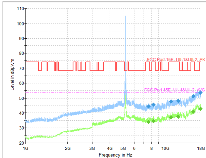
Fig. 92 Transmitter Spurious Emission (802.11ac-VHT40, CH38 5190MHz, 1 GHz-18 GHz)
