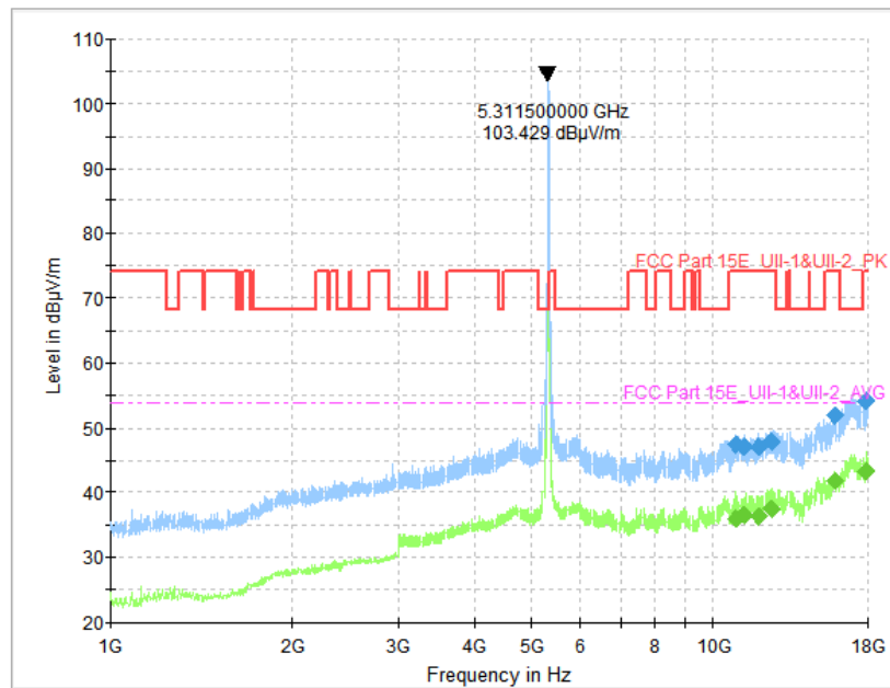
Fig. 95 Transmitter Spurious Emission (802.11ac-VHT40, CH62 5310MHz, 1 GHz-18 GHz)
