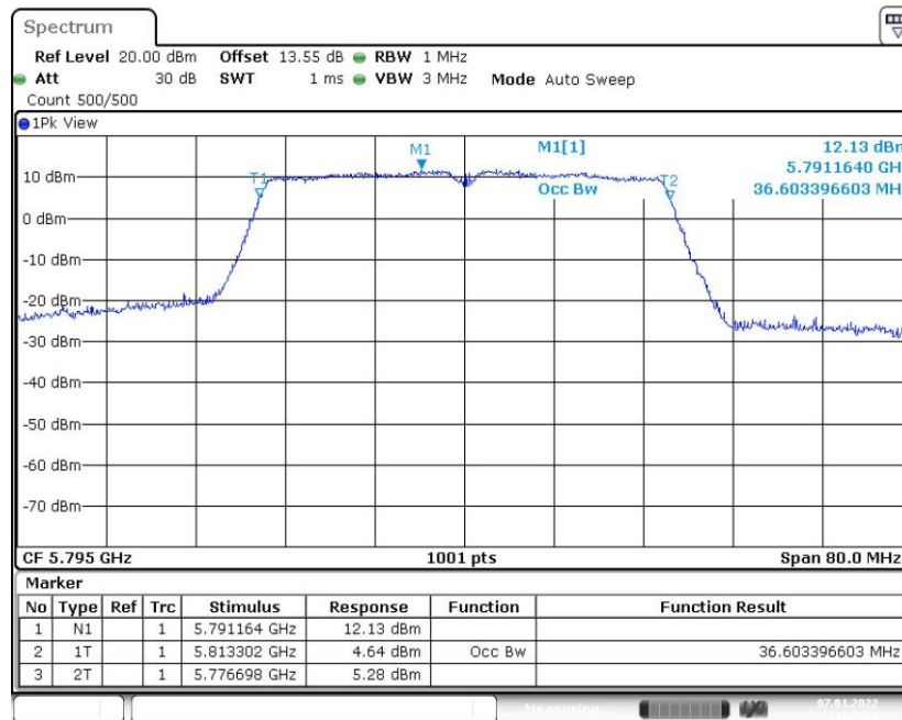
Fig. 53 99% Occupied Bandwidth (802.11ac-VHT40, 5795MHz)
