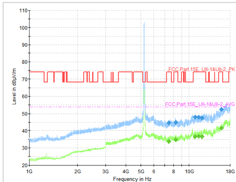
Fig. 93 Transmitter Spurious Emission (802.11ac-VHT40, CH46 5230MHz, 1 GHz-18 GHz)
