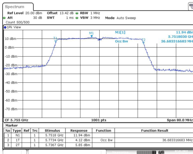
Fig. 52 99% Occupied Bandwidth (802.11ac-VHT40, 5755MHz)
