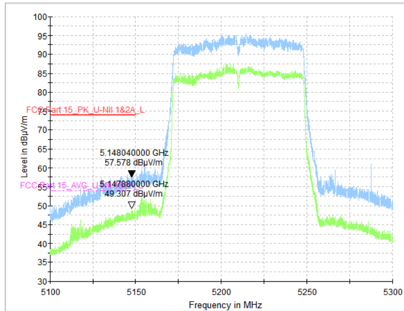
Fig. 75 Band Edges (802.11ac-VHT80, CH42 5210MHz)
