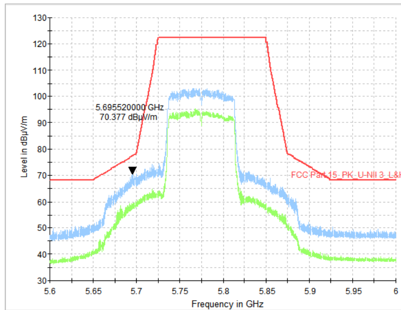
Fig. 79 Band Edges (802.11ac-VHT80, CH155 5775MHz)
