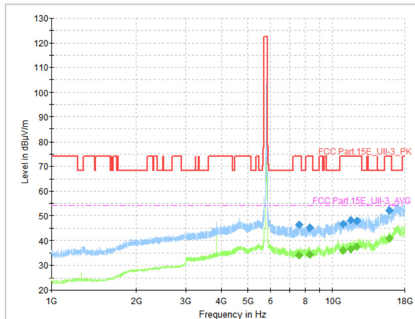
Fig. 100 Transmitter Spurious Emission (802.11ac-VHT40, CH159 5795MHz, 1 GHz-18 GHz)
