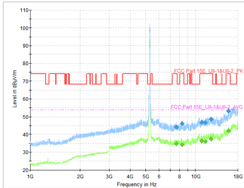
Fig. 94 Transmitter Spurious Emission (802.11ac-VHT40, CH54 5270MHz, 1 GHz-18 GHz)
