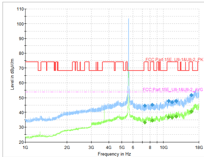
Fig. 97 Transmitter Spurious Emission (802.11ac-VHT40, CH118 5580MHz, 1 GHz-18 GHz)
