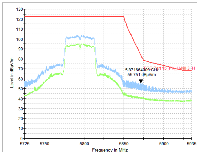
Fig. 74 Band Edges (802.11ac-VHT40, CH159 5795MHz)
