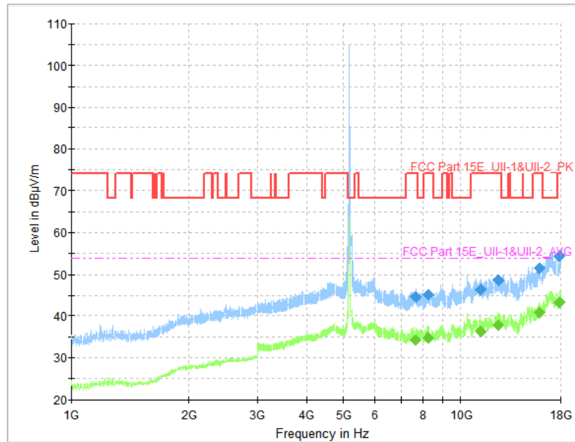
Fig. 80 Transmitter Spurious Emission (802.11a, CH36 5180MHz, 1 GHz-18 GHz)
