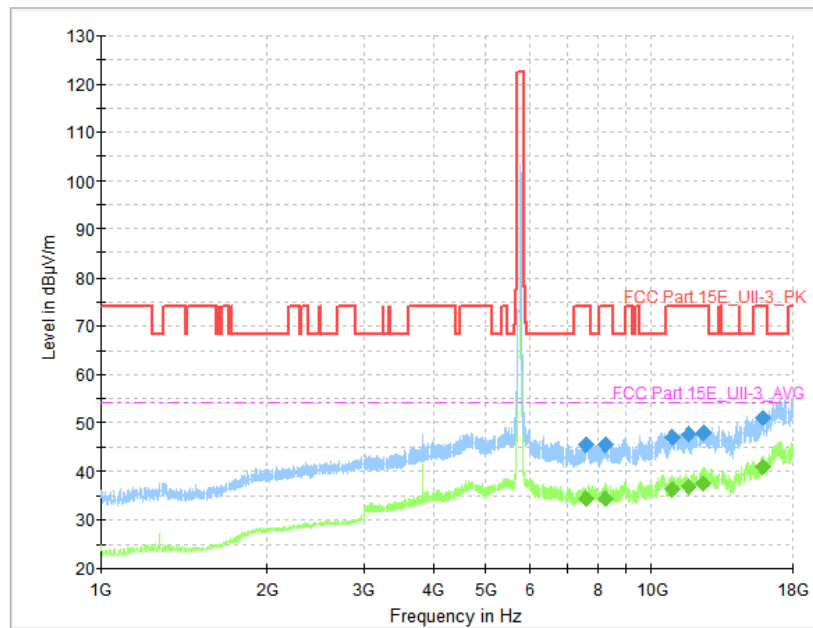
Fig. 99 Transmitter Spurious Emission (802.11ac-VHT40, CH151 5755MHz, 1 GHz-18 GHz)
