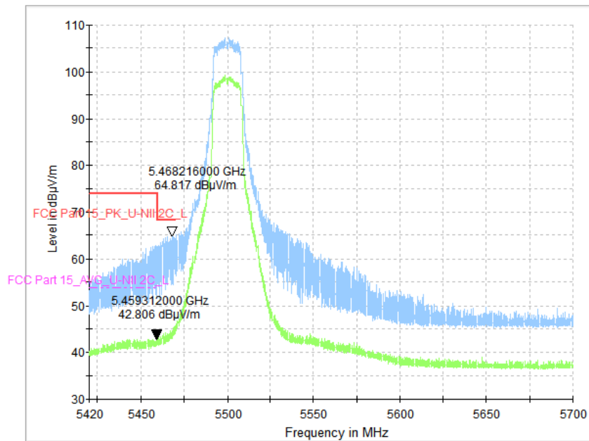
Fig. 65 Band Edges (802.11a, CH100 5500MHz)
