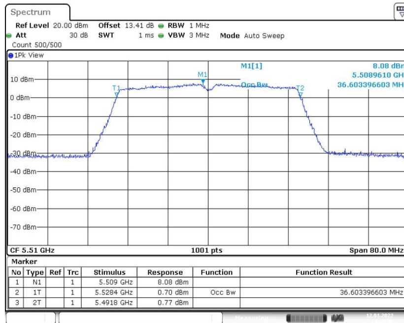
Fig. 49 99% Occupied Bandwidth (802.11ac-VHT40, 5510MHz)
