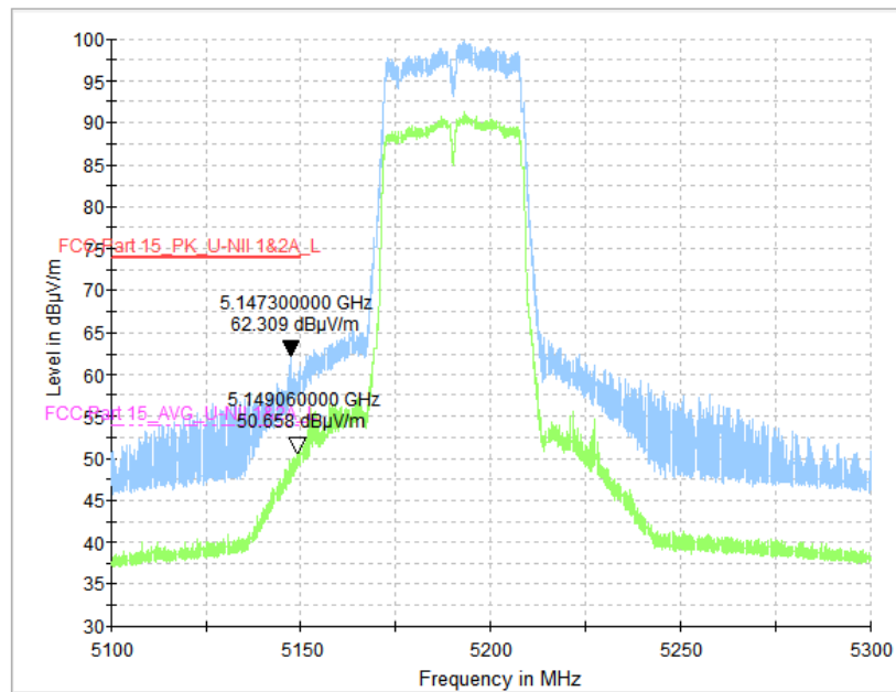
Fig. 69 Band Edges (802.11ac-VHT40, CH38 5190MHz)
