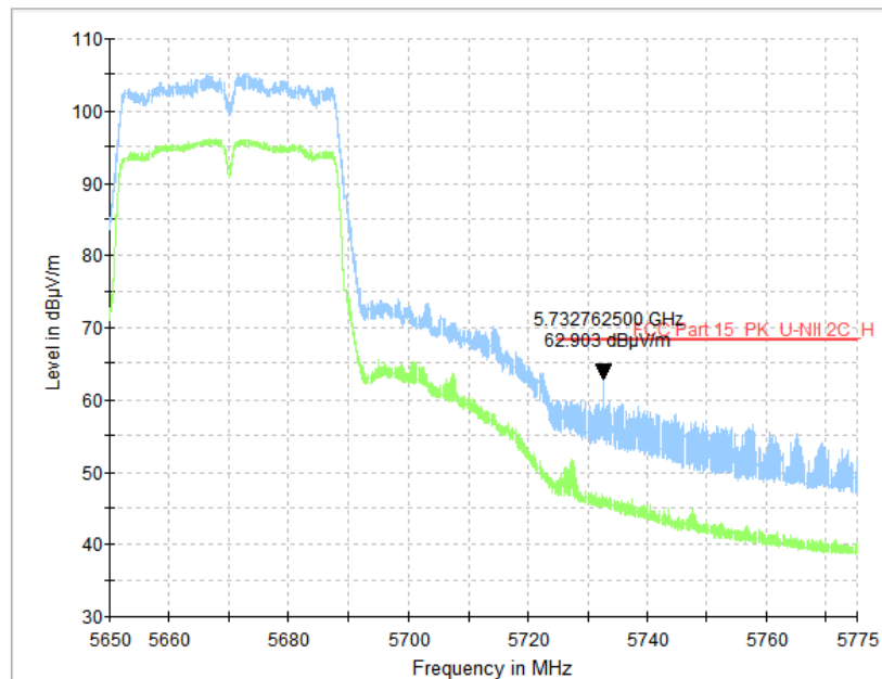
Fig. 72 Band Edges (802.11ac-VHT40, CH134 5670MHz)
