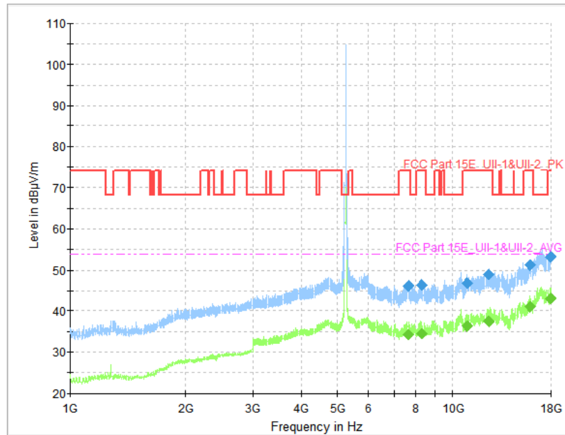
Fig. 82 Transmitter Spurious Emission (802.11a, CH48 5240MHz, 1 GHz-18 GHz)
