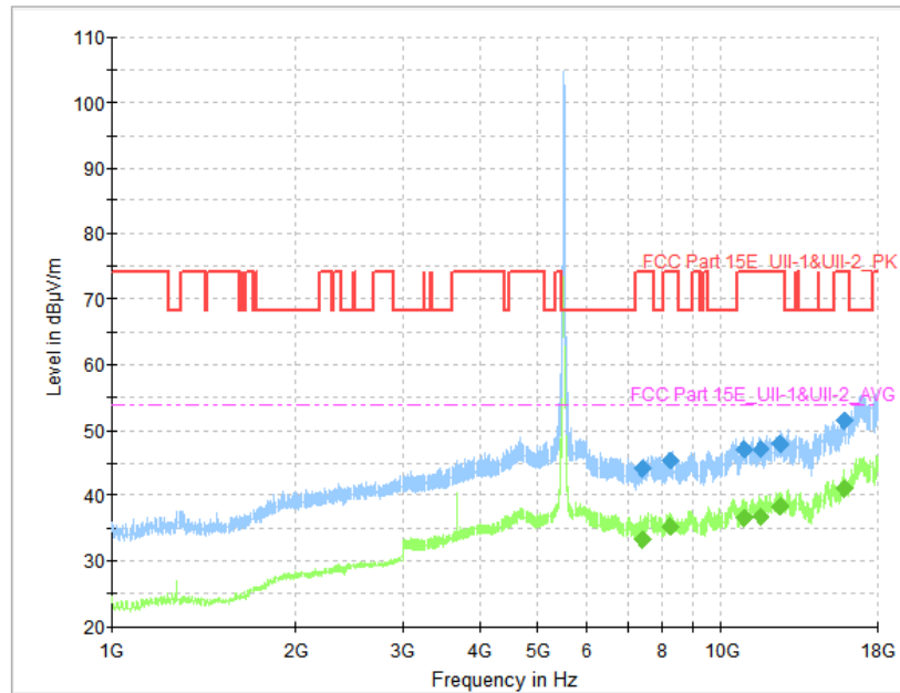
Fig. 96 Transmitter Spurious Emission (802.11ac-VHT40, CH102 5510MHz, 1 GHz-18 GHz)
