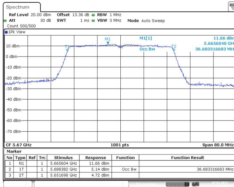
Fig. 51 99% Occupied Bandwidth (802.11ac-VHT40, 5670MHz)
