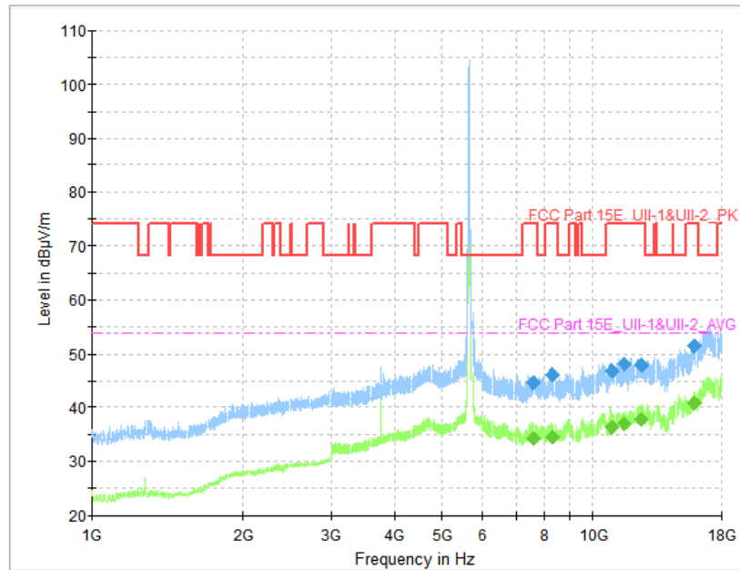
Fig. 98 Transmitter Spurious Emission (802.11ac-VHT40, CH134 5670MHz, 1 GHz-18 GHz)
