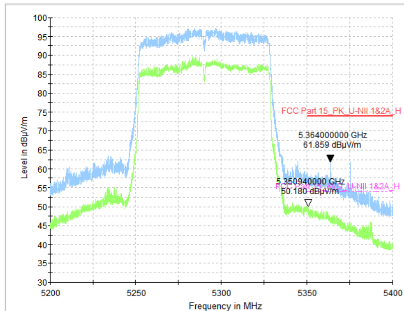
Fig. 76 Band Edges (802.11ac-VHT80, CH58 5290MHz)
