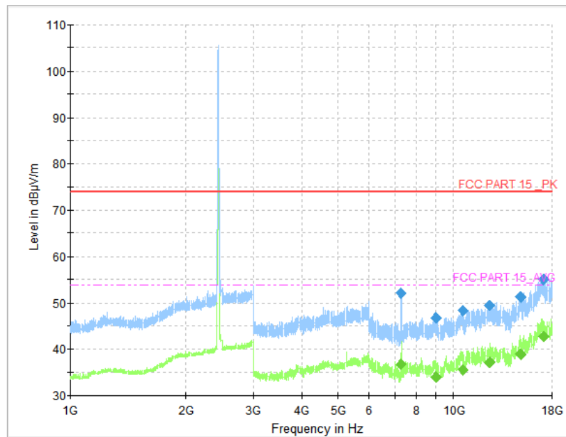
Fig.119 Radiated Spurious Emission (802.11-VHT20, CH6, 1 GHz-18 GHz)
