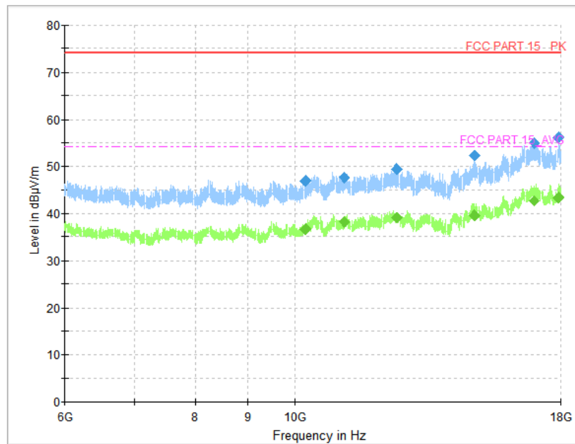
Fig.133 Radiated Spurious Emission (802.11-VHT40, CH9, 6 GHz-18 GHz)
