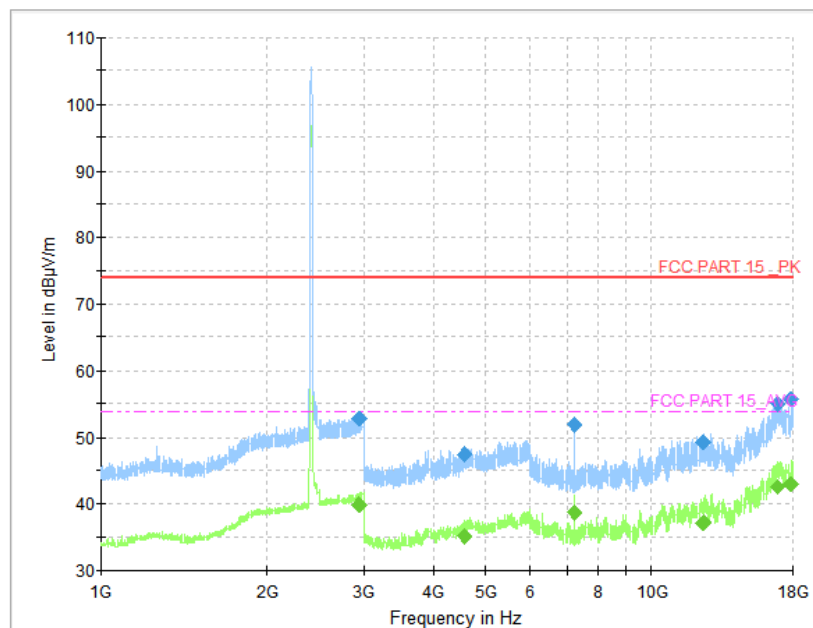
Fig.108 Radiated Spurious Emission (802.11g, CH1, 1 GHz-18 GHz)
