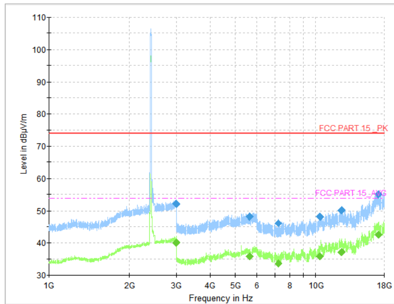
Fig.113 Radiated Spurious Emission (802.11n-HT20, CH1, 1 GHz-18 GHz)
