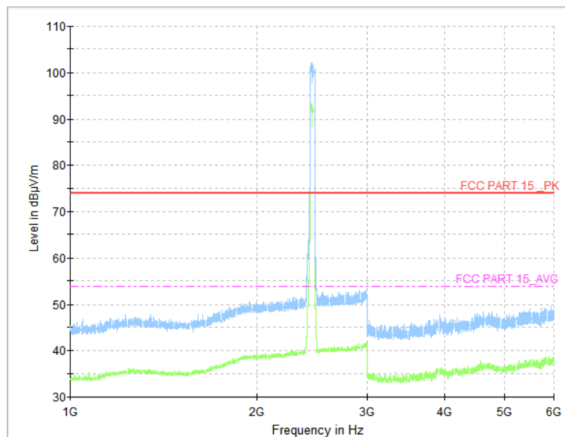
Fig.132 Radiated Spurious Emission (802.11-VHT40, CH9, 1 GHz-6 GHz)
