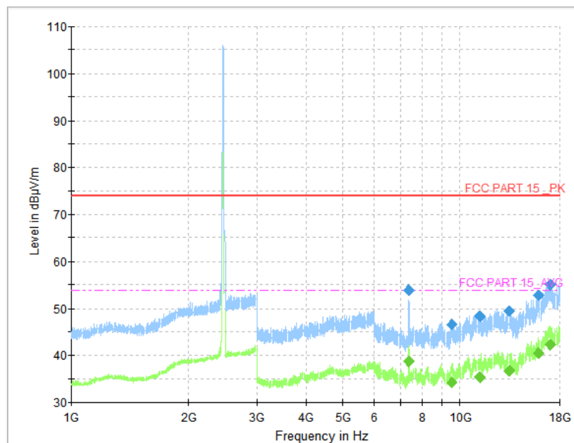
Fig.120 Radiated Spurious Emission (802.11-VHT20, CH11, 1 GHz-18 GHz)
