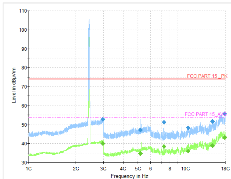
Fig.124 Radiated Spurious Emission (802.11n-HT40, CH6, 1 GHz-18 GHz)
