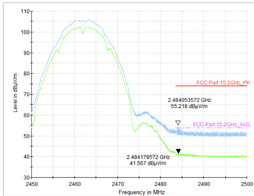
Fig.107 Radiated Restricted Band (802.11b, CH11, 2.45GHz~2.5GHz)
