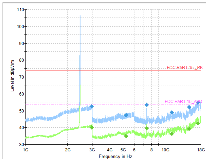
Fig.110 Radiated Spurious Emission (802.11g, CH11, 1 GHz-18 GHz)
