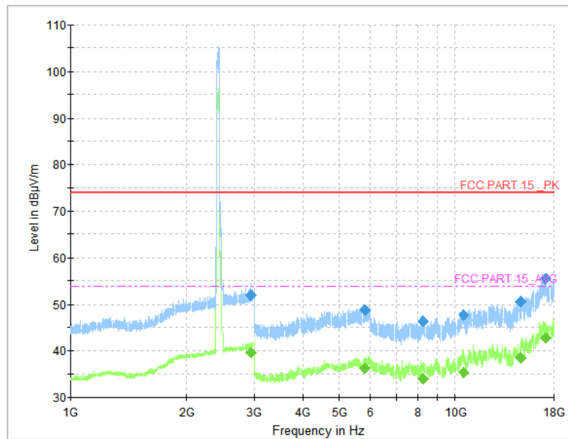
Fig.123 Radiated Spurious Emission (802.11n-HT40, CH3, 1 GHz-18 GHz)
