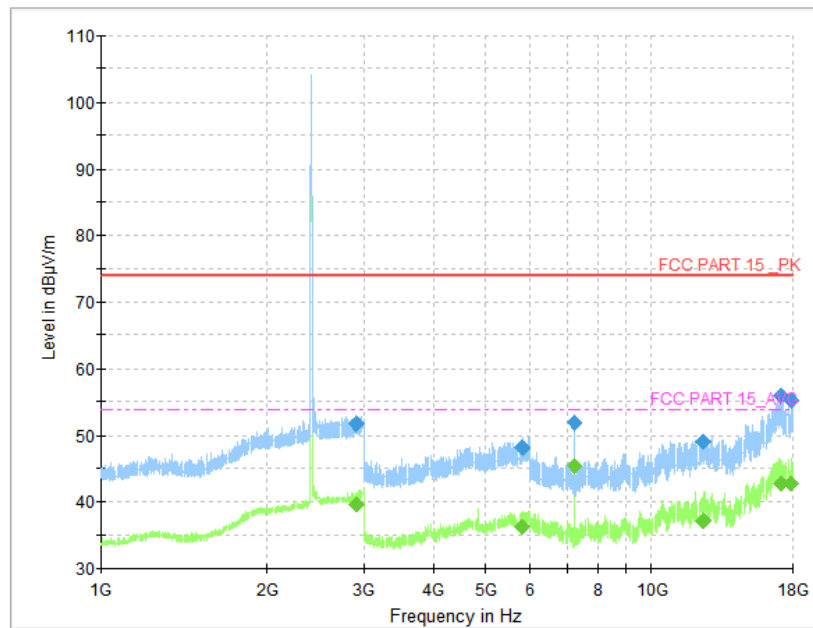
Fig.103 Radiated Spurious Emission (802.11b, CH1, 1 GHz-18GHz)
