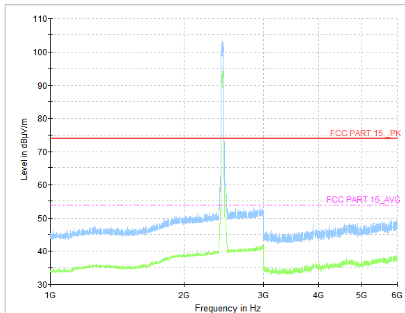
Fig.130 Radiated Spurious Emission (802.11-VHT40, CH6, 1 GHz-6 GHz)
