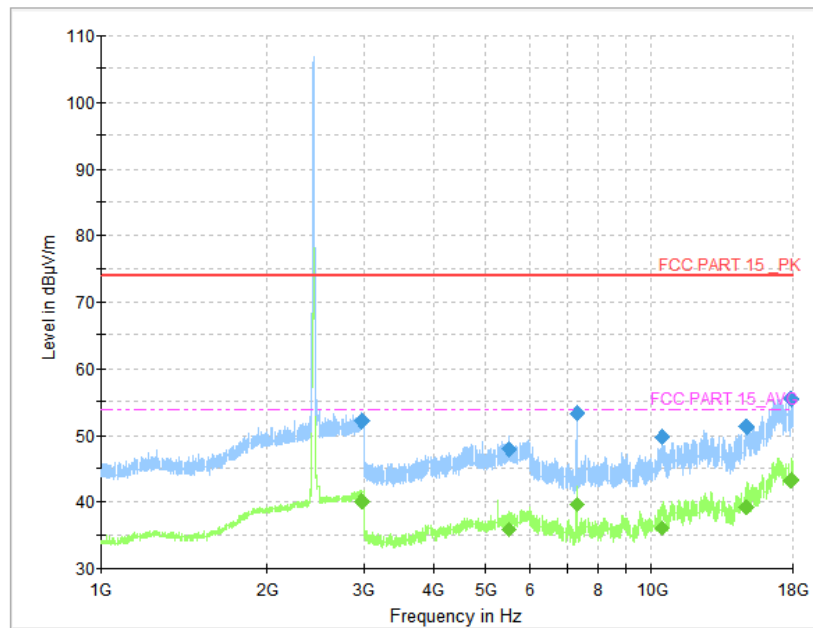
Fig.109 Radiated Spurious Emission (802.11g, CH6, 1 GHz-18 GHz)
