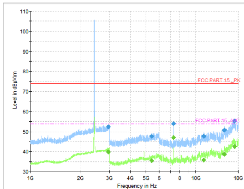
Fig.104 Radiated Spurious Emission (802.11b, CH6, 1 GHz-18GHz)
