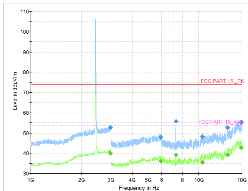
Fig.114 Radiated Spurious Emission (802.11n-HT20, CH6, 1 GHz-18 GHz)
