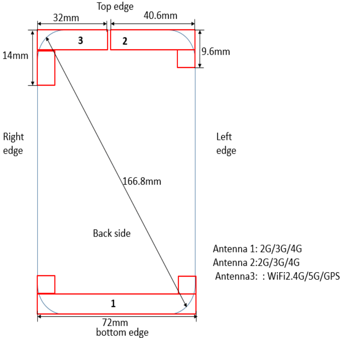
Figure: The location of the antennas
