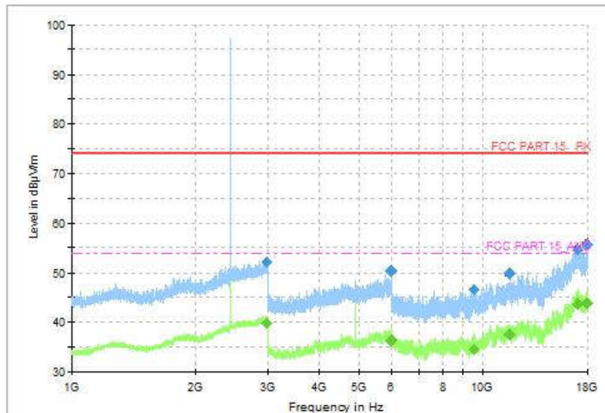
Fig. 24 Radiated Spurious Emission (GFSK, CH39, 1GHz ~18GHz)
