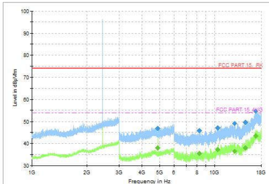
Fig. 34 Radiated Spurious Emission (8DPSK, CH39, 1GHz ~18GHz)
