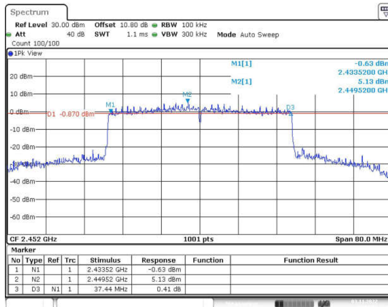
Fig.39 6dB Bandwidth (802.11ax-HE40, CH9)
