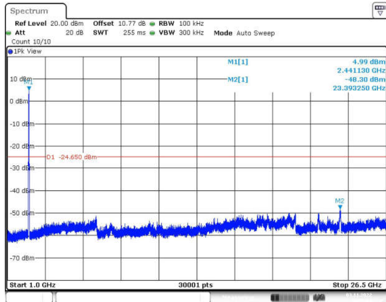
Fig.72 Conducted Spurious Emission (1GHz-26.5GHz, 802.11n-HT40, CH6)
