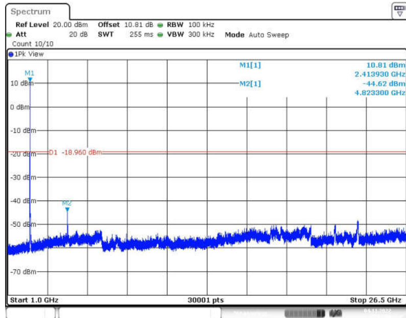
Fig.56 Conducted Spurious Emission (1GHz-26.5GHz, 802.11b, CH1)
