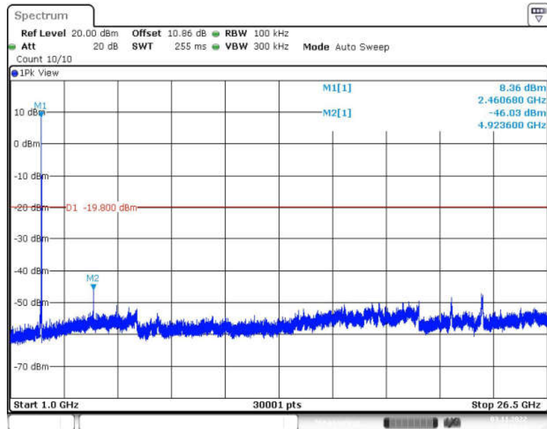
Fig.58 Conducted Spurious Emission (1GHz-26.5GHz, 802.11b, CH11)
