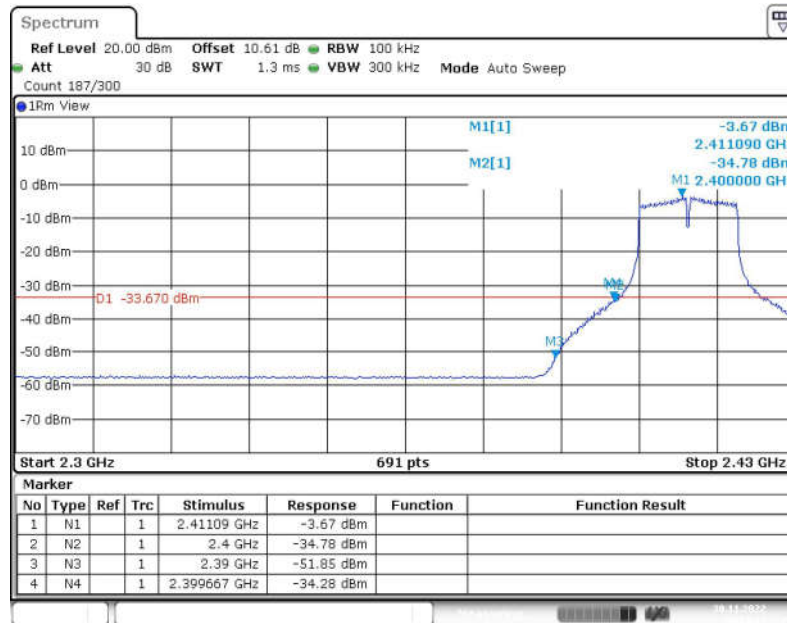
Fig.42 Band Edges (802.11g, CH1)
