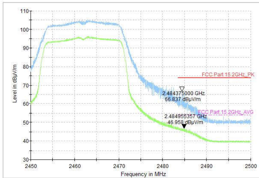
Fig.95 Radiated Restricted Band (802.11n-HT20, CH11, 2.45GHz~2.5GHz)
