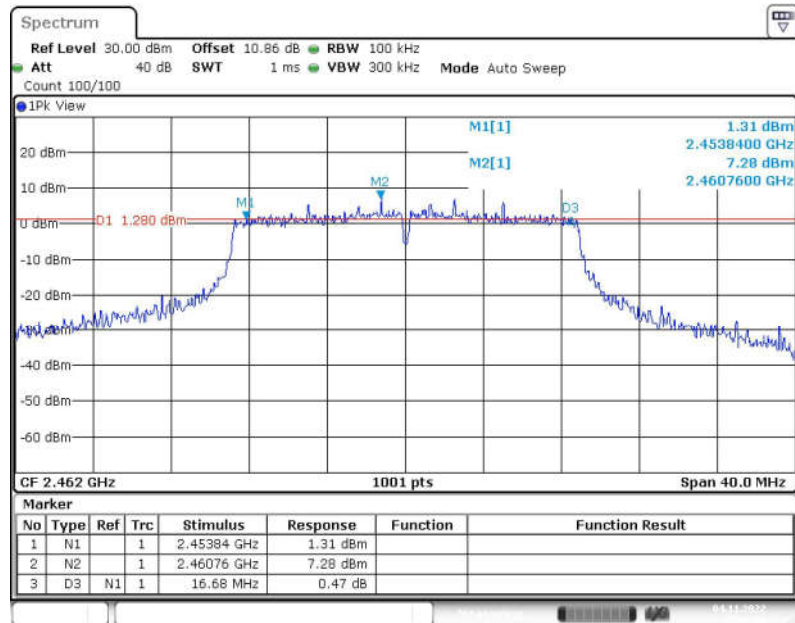
Fig.24 6dB Bandwidth (802.11n-HT20, CH11)
