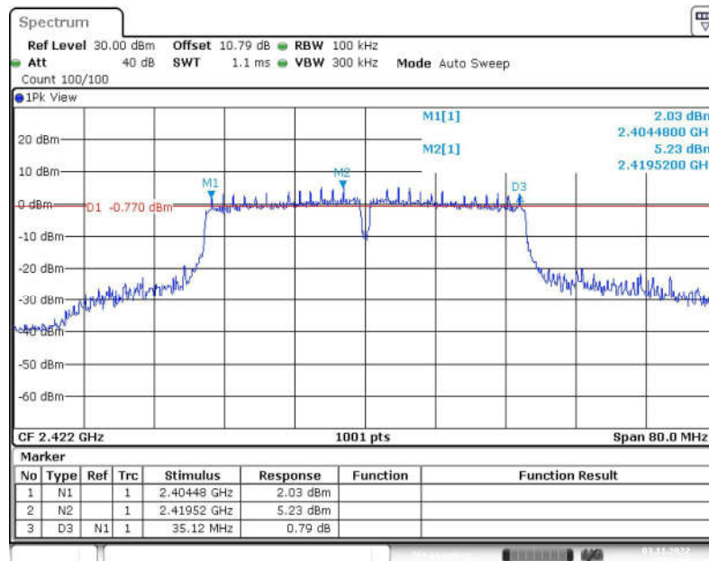
Fig.31 6dB Bandwidth (802.11n-HT40, CH3)
