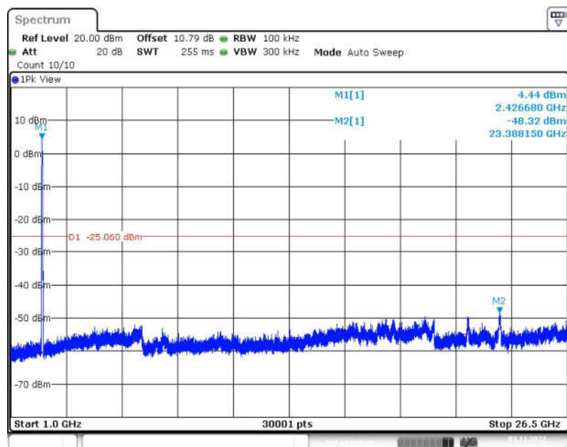
Fig.77 Conducted Spurious Emission (1GHz-26.5GHz, 802.11ax-HE40, CH3)
