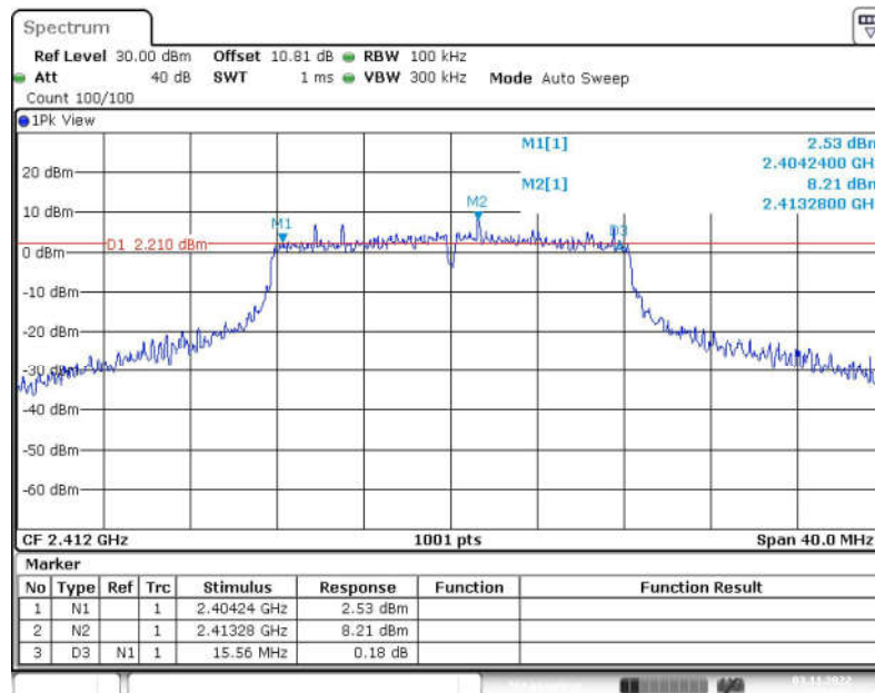
Fig.19 6dB Bandwidth (802.11g, CH1)
