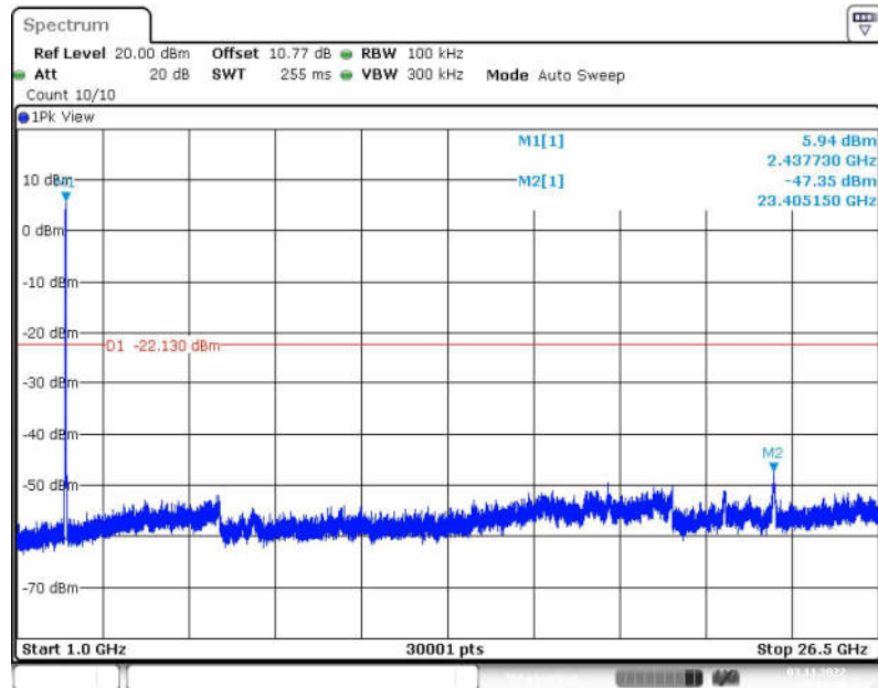
Fig.60 Conducted Spurious Emission (1GHz-26.5GHz, 802.11g, CH6)
