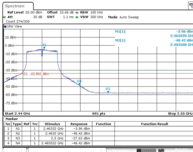
Fig.45 Band Edges (802.11n-HT20, CH11)
