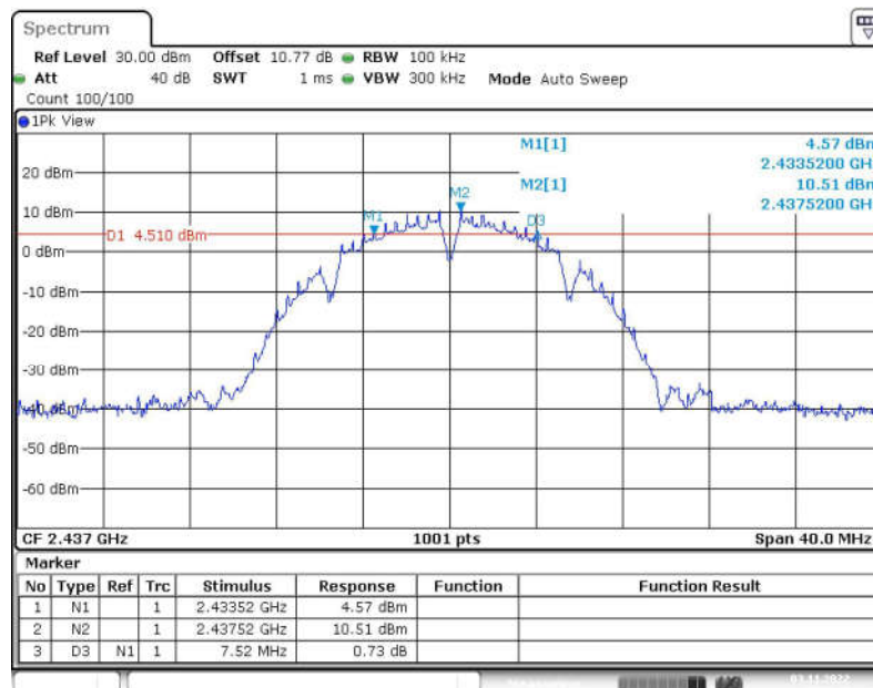
Fig.17 6dB Bandwidth (802.11b, CH6)
