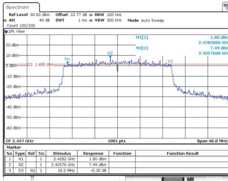
Fig.29 6dB Bandwidth (802.11ax-HE20, CH6)
