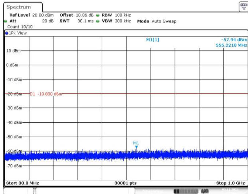
Fig.80 Conducted Spurious Emission (All Channels, 30MHz -1GHz)
