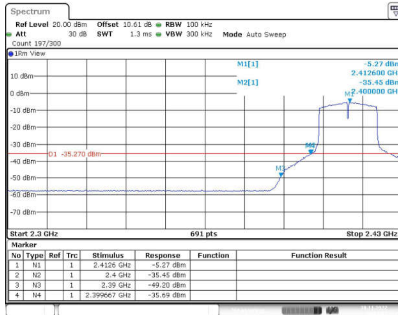
Fig.48 Band Edges (802.11ax-HE20, CH1)
