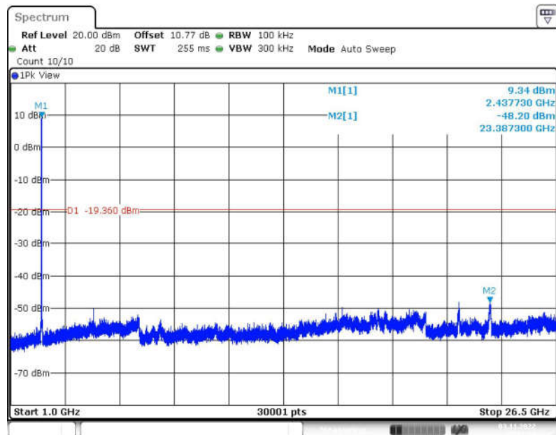
Fig.57 Conducted Spurious Emission (1GHz-26.5GHz, 802.11b, CH6)
