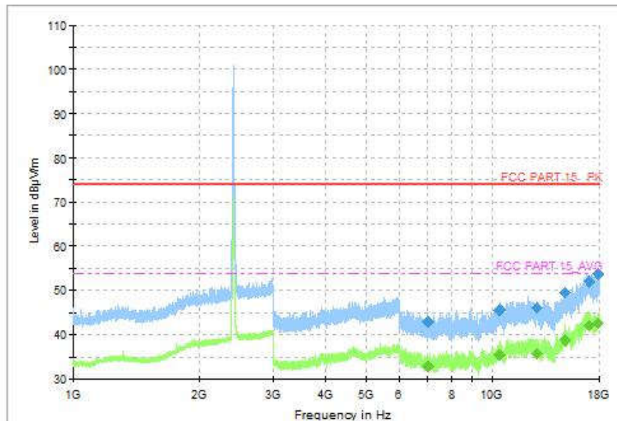
Fig.96 Radiated Spurious Emission (802.11-VHT20, CH1, 1GHz-18GHz)
