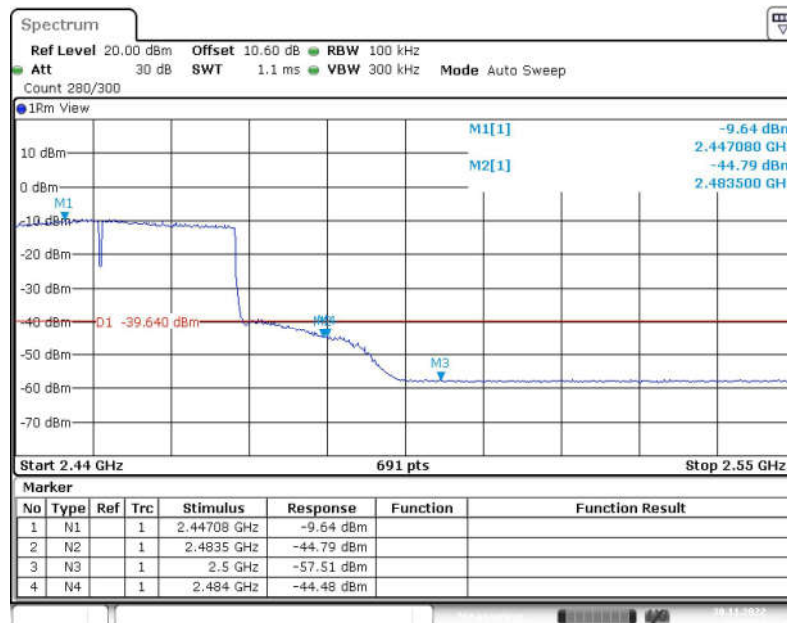
Fig.55 Band Edges (802.11ax-HE40, CH9)
