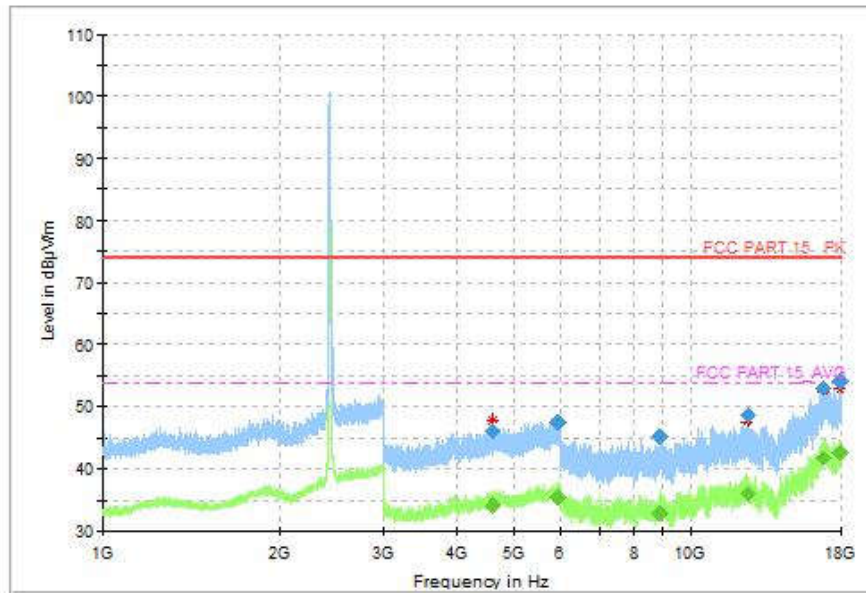
Fig.87 Radiated Spurious Emission (802.11g, CH6, 1GHz-18GHz)
