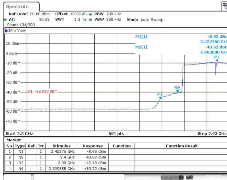
Fig.54 Band Edges (802.11ax-HE40, CH3)
