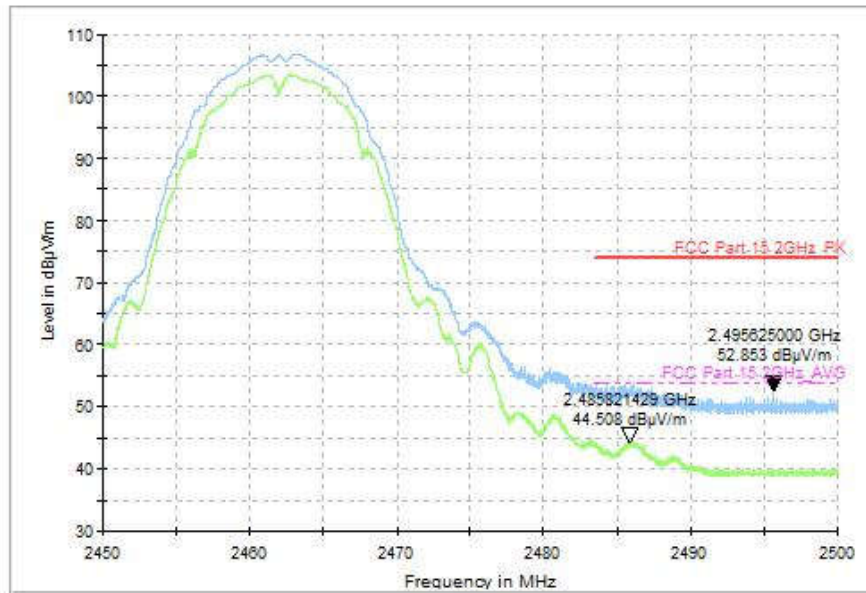
Fig.85 Radiated Restricted Band (802.11b, CH11, 2.45GHz~2.50GHz)
