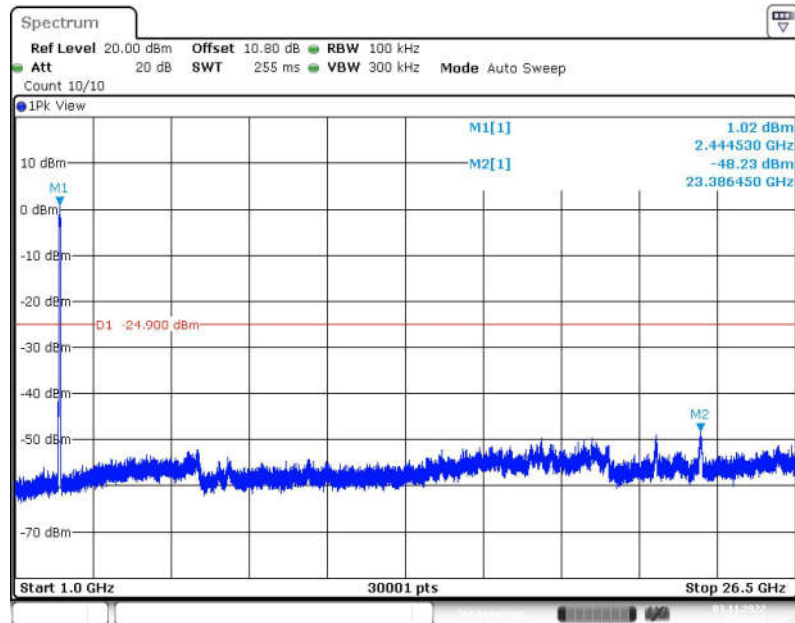
Fig.76 Conducted Spurious Emission (1GHz-26.5GHz, 802.11-VHT40, CH9)
