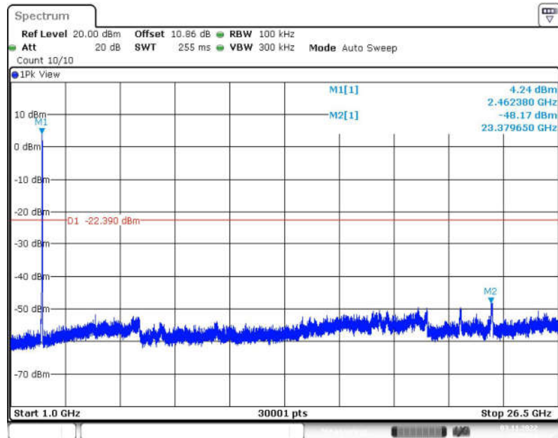
Fig.64 Conducted Spurious Emission (1GHz-26.5GHz, 802.11n-HT20, CH11)
