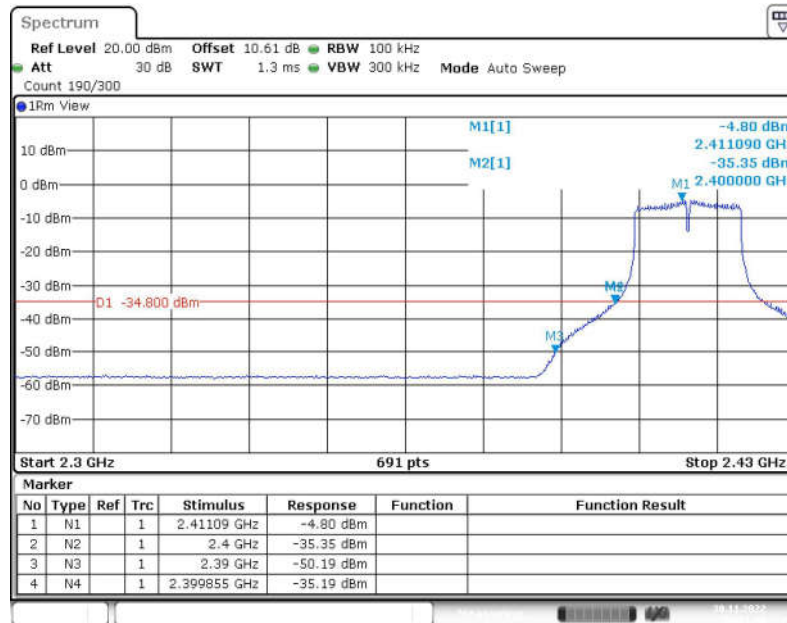
Fig.46 Band Edges (802.11-VHT20, CH1)
