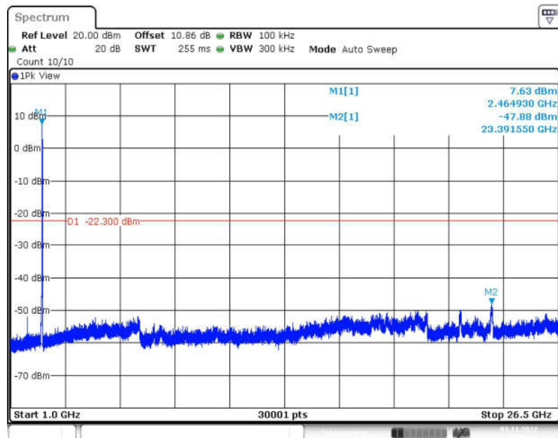
Fig.61 Conducted Spurious Emission (1GHz-26.5GHz, 802.11g, CH11)
