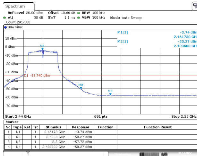
Fig.43 Band Edges (802.11g, CH11)
