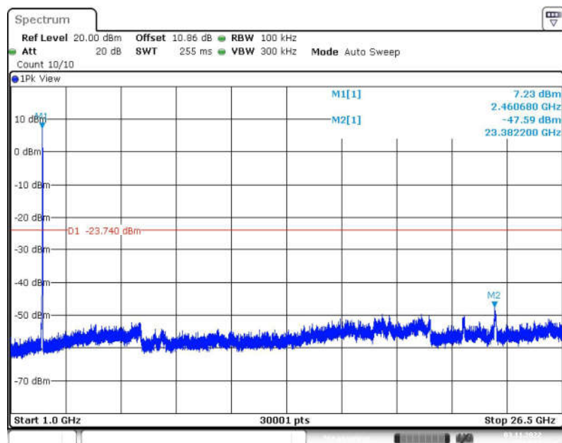
Fig.67 Conducted Spurious Emission (1GHz-26.5GHz, 802.11-VHT20, CH11)
