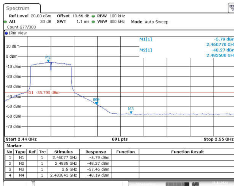
Fig.49 Band Edges (802.11ax-HE20, CH11)
