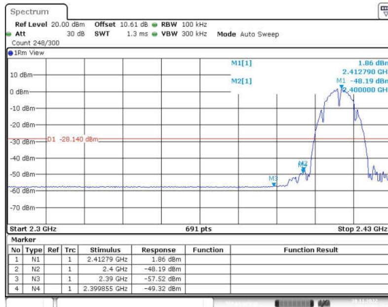
Fig.40 Band Edges (802.11b, CH1)
