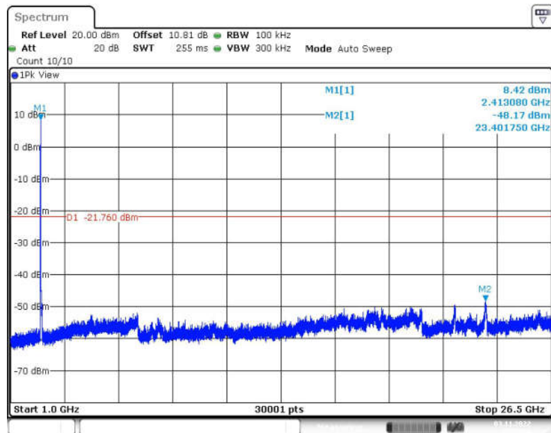
Fig.59 Conducted Spurious Emission (1GHz-26.5GHz, 802.11g, CH1)
