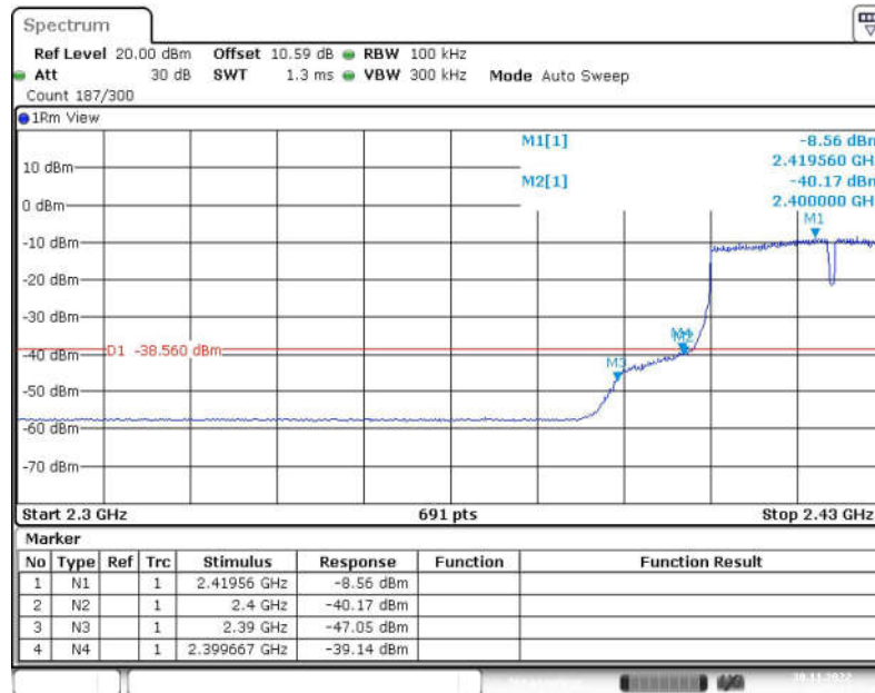
Fig.52 Band Edges (802.11-VHT40, CH3)
