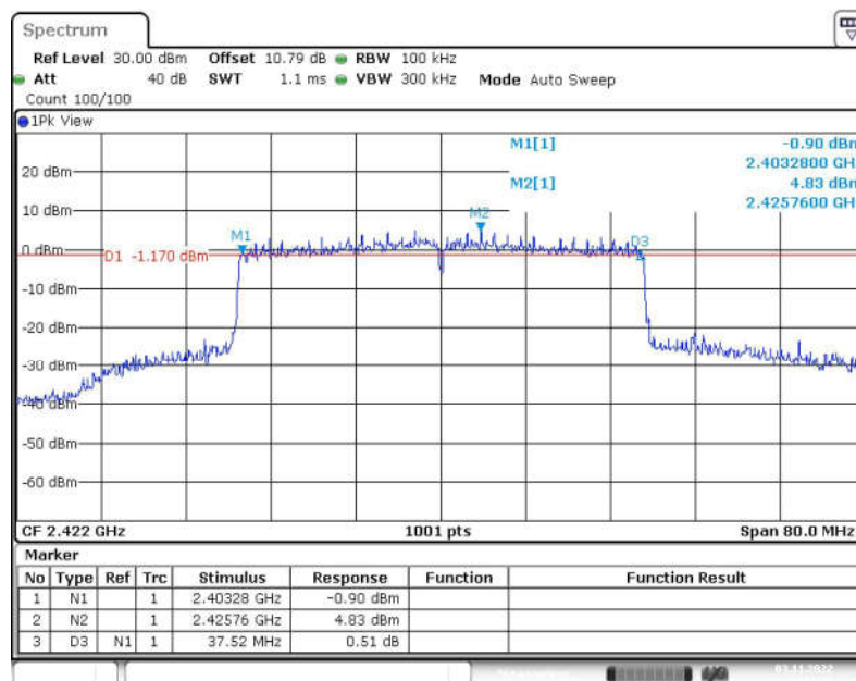
Fig.37 6dB Bandwidth (802.11ax-HE40, CH3)
