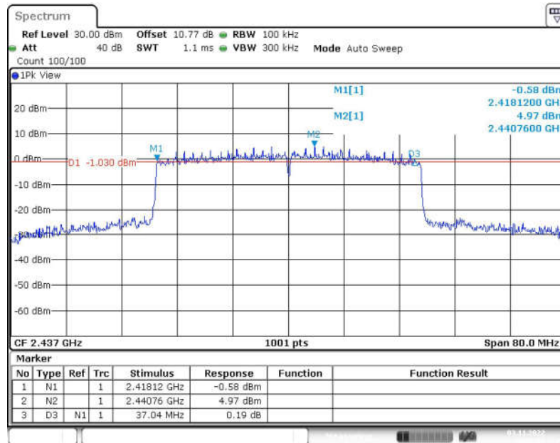
Fig.38 6dB Bandwidth (802.11ax-HE40, CH6)
