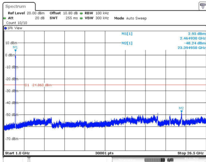
Fig.79 Conducted Spurious Emission (1GHz-26.5GHz, 802.11ax-HE40, CH9)
