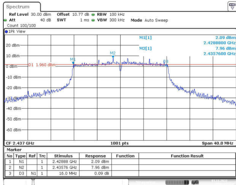
Fig.20 6dB Bandwidth (802.11g, CH6)
