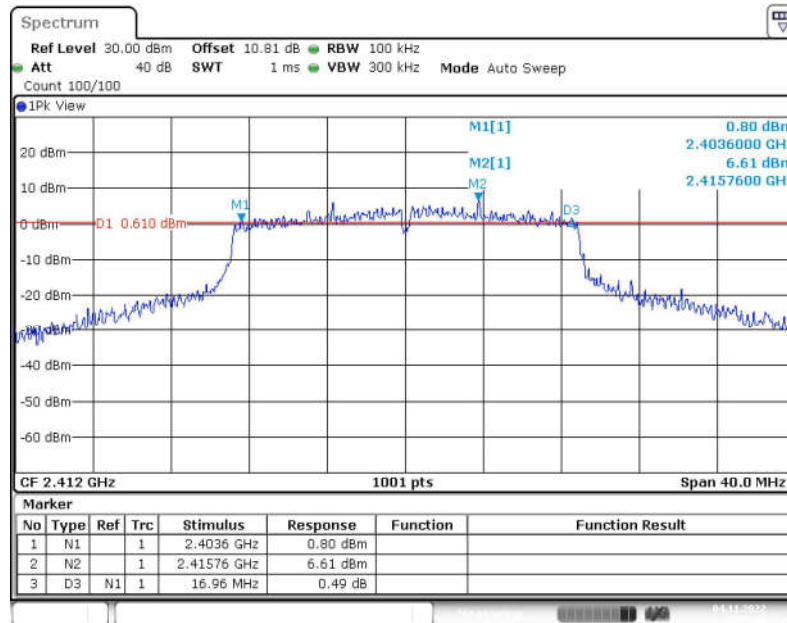
Fig.22 6dB Bandwidth (802.11n-HT20, CH1)
