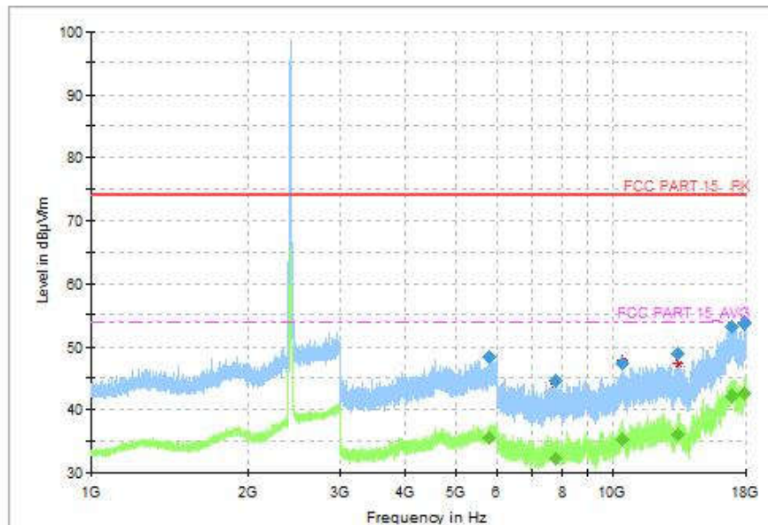
Fig.86 Radiated Spurious Emission (802.11g, CH1, 1GHz-18GHz)
