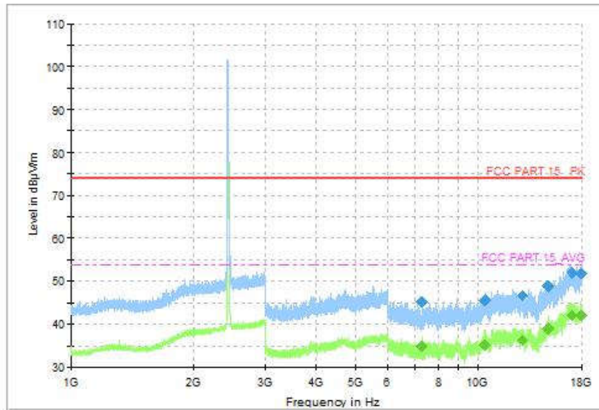
Fig.97 Radiated Spurious Emission (802.11-VHT20, CH6, 1GHz-18GHz)
