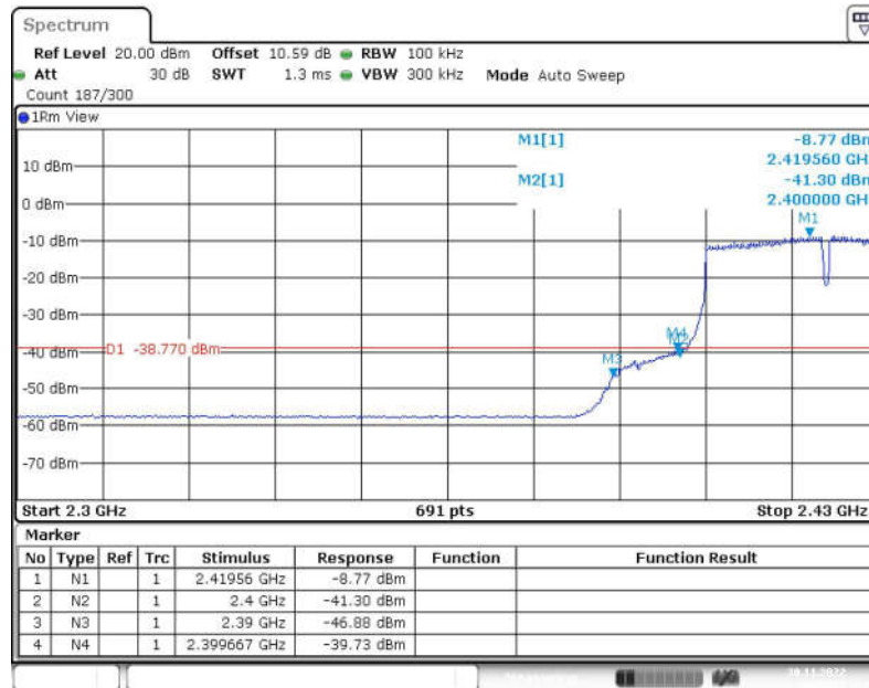
Fig.50 Band Edges (802.11n-HT40, CH3)
