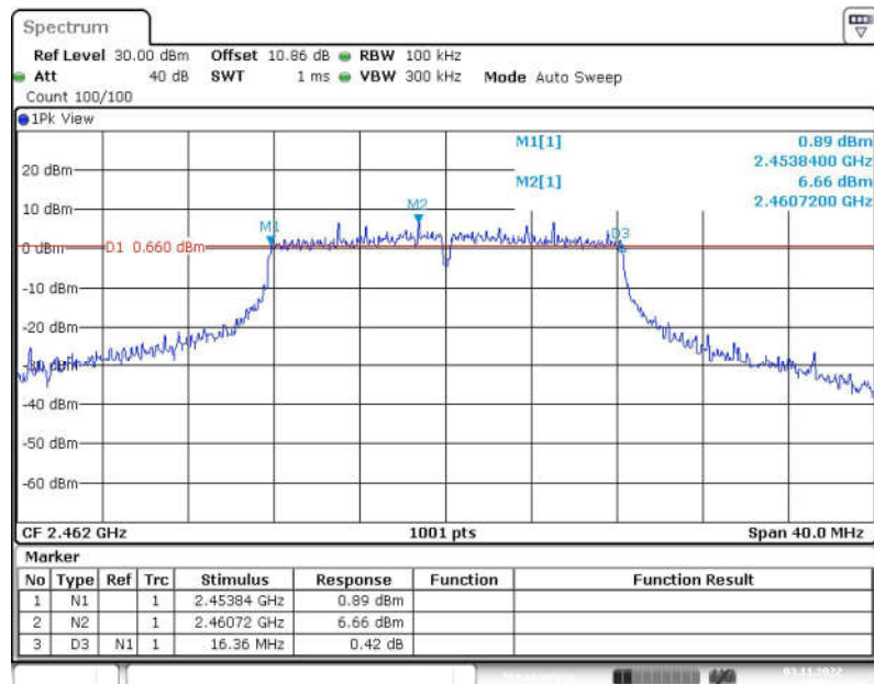
Fig.21 6dB Bandwidth (802.11g, CH11)
