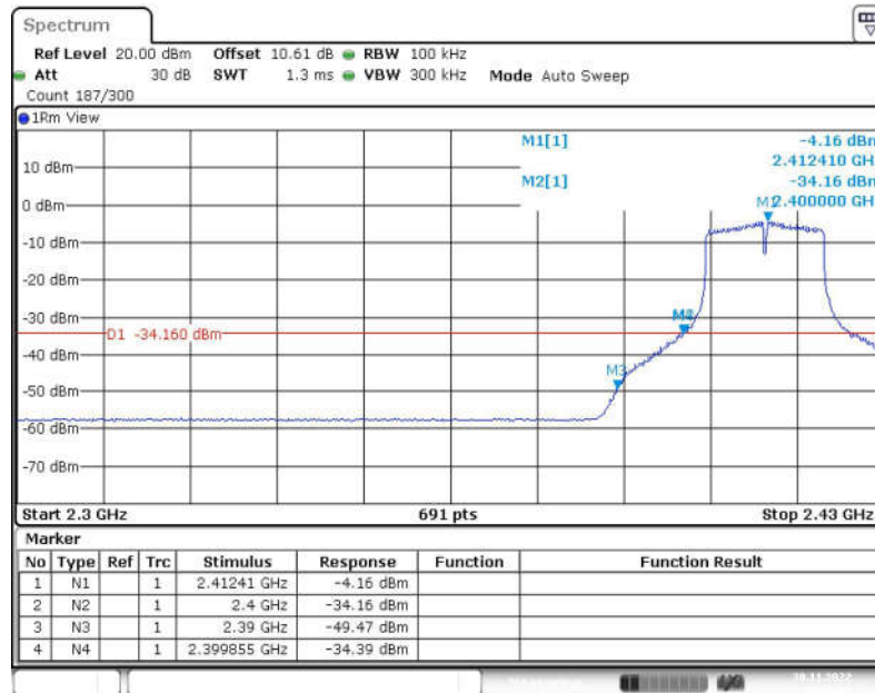
Fig.44 Band Edges (802.11n-HT20, CH1)
