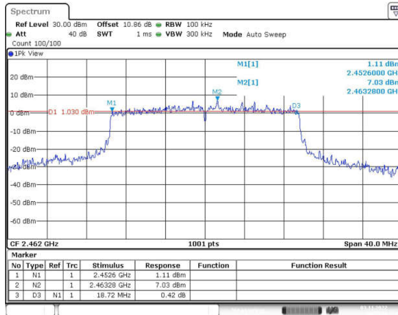
Fig.30 6dB Bandwidth (802.11ax-HE20, CH11)
