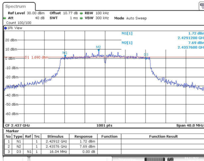
Fig.23 6dB Bandwidth (802.11n-HT20, CH6)
