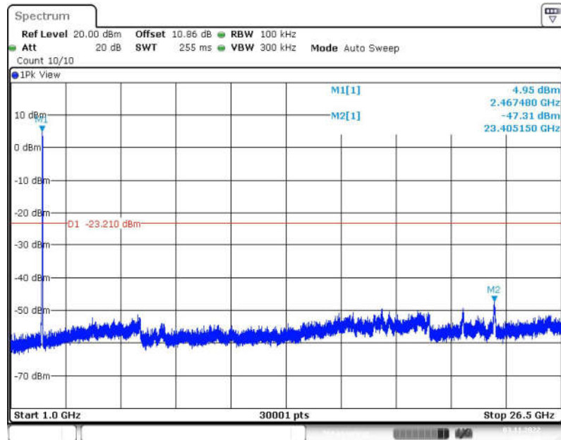
Fig.70 Conducted Spurious Emission (1GHz-26.5GHz, 802.11ax-HE20, CH11)
