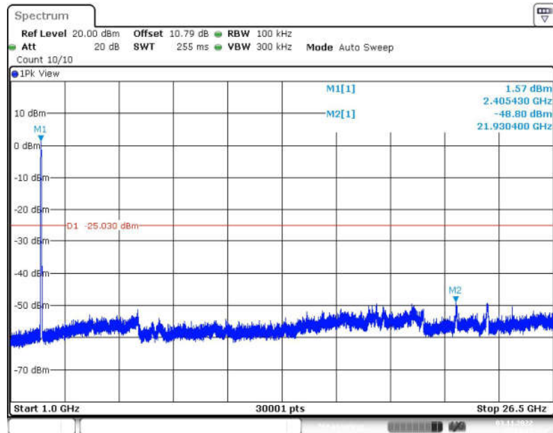
Fig.74 Conducted Spurious Emission (1GHz-26.5GHz, 802.11-VHT40, CH3)
