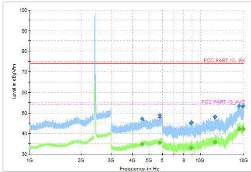
Fig.91 Radiated Spurious Emission (802.11n-HT20, CH1, 1GHz-18GHz)
