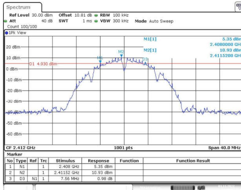
Fig.16 6dB Bandwidth (802.11b, CH1)
