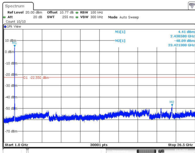
Fig.69 Conducted Spurious Emission (1GHz-26.5GHz, 802.11ax-HE20, CH6)
