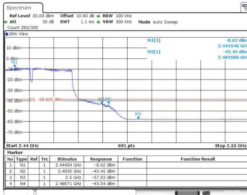
Fig.51 Band Edges (802.11n-HT40, CH9)
