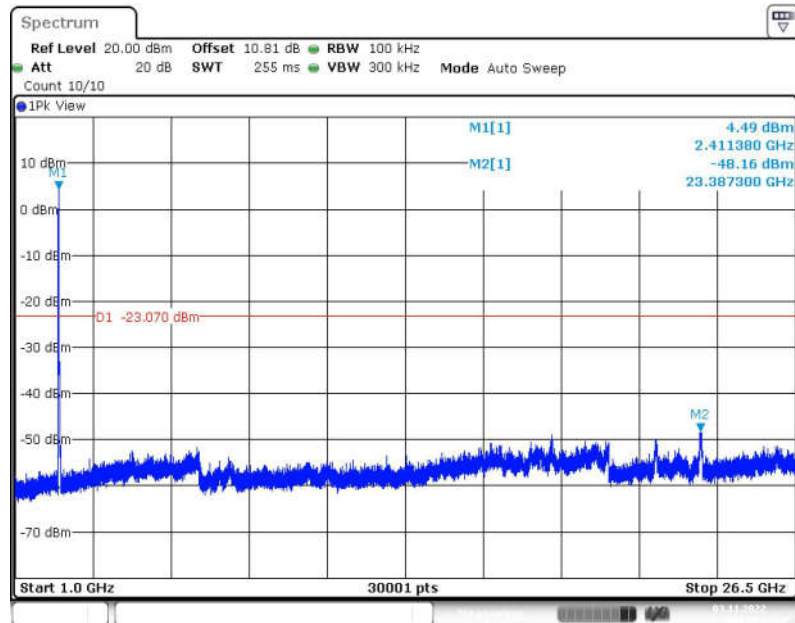
Fig.68 Conducted Spurious Emission (1GHz-26.5GHz, 802.11ax-HE20, CH1)
