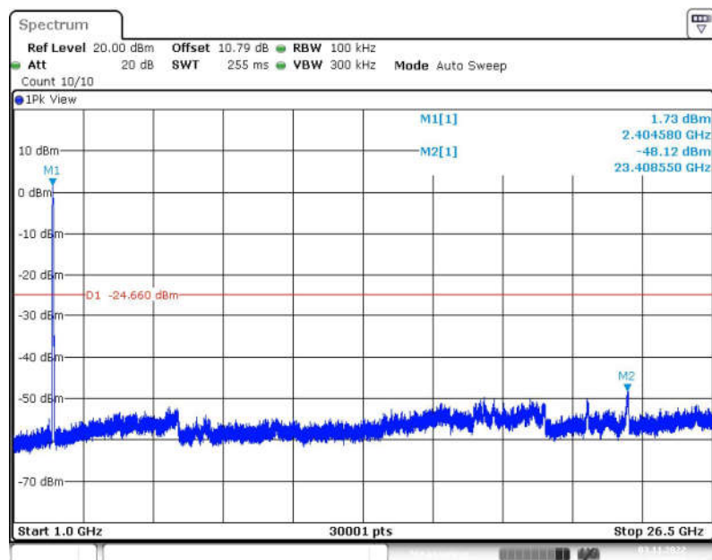
Fig.71 Conducted Spurious Emission (1GHz-26.5GHz, 802.11n-HT40, CH3)
