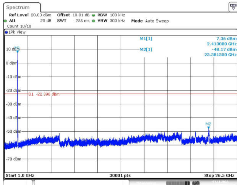
Fig.65 Conducted Spurious Emission (1GHz-26.5GHz, 802.11-VHT20, CH1)
