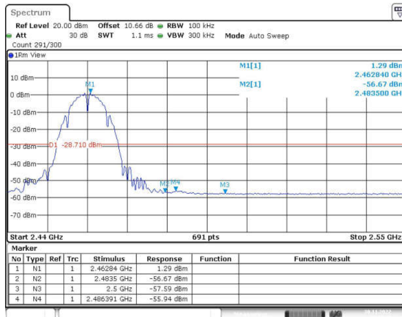
Fig.41 Band Edges (802.11b, CH11)
