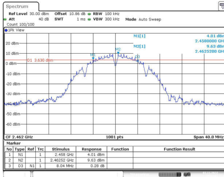
Fig.18 6dB Bandwidth (802.11b, CH11)
