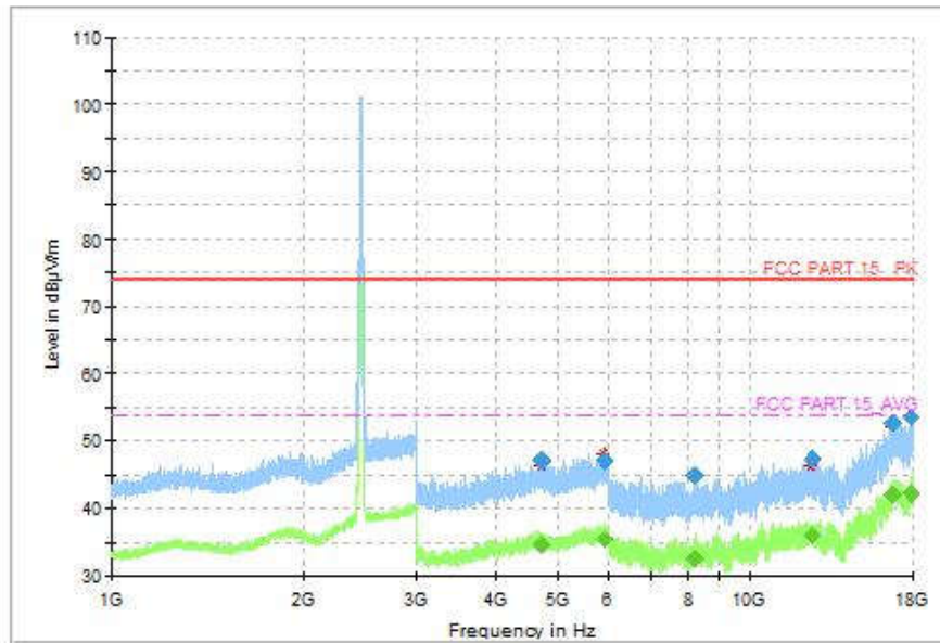
Fig.93 Radiated Spurious Emission (802.11n-HT20, CH11, 1GHz-18GHz)
