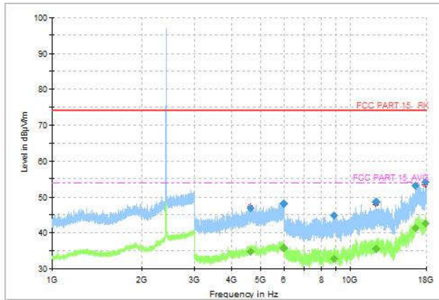
Fig.81 Radiated Spurious Emission (802.11b, CH1, 1GHz-18GHz)
