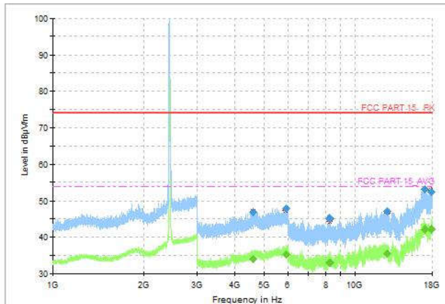
Fig.92 Radiated Spurious Emission (802.11n-HT20, CH6, 1GHz-18GHz)
