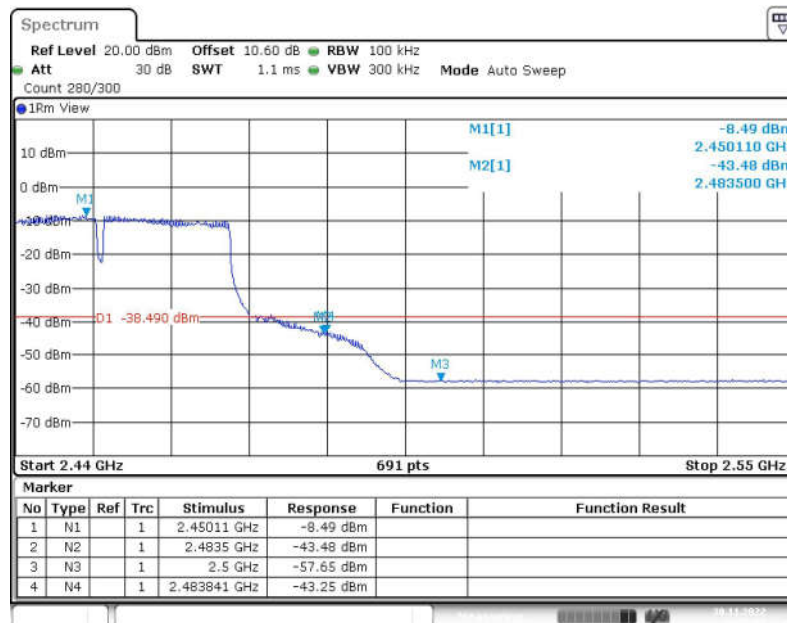
Fig.53 Band Edges (802.11-VHT40, CH9)
