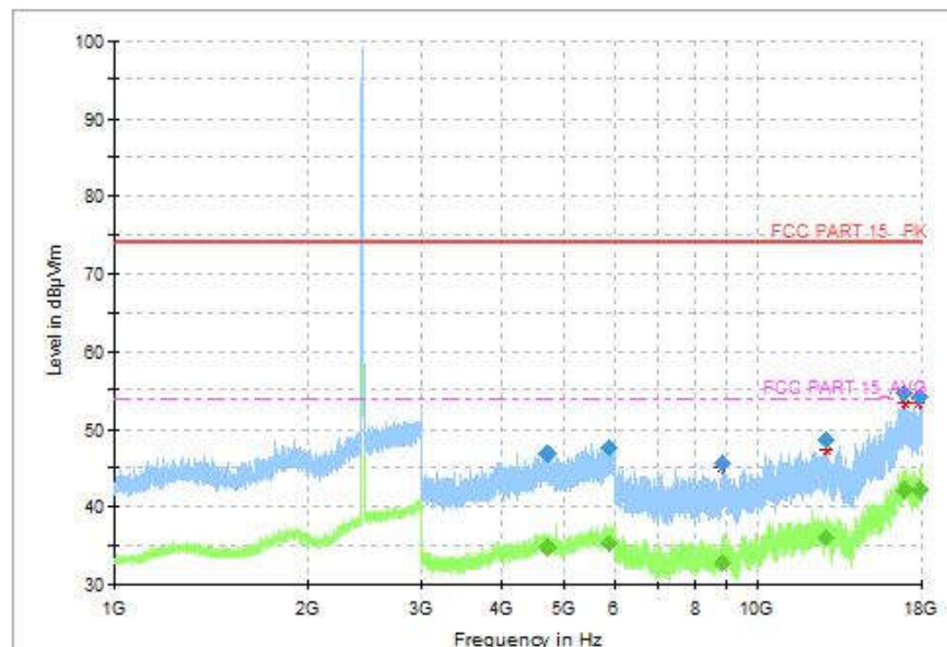
Fig.82 Radiated Spurious Emission (802.11b, CH6, 1GHz-18GHz)
