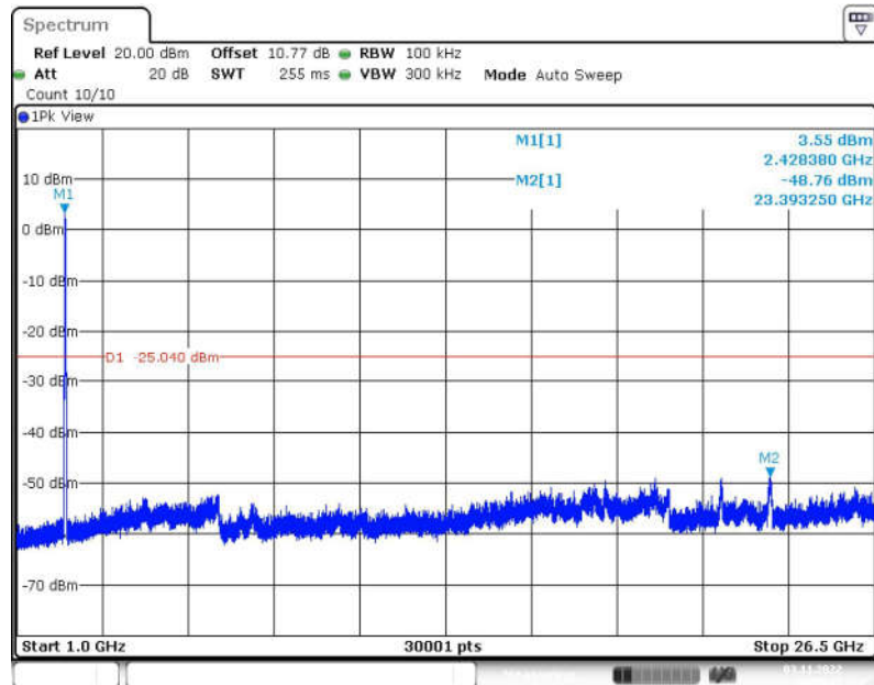
Fig.78 Conducted Spurious Emission (1GHz-26.5GHz, 802.11ax-HE40, CH6)
