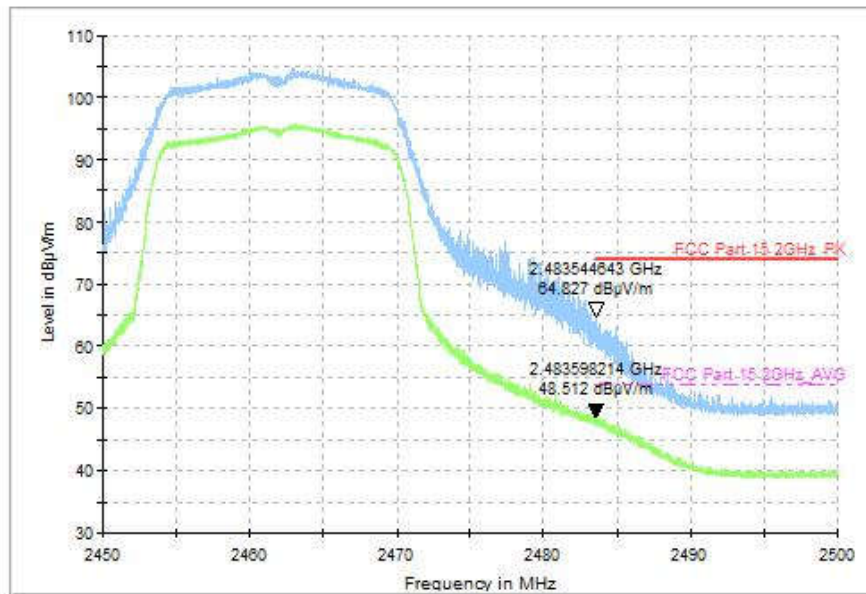
Fig.90 Radiated Restricted Band (802.11g, CH11, 2.45GHz~2.50GHz)
