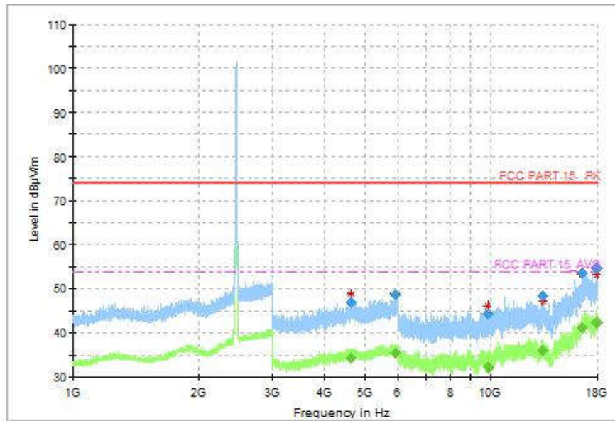
Fig.83 Radiated Spurious Emission (802.11b, CH1, 1GHz-18GHz)
