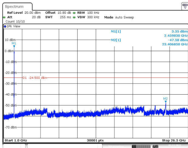
Fig.73 Conducted Spurious Emission (1GHz-26.5GHz, 802.11n-HT40, CH9)
