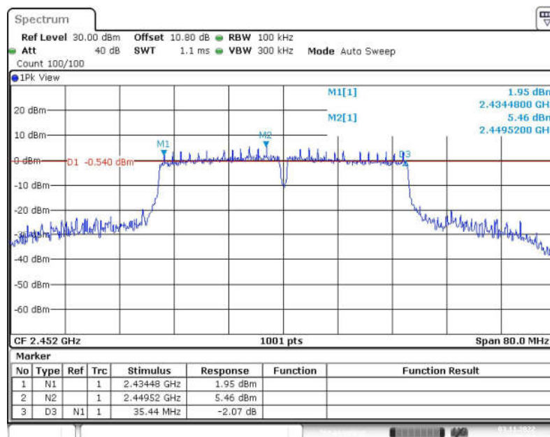
Fig.33 6dB Bandwidth (802.11n-HT40, CH9)
