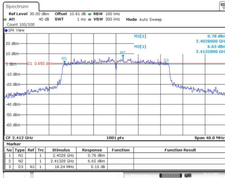
Fig.28 6dB Bandwidth (802.11ax-HE20, CH1)
