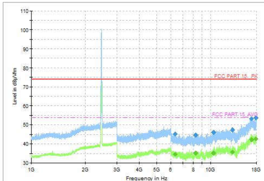
Fig.98 Radiated Spurious Emission (802.11-VHT20, CH11, 1GHz-18GHz)
