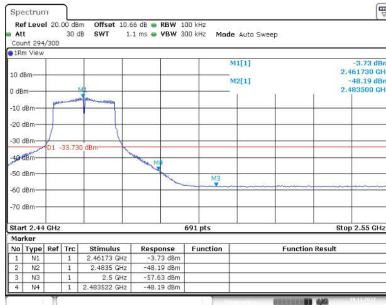
Fig.47 Band Edges (802.11-VHT20, CH11)
