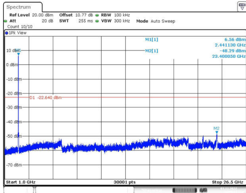
Fig.66 Conducted Spurious Emission (1GHz-26.5GHz, 802.11-VHT20, CH6)
