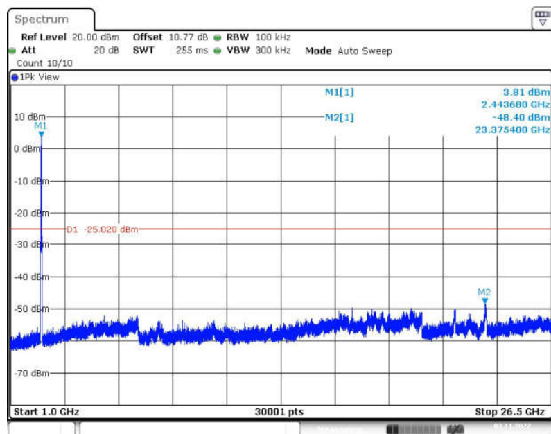
Fig.75 Conducted Spurious Emission (1GHz-26.5GHz, 802.11-VHT40, CH6)
