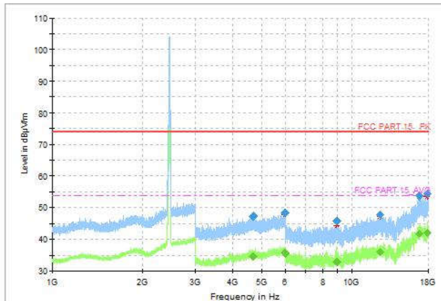
Fig.88 Radiated Spurious Emission (802.11g, CH11, 1GHz-18GHz)
