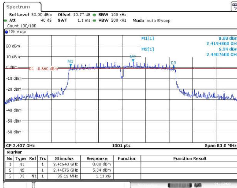
Fig.32 6dB Bandwidth (802.11n-HT40, CH6)
