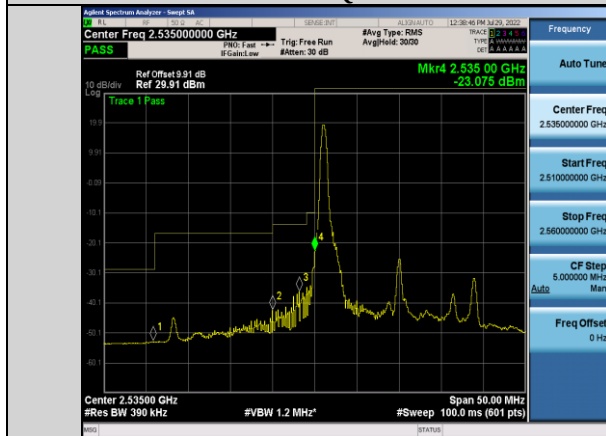
Band41-20MHz-QPSK-40140-1RB#0
