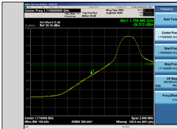
Band66-10MHz-16QAM-132022-1RB#0
