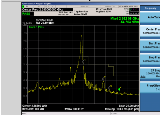
Band41-5MHz-16QAM-41215-1RB#24
