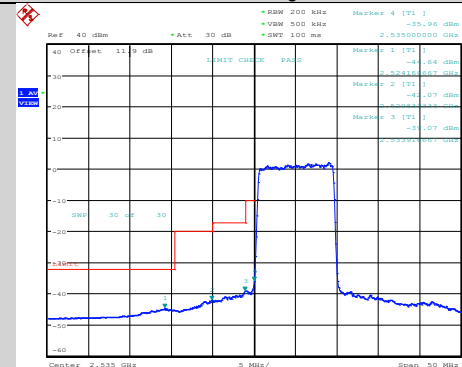
Band41-10MHz-64QAM-40090-1RB#0
