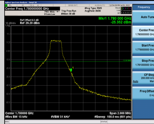
Band66-1.4MHz-16QAM-132665-1RB#5
