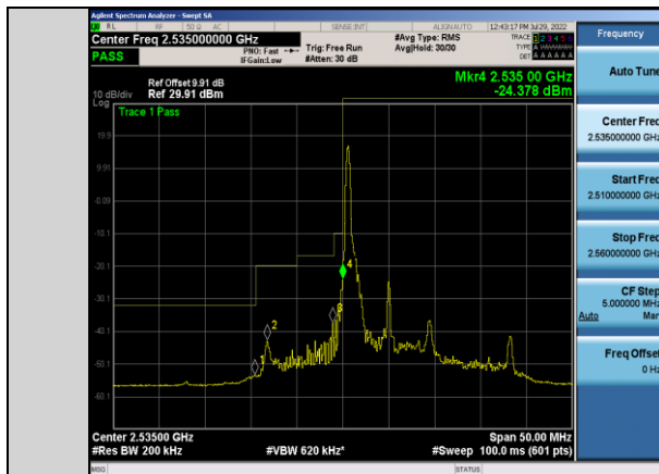
Band41-10MHz-16QAM-40090-1RB#0
