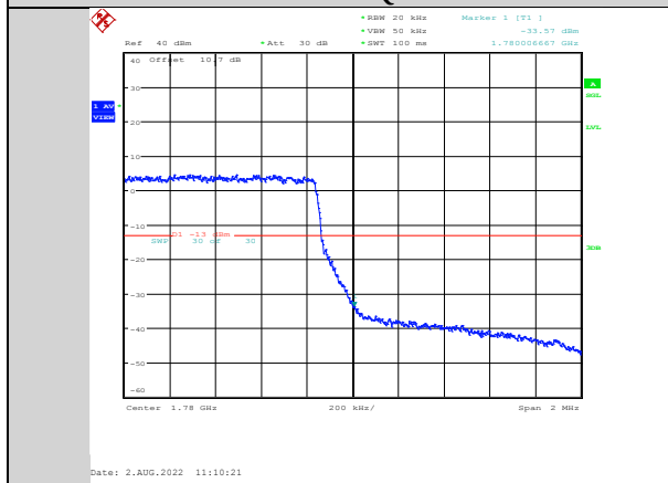
Band66-1.4MHz-64QAM-132665-6RB#0
