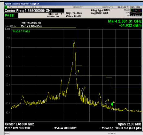
Band41-5MHz-QPSK-41215-1RB#24
