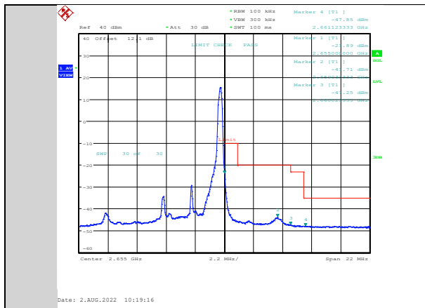
Band41-5MHz-64QAM-41215-1RB#24
