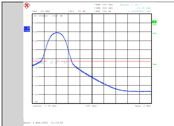
Band66-10MHz-64QAM-132622-1RB#49
