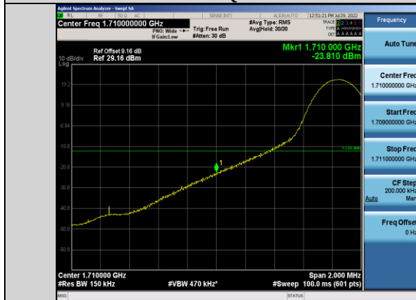
Band66-15MHz-QPSK-132047-1RB#0
