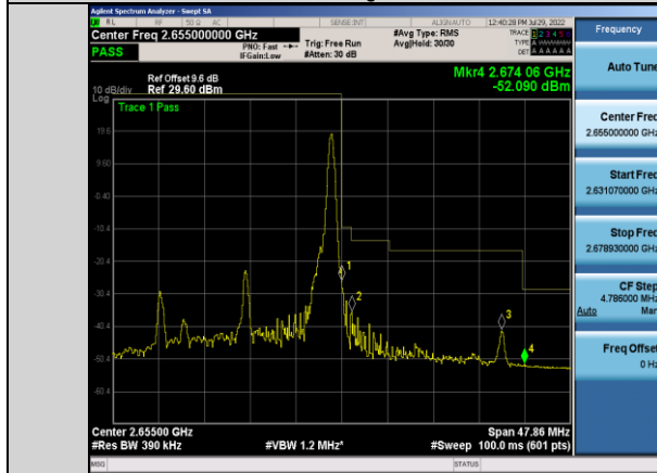
Band41-20MHz-16QAM-41140-1RB#99
