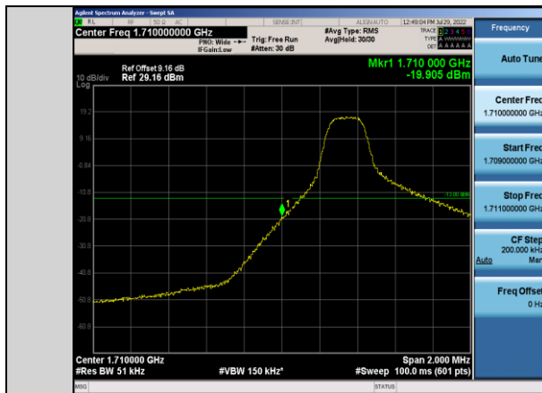
Band66-5MHz-16QAM-131997-1RB#0
