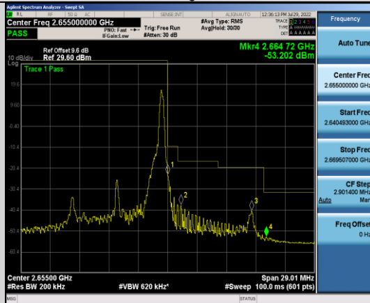
Band41-10MHz-16QAM-41190-1RB#49
