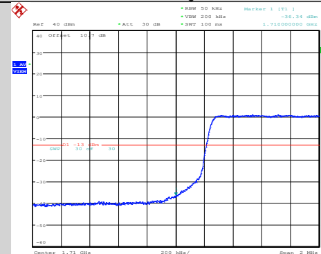
Band66-5MHz-64QAM-131997-1RB#0
