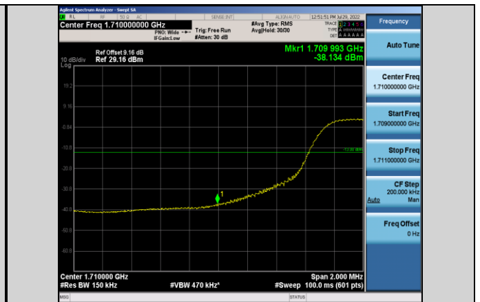
Band66-15MHz-QPSK-132047-75RB#0
