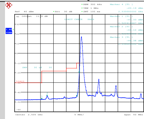
Band41-15MHz-16QAM-41165-75RB#0
