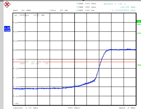
Band66-10MHz-64QAM-132022-1RB#0
