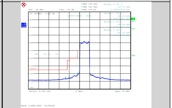
Band41-5MHz-64QAM-40065-25RB#0
