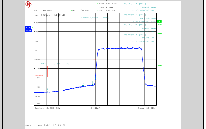
Band41-20MHz-64QAM-40140-100RB#0
