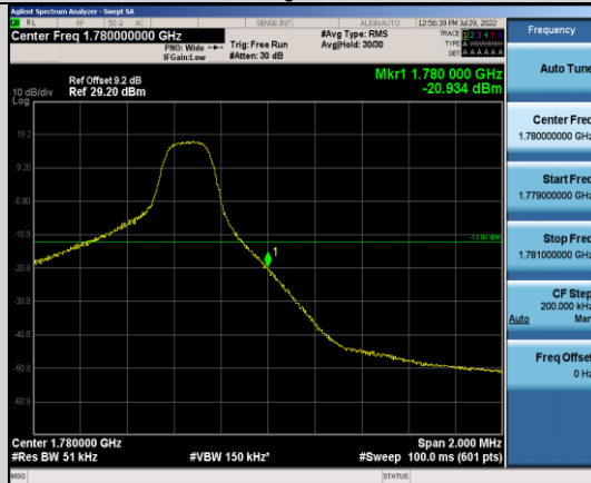
Band66-5MHz-16QAM-132647-1RB#24
