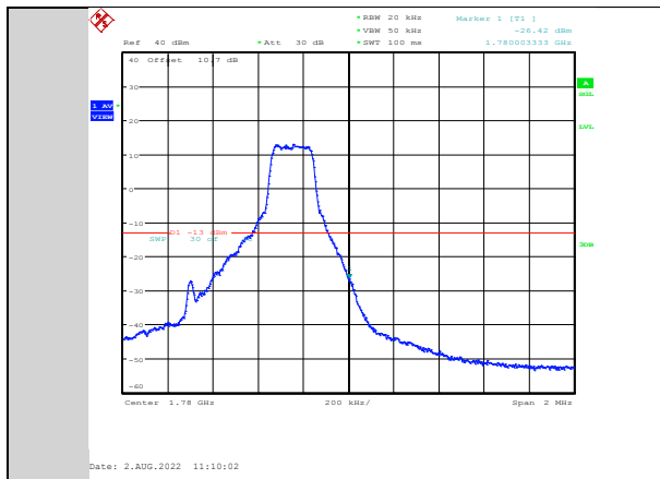
Band66-1.4MHz-64QAM-132665-1RB#5
