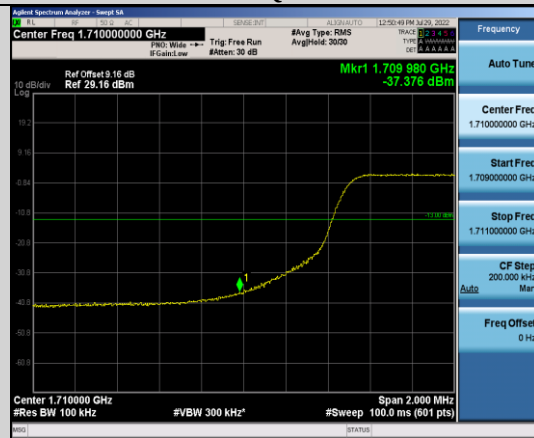
Band66-10MHz-16QAM-132022-50RB#0
