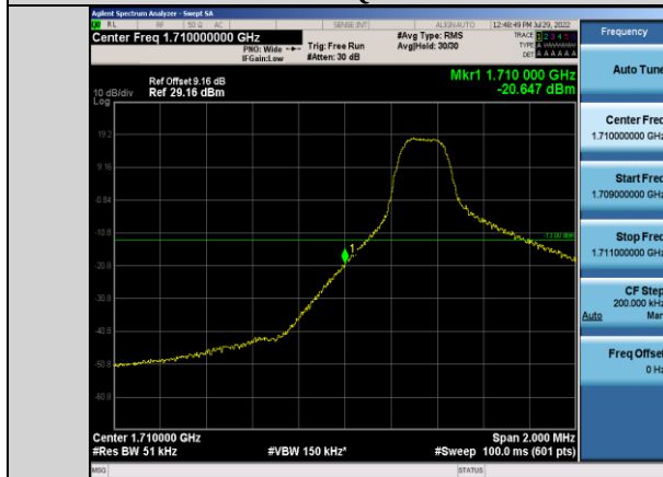
Band66-5MHz-QPSK-131997-1RB#0
