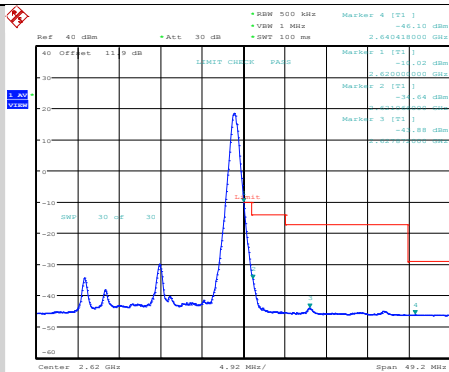
Band38-20MHz-64QAM-38150-1RB#99
