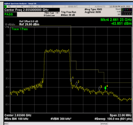
Band41-5MHz-QPSK-41215-25RB#0
