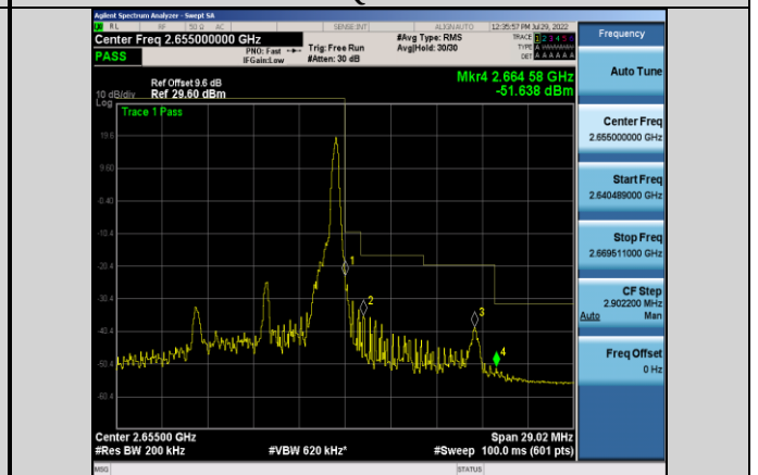
Band41-10MHz-QPSK-41190-1RB#49
