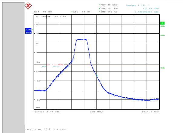
Band66-3MHz-64QAM-132657-1RB#14
