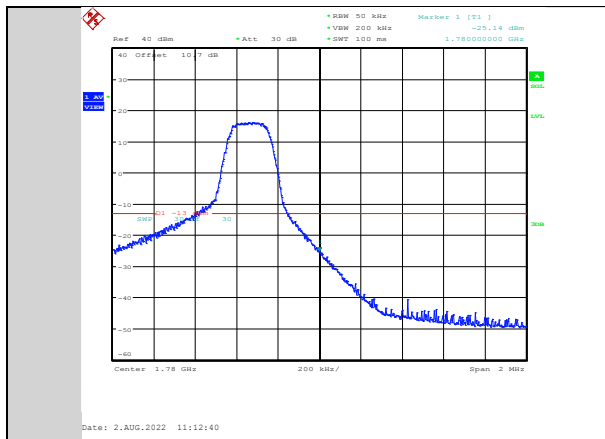
Band66-5MHz-64QAM-132647-1RB#24
