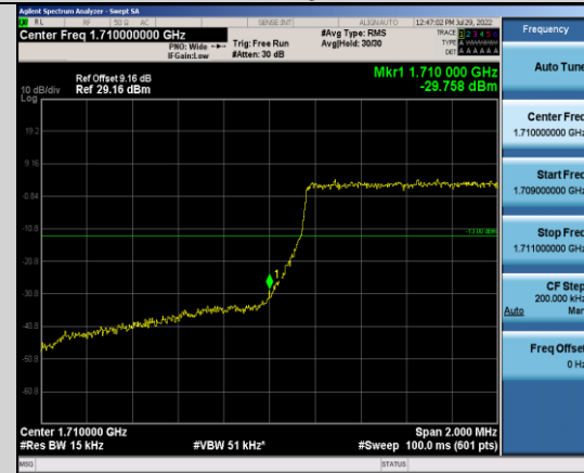
Band66-1.4MHz-16QAM-131979-6RB#0
