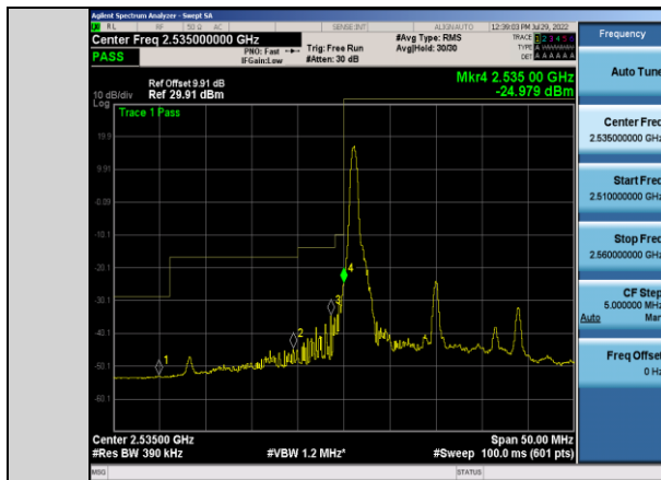
Band41-20MHz-16QAM-40140-1RB#0
