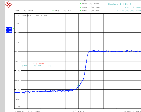
Band66-3MHz-64QAM-131987-1RB#0
