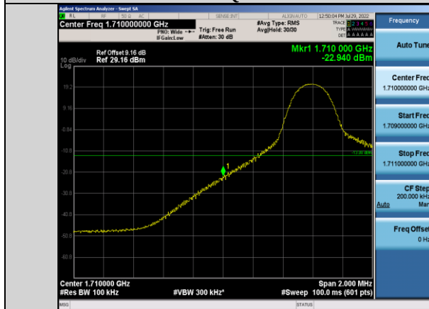
Band66-10MHz-QPSK-132022-1RB#0
