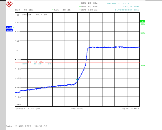
Band66-1.4MHz-64QAM-131979-6RB#0
