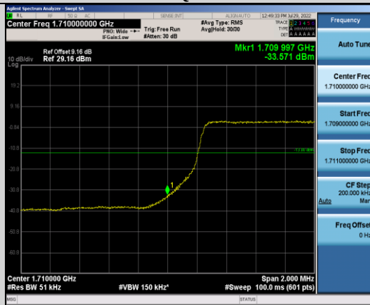
Band66-5MHz-16QAM-131997-25RB#0
