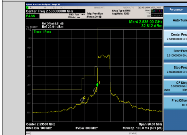
Band41-5MHz-16QAM-40065-25RB#0
