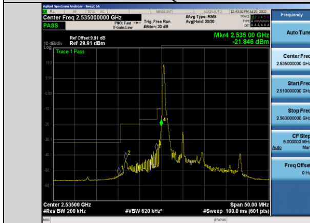
Band41-10MHz-QPSK-40090-1RB#0
