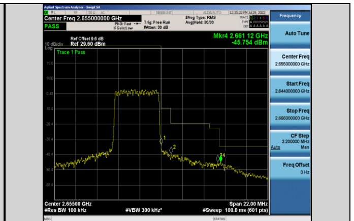
Band41-5MHz-16QAM-41215-25RB#0
