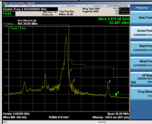
Band41-15MHz-16QAM-41165-1RB#74
