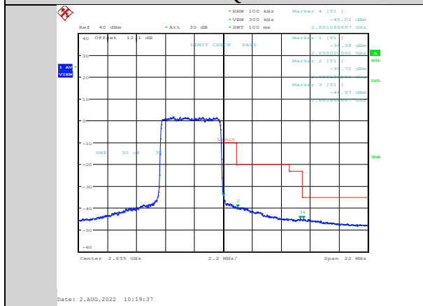
Band41-5MHz-64QAM-41215-25RB#0
