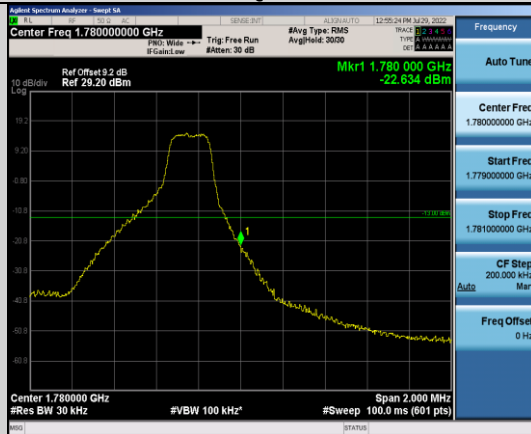
Band66-3MHz-16QAM-132657-1RB#14
