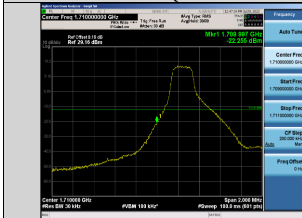
Band66-3MHz-QPSK-131987-1RB#0
