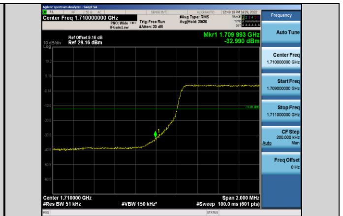
Band66-5MHz-QPSK-131997-25RB#0
