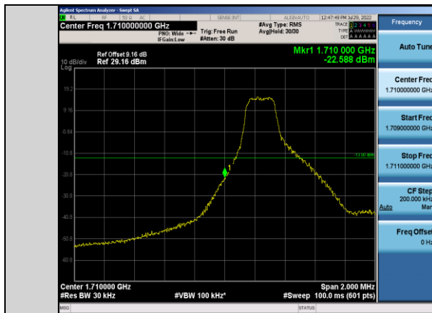
Band66-3MHz-16QAM-131987-1RB#0
