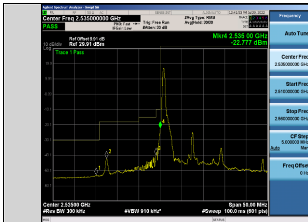
Band41-15MHz-16QAM-40115-1RB#0
