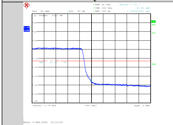
Band66-3MHz-64QAM-132657-15RB#0
