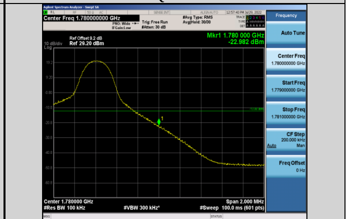
Band66-10MHz-QPSK-132622-1RB#49
