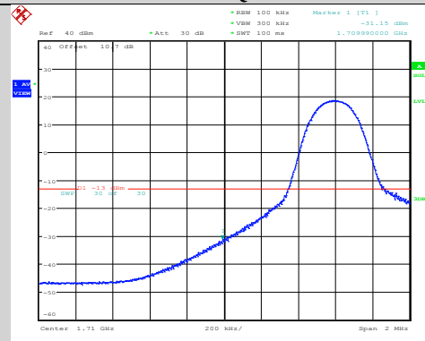
Band66-10MHz-16QAM-132622-50RB#0
