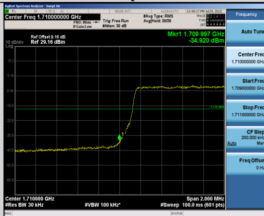
Band66-3MHz-16QAM-131987-15RB#0
