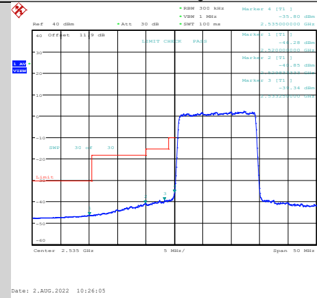
Band41-15MHz-64QAM-40115-75RB#0
