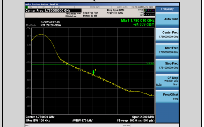
Band66-15MHz-QPSK-132597-1RB#74
