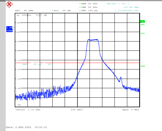
Band66-1.4MHz-64QAM-131979-1RB#0
