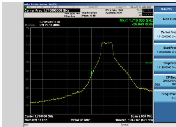
Band66-1.4MHz-16QAM-131979-1RB#0
