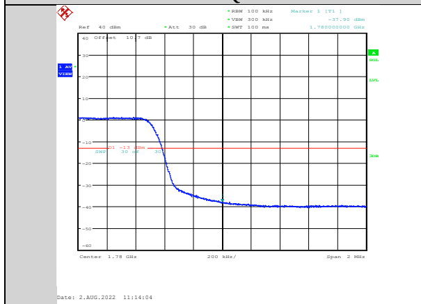
Band66-10MHz-64QAM-132622-50RB#0
