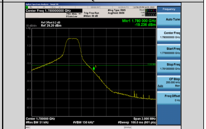
Band66-5MHz-QPSK-132647-1RB#24
