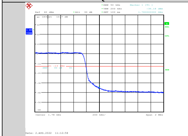
Band66-5MHz-64QAM-132647-25RB#0
