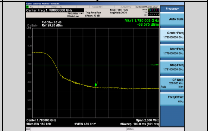
Band66-15MHz-QPSK-132597-75RB#0
