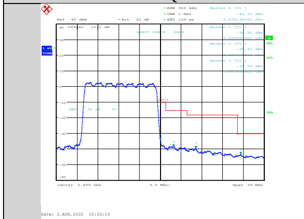
Band41-15MHz-64QAM-41165-75RB#0
