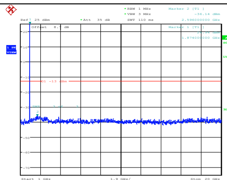
Band2-1.4MHz-16QAM-18900-1RB#0- Range2:1000~20000MHz
