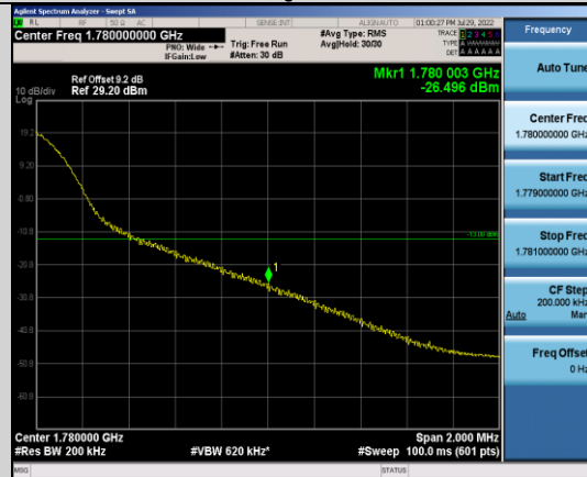
Band66-20MHz-16QAM-132572-1RB#99
