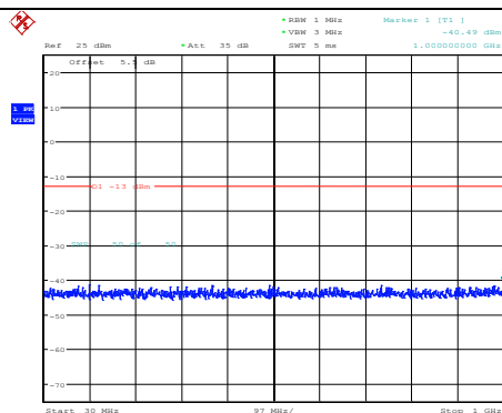
Band2-1.4MHz-16QAM-18607-1RB#0- Range1:30~1000MHz
