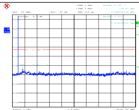
Band2-3MHz-64QAM-18900-1RB#0- Range2:1000~20000MHz
