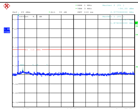
Band2-10MHz-16QAM-18900-1RB#0- Range2:1000~20000MHz
