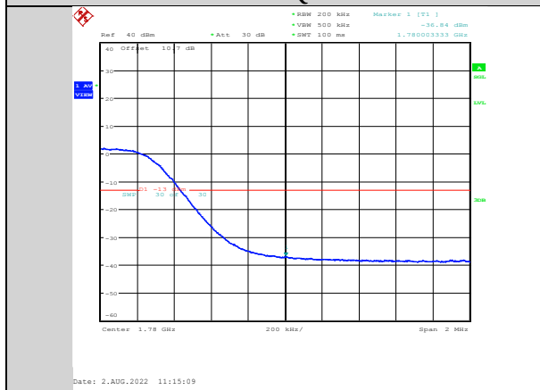
Band66-15MHz-64QAM-132597-75RB#0
