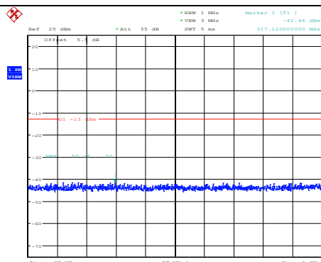
Band2-10MHz-QPSK-18650-1RB#0- Range1:30~1000MHz
