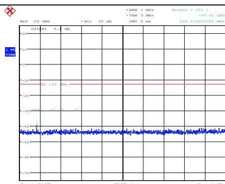
Band2-3MHz-16QAM-18615-1RB#0- Range1:30~1000MHz
