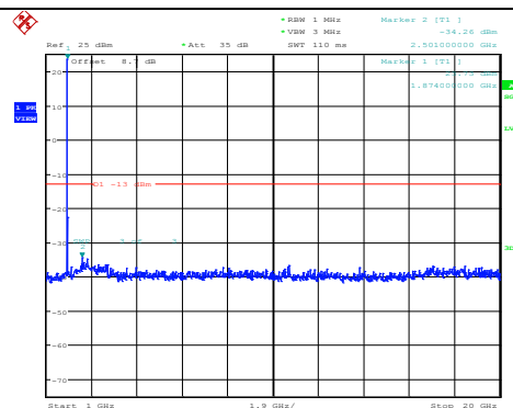
Band2-15MHz-QPSK-18900-1RB#0- Range2:1000~20000MHz
