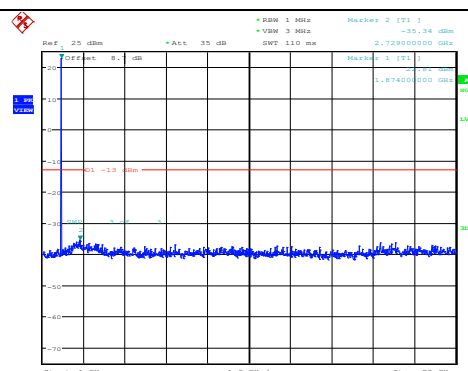
Band2-3MHz-16QAM-18900-1RB#0- Range2:1000~20000MHz
