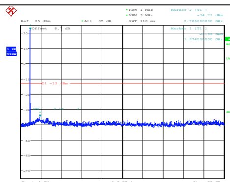
Band2-20MHz-64QAM-18900-1RB#0- Range2:1000~20000MHz
