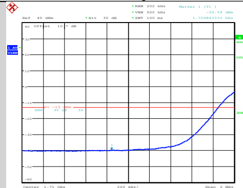
Band66-20MHz-64QAM-132072-1RB#0
