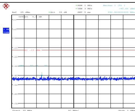
Band2-15MHz-QPSK-18675-1RB#0- Range1:30~1000MHz
