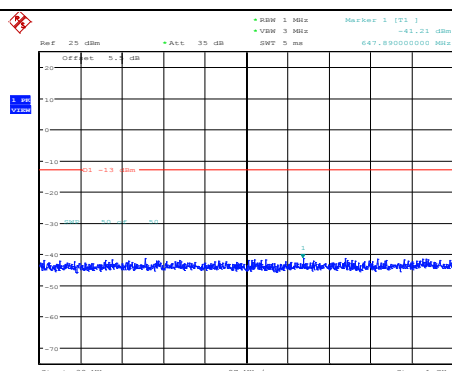
Band2-15MHz-16QAM-18675-1RB#0- Range1:30~1000MHz
