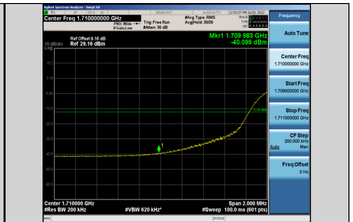
Band66-20MHz-QPSK-132072-100RB#0
