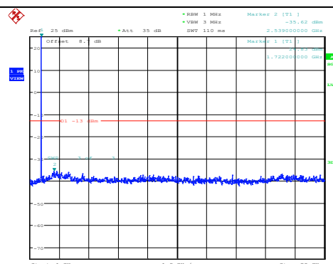
Band4-3MHz-16QAM-20175-1RB#0- Range2:1000~20000MHz
