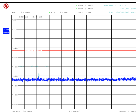
Band2-5MHz-QPSK-18625-1RB#0- Range1:30~1000MHz
