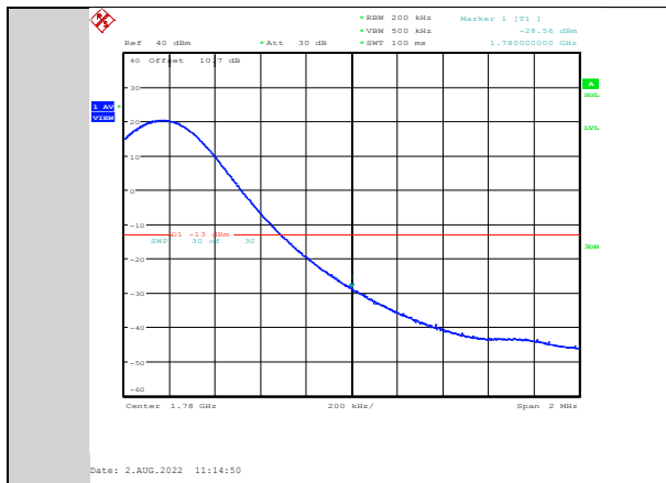
Band66-15MHz-64QAM-132597-1RB#74
