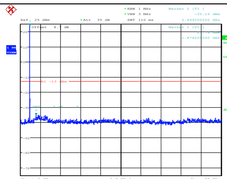
Band2-10MHz-QPSK-18900-1RB#0- Range2:1000~20000MHz
