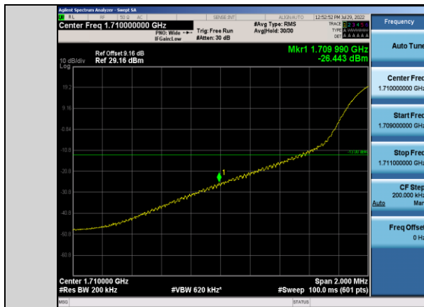
Band66-20MHz-16QAM-132072-1RB#0
