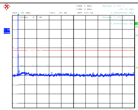
Band2-15MHz-16QAM-18900-1RB#0- Range2:1000~20000MHz
