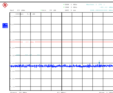
Band2-20MHz-16QAM-18700-1RB#0- Range1:30~1000MHz
