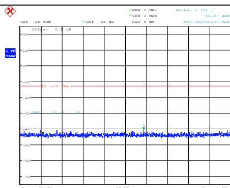
Band2-20MHz-64QAM-18700-1RB#0- Range1:30~1000MHz
