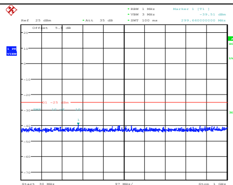
Band7-5MHz-QPSK-21100-1RB#0-Range1:30~1000MHz
