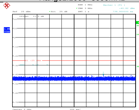
Band7-20MHz-64QAM-20850-1RB#0- Range2:1000~3000MHz
