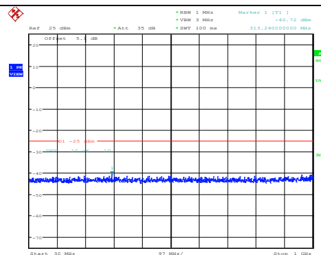
Band7-20MHz-64QAM-20850-1RB#0- Range1:30~1000MHz
