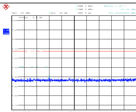
Band4-10MHz-64QAM-20000-1RB#0- Range1:30~1000MHz
