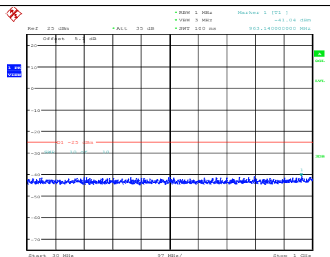
Band7-20MHz-64QAM-21100-1RB#0- Range1:30~1000MHz
