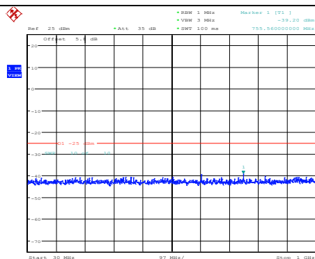
Band7-5MHz-QPSK-21425-1RB#0- Range1:30~1000MHz
