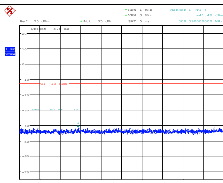
Band4-20MHz-16QAM-20050-1RB#0- Range1:30~1000MHz
