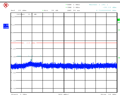
Band5-3MHz-16QAM-20525-1RB#0- Range2:1000~10000MHz
