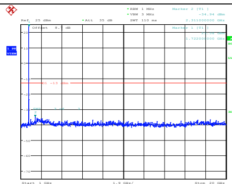
Band4-10MHz-16QAM-20175-1RB#0- Range2:1000~20000MHz
