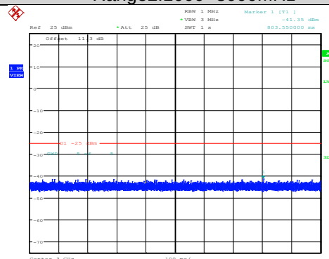
Band7-10MHz-64QAM-21400-1RB#0- Range2:1000~3000MHz
