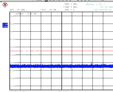
Band7-10MHz-64QAM-21100-1RB#0- Range2:1000~3000MHz
