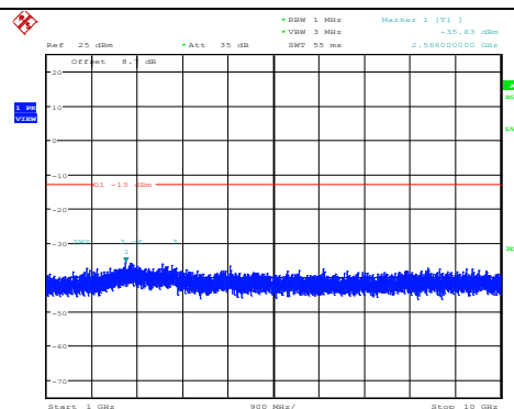
Band5-1.4MHz-QPSK-20525-1RB#0- Range2:1000~10000MHz
