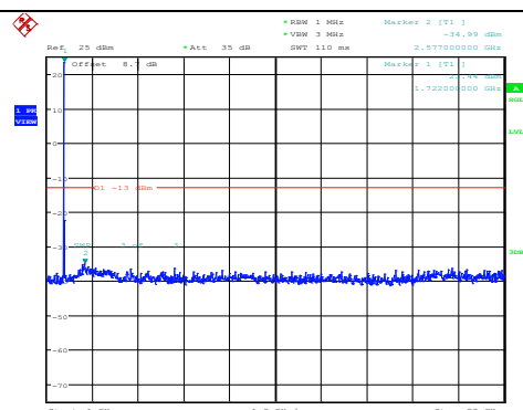
Band4-10MHz-64QAM-20175-1RB#0- Range2:1000~20000MHz
