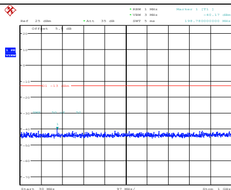
Band4-10MHz-16QAM-20000-1RB#0- Range1:30~1000MHz
