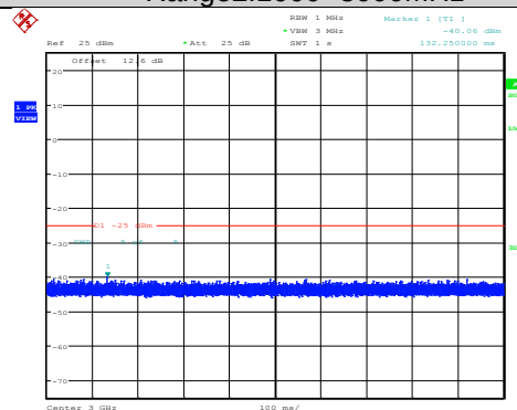
Band7-15MHz-16QAM-21375-1RB#0-Range2:1000~3000MHz
