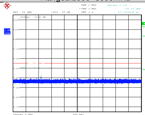
Band7-5MHz-16QAM-20775-1RB#0- Range2:1000~3000MHz
