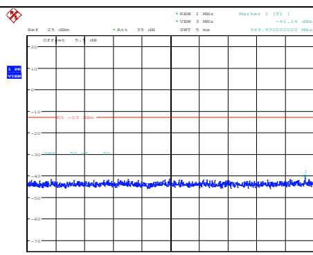
Band4-15MHz-QPSK-20025-1RB#0- Range1:30~1000MHz
