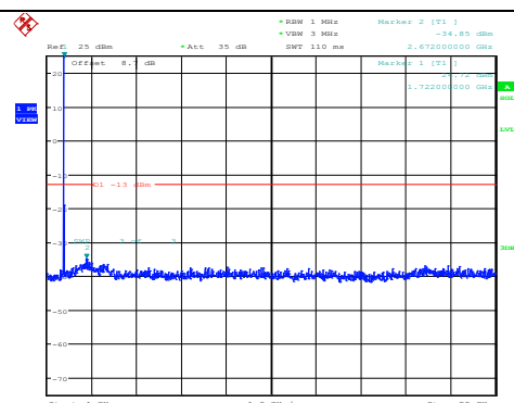
Band4-5MHz-16QAM-20175-1RB#0- Range2:1000~20000MHz
