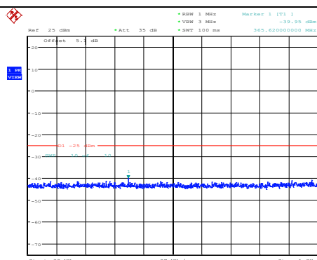
Band7-10MHz-64QAM-21100-1RB#0- Range1:30~1000MHz
