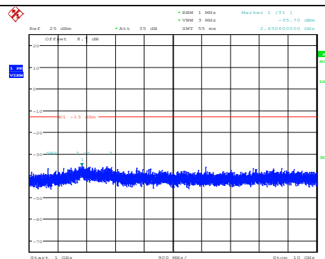
Band5-3MHz-64QAM-20525-1RB#0- Range2:1000~10000MHz
