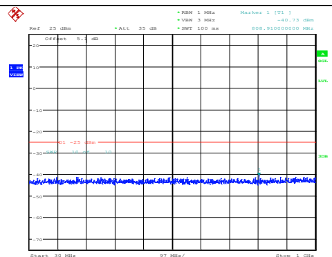
Band7-20MHz-64QAM-21350-1RB#0- Range1:30~1000MHz
