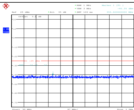
Band7-15MHz-QPSK-21375-1RB#0- Range1:30~1000MHz
