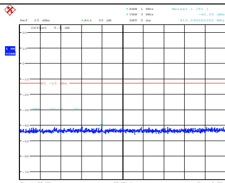
Band4-3MHz-64QAM-19965-1RB#0- Range1:30~1000MHz
