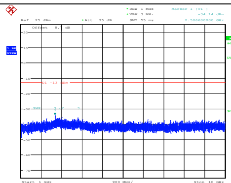
Band5-3MHz-QPSK-20525-1RB#0- Range2:1000~10000MHz
