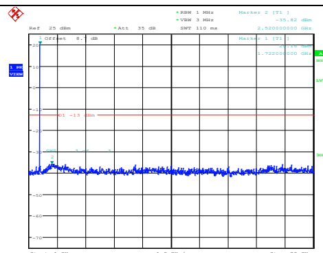
Band4-3MHz-64QAM-20175-1RB#0- Range2:1000~20000MHz
