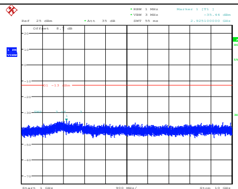
Band12-3MHz-64QAM-23095-1RB#0- Range2:1000~10000MHz
