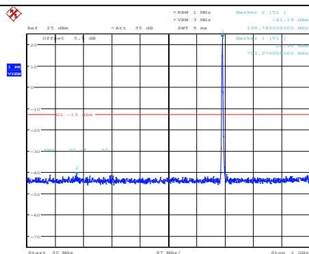
Band12-3MHz-16QAM-23025-1RB#0- Range1:30~1000MHz
