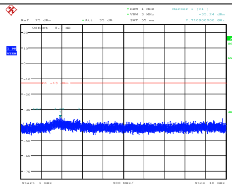
Band12-10MHz-QPSK-23095-1RB#0- Range2:1000~10000MHz
