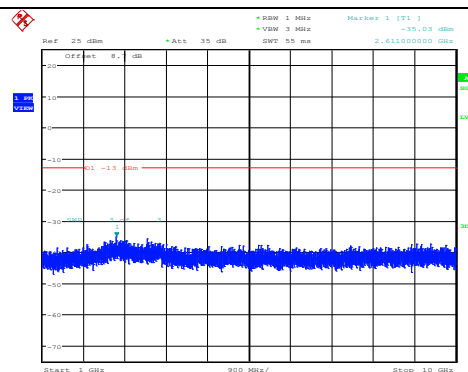
Band26-5MHz-16QAM-26740-1RB#0- Range2:1000~10000MHz
