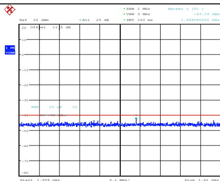
Band13-10MHz-16QAM-23230-1RB#0- Range5:1559~1610MHz
