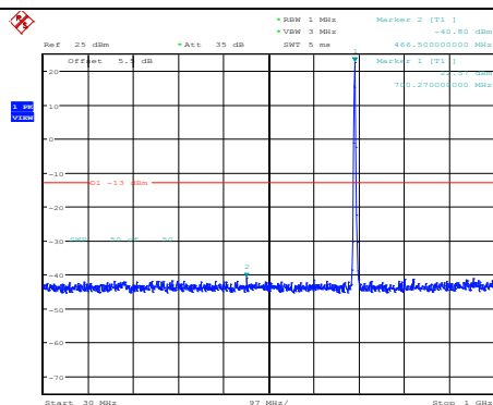
Band12-3MHz-64QAM-23025-1RB#0- Range1:30~1000MHz
