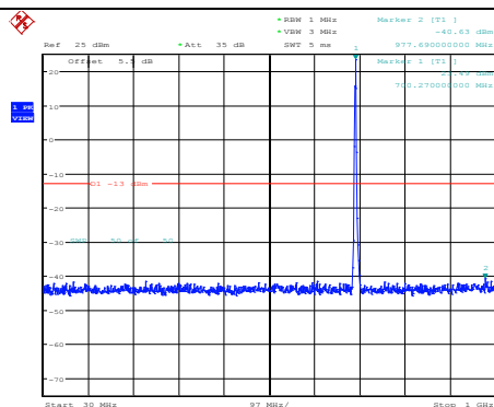
Band12-3MHz-QPSK-23025-1RB#0- Range1:30~1000MHz
