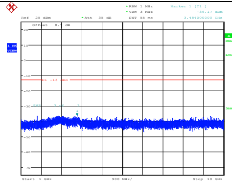
Band26-10MHz-16QAM-26740-1RB#0- Range2:1000~10000MHz
