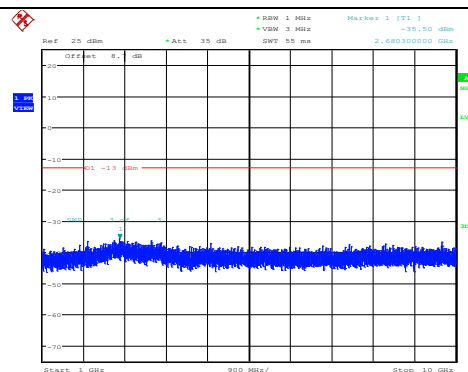
Band12-10MHz-16QAM-23095-1RB#0- Range2:1000~10000MHz
