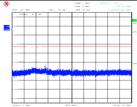
Band26-1.4MHz-QPSK-26740-1RB#0- Range2:1000~10000MHz
