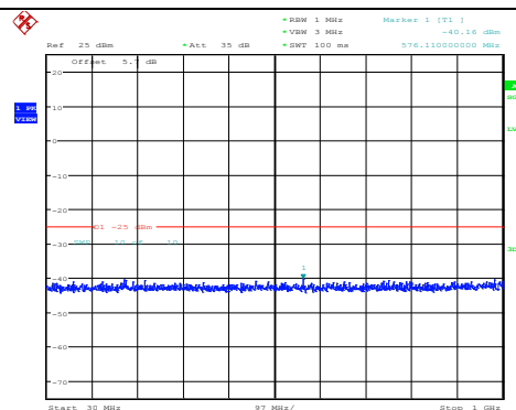
Band38-5MHz-QPSK-38000-1RB#0-Range1:30~1000MHz
