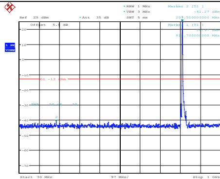
Band26-10MHz-QPSK-26740-1RB#0- Range1:30~1000MHz
