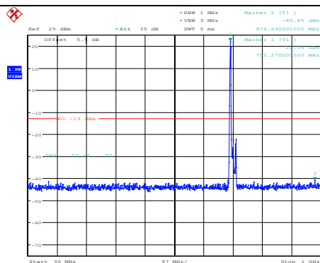
Band12-10MHz-16QAM-23060-1RB#0- Range1:30~1000MHz
