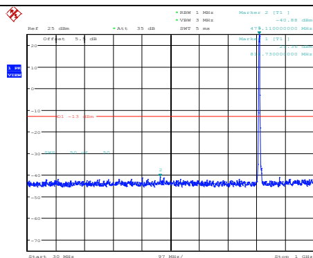
Band26-3MHz-QPSK-26705-1RB#0- Range1:30~1000MHz
