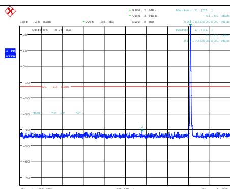
Band26-3MHz-16QAM-26705-1RB#0- Range1:30~1000MHz
