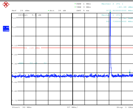
Band26-5MHz-64QAM-26715-1RB#0- Range1:30~1000MHz
