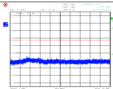
Band26-3MHz-QPSK-26740-1RB#0- Range2:1000~10000MHz
