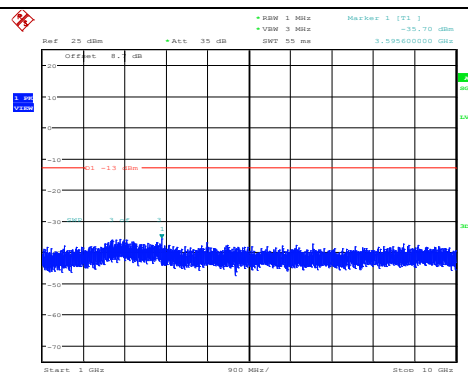
Band17-5MHz-QPSK-23790-1RB#0- Range2:1000~10000MHz
