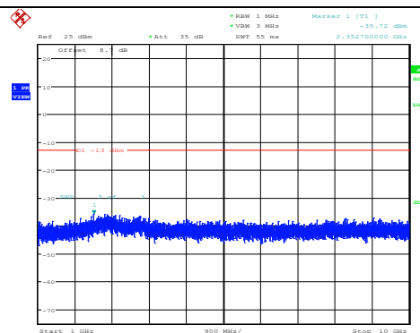
Band12-3MHz-QPSK-23095-1RB#0- Range2:1000~10000MHz
