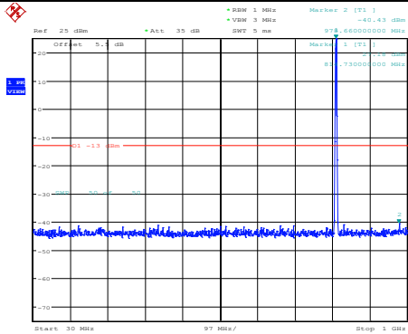
Band26-1.4MHz-QPSK-26697-1RB#0- Range1:30~1000MHz
