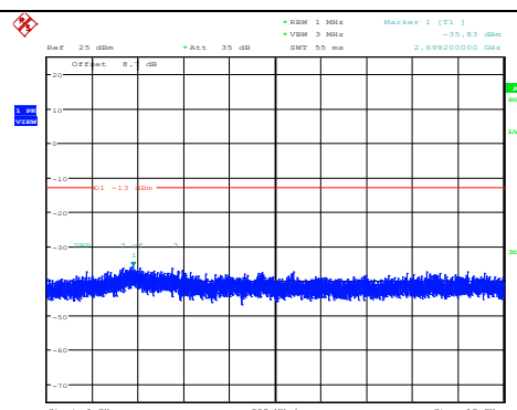
Band26-3MHz-16QAM-26740-1RB#0- Range2:1000~10000MHz
