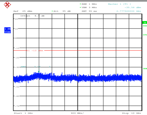
Band26-5MHz-64QAM-26740-1RB#0- Range2:1000~10000MHz
