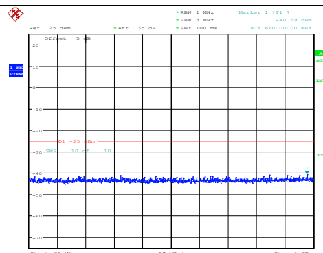
Band38-10MHz-64QAM-38200-1RB#0- Range1:30~1000MHz
