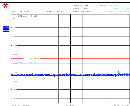
Band38-5MHz-64QAM-37775-1RB#0- Range1:30~1000MHz
