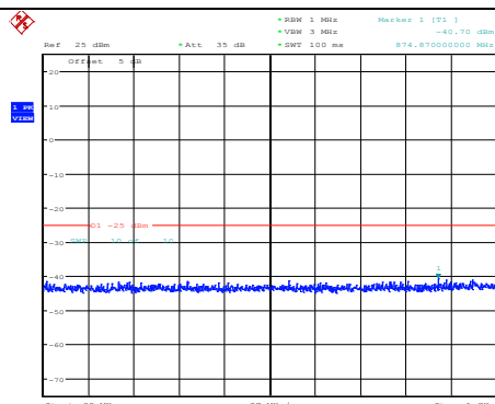
Band38-10MHz-64QAM-38000-1RB#0- Range1:30~1000MHz
