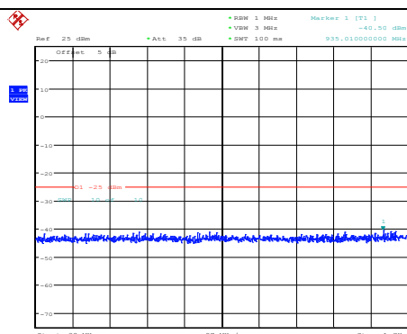
Band38-5MHz-64QAM-38225-1RB#0- Range1:30~1000MHz
