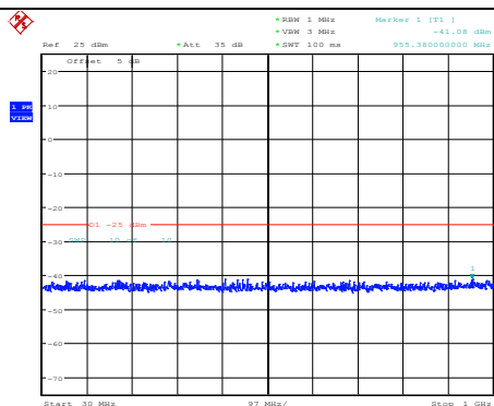
Band41-5MHz-64QAM-40065-1RB#0- Range1:30~1000MHz
