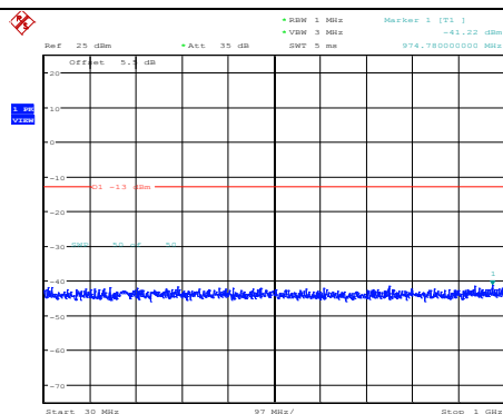
Band66-5MHz-QPSK-131997-1RB#0- Range1:30~1000MHz
