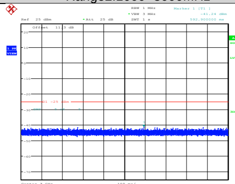
Band38-5MHz-64QAM-38000-1RB#0- Range2:1000~3000MHz
