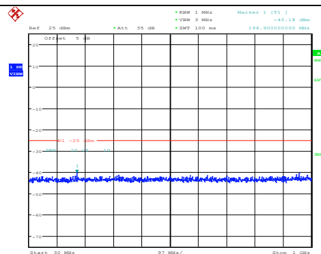
Band38-5MHz-64QAM-38000-1RB#0- Range1:30~1000MHz
