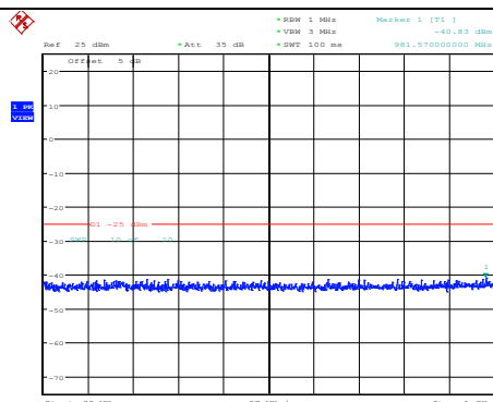
Band41-15MHz-64QAM-40115-1RB#0- Range1:30~1000MHz
