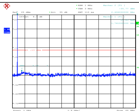
Band66-5MHz-QPSK-132322-1RB#0- Range2:1000~20000MHz
