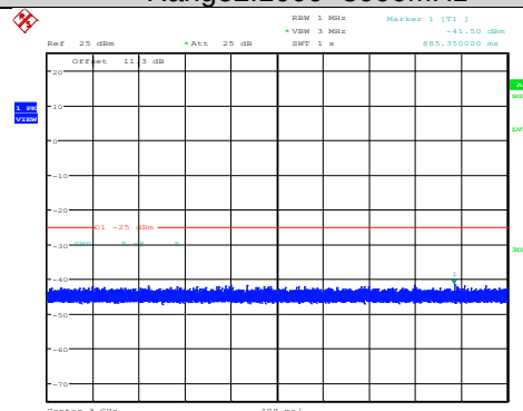
Band38-10MHz-64QAM-38200-1RB#0- Range2:1000~3000MHz
