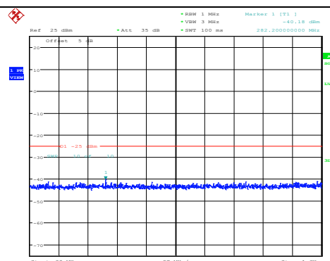
Band41-20MHz-64QAM-41140-1RB#0- Range1:30~1000MHz
