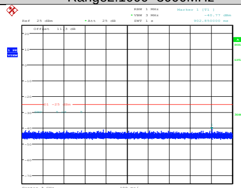
Band41-20MHz-64QAM-40140-1RB#0- Range2:1000~3000MHz
