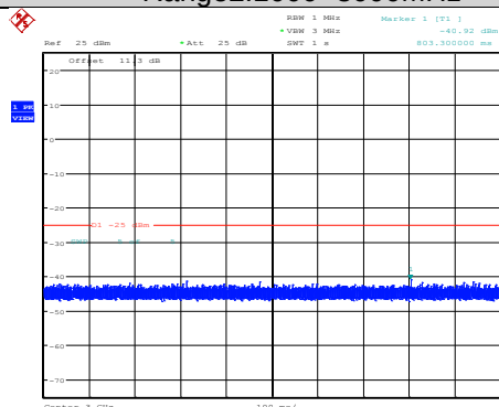
Band41-15MHz-64QAM-40115-1RB#0- Range2:1000~3000MHz
