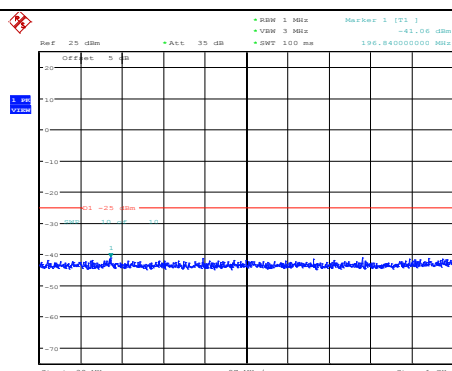
Band41-20MHz-64QAM-40590-1RB#0- Range1:30~1000MHz
