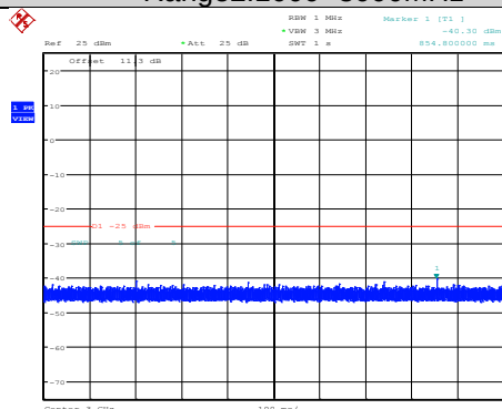
Band38-10MHz-64QAM-38000-1RB#0- Range2:1000~3000MHz
