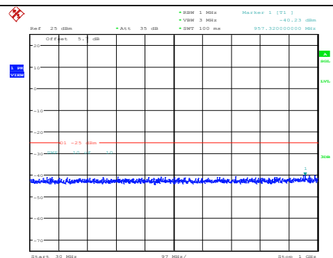
Band38-10MHz-QPSK-38200-1RB#0-Range1:30~1000MHz
