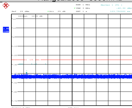
Band41-15MHz-QPSK-40115-1RB#0-Range2:1000~3000MHz
