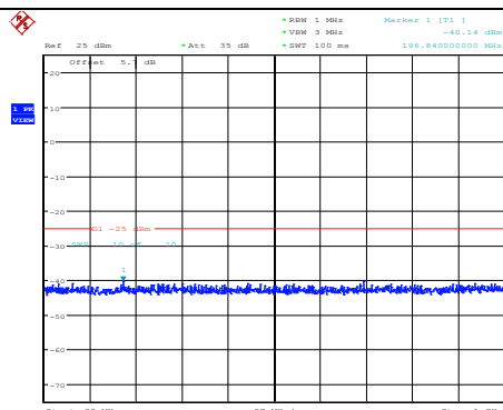
Band41-20MHz-QPSK-40590-1RB#0-Range1:30~1000MHz
