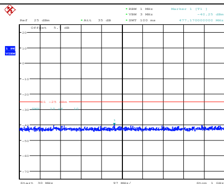
Band38-10MHz-16QAM-38200-1RB#0- Range1:30~1000MHz
