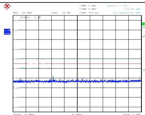
Band38-10MHz-64QAM-37800-1RB#0- Range1:30~1000MHz
