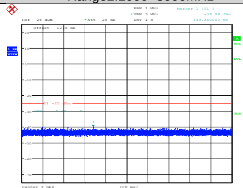
Band38-10MHz-QPSK-38200-1RB#0-Range2:1000~3000MHz
