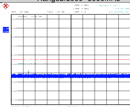
Band41-20MHz-16QAM-41140-1RB#0- Range2:1000~3000MHz
