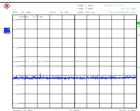
Band38-20MHz-QPSK-38150-1RB#0- Range1:30~1000MHz
