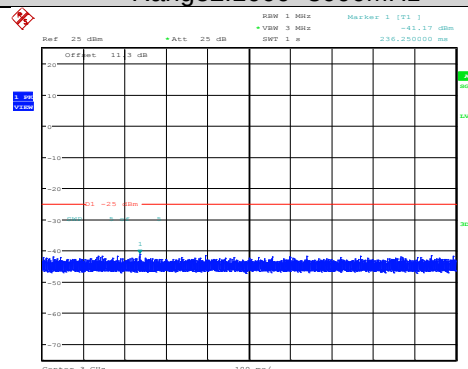
Band41-20MHz-64QAM-41140-1RB#0- Range2:1000~3000MHz
