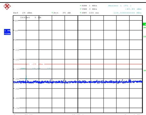
Band41-15MHz-64QAM-40590-1RB#0- Range1:30~1000MHz
