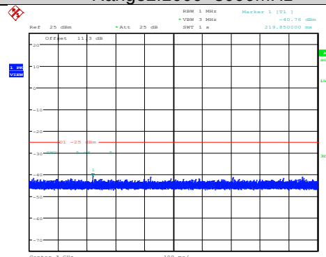
Band41-15MHz-64QAM-40590-1RB#0- Range2:1000~3000MHz
