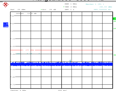
Band38-15MHz-QPSK-38000-1RB#0- Range2:1000~3000MHz
