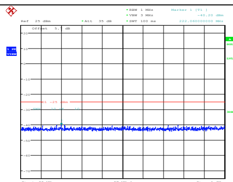
Band38-10MHz-QPSK-37800-1RB#0- Range1:30~1000MHz
