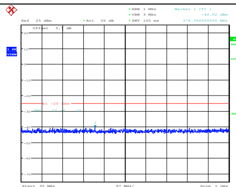
Band38-15MHz-QPSK-38000-1RB#0- Range1:30~1000MHz
