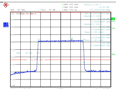
Band4-20MHz-64QAM-20050-100RB#0
