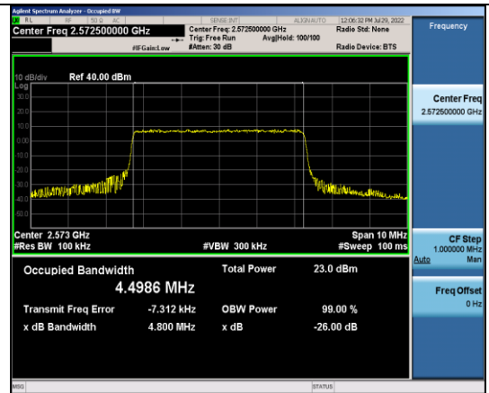
Band38-5MHz-16QAM-37775-25RB#0
