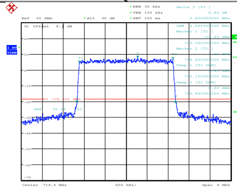
Band12-3MHz-QPSK-23095-15RB#0
