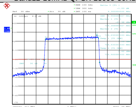
Band12-10MHz-QPSK-23095-50RB#0
