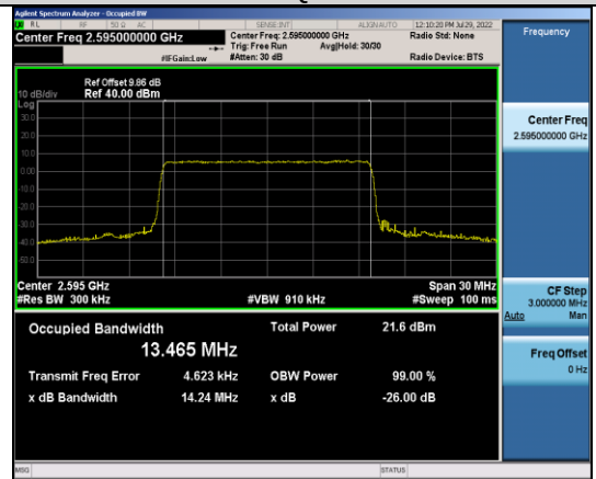
Band38-15MHz-16QAM-38000-75RB#0
