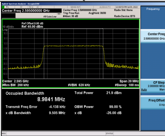
Band38-10MHz-16QAM-38000-50RB#0
