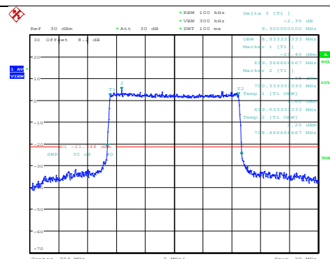
Band12-10MHz-QPSK-23060-50RB#0
