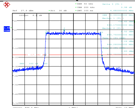
Band5-5MHz-16QAM-20525-25RB#0
