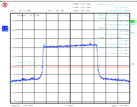
Band17-10MHz-16QAM-23780-50RB#0
