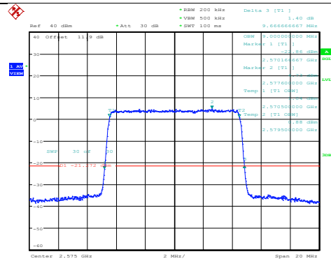
Band38-10MHz-64QAM-37800-50RB#0
