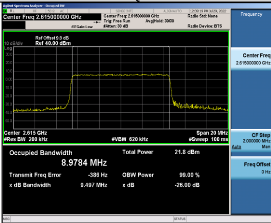
Band38-10MHz-16QAM-38200-50RB#0
