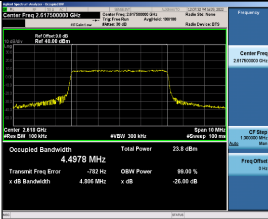
Band38-5MHz-QPSK-38225-25RB#0
