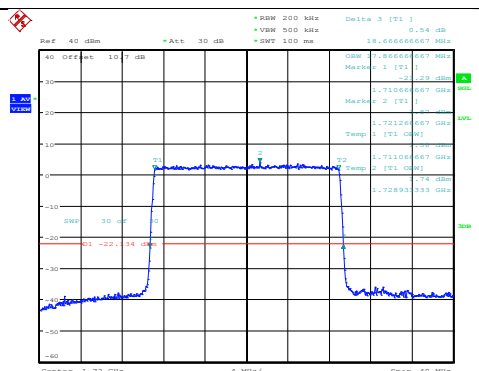
Band4-20MHz-16QAM-20050-100RB#0
