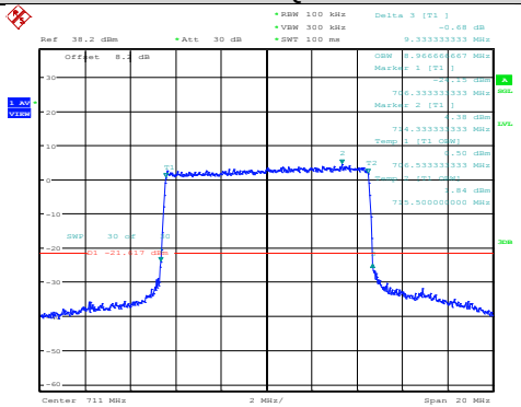
Band17-10MHz-16QAM-23790-50RB#0
