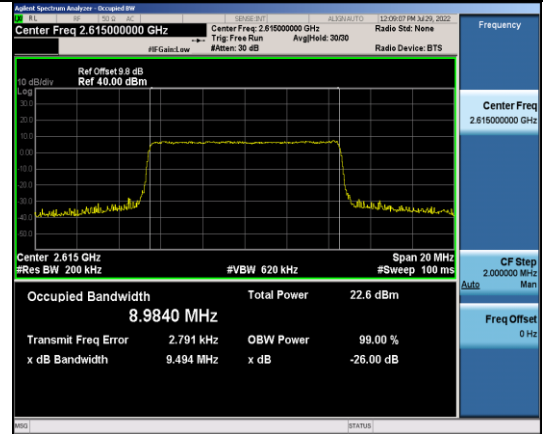
Band38-10MHz-QPSK-38200-50RB#0
