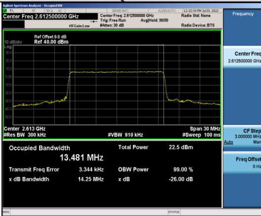
Band38-15MHz-QPSK-38175-75RB#0
