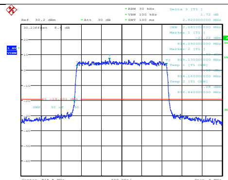
Band26-3MHz-64QAM-26705-15RB#0
