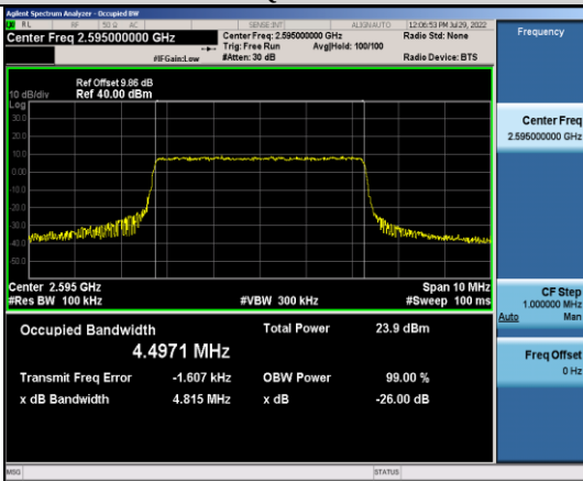
Band38-5MHz-QPSK-38000-25RB#0
