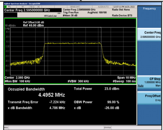
Band38-5MHz-16QAM-38000-25RB#0
