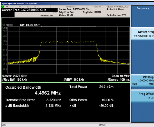
Band38-5MHz-QPSK-37775-25RB#0
