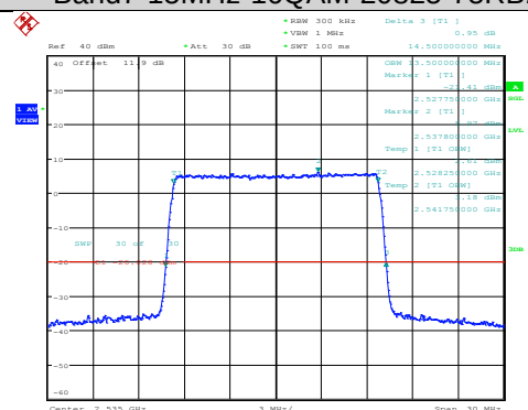
Band7-15MHz-16QAM-20825-75RB#0
