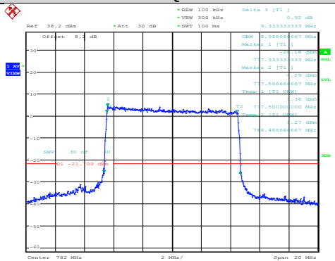
Band13-10MHz-QPSK-23230-50RB#0
