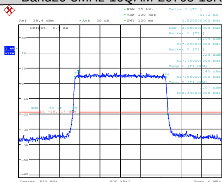
Band26-3MHz-16QAM-26705-15RB#0
