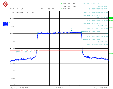
Band17-10MHz-64QAM-23780-50RB#0
