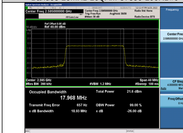
Band38-20MHz-16QAM-38000-100RB#0
