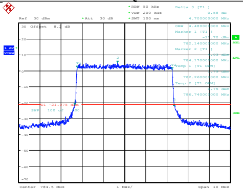
Band13-5MHz-64QAM-23230-25RB#0
