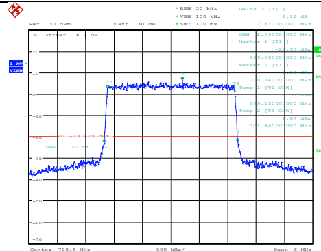
Band12-3MHz-QPSK-23025-15RB#0
