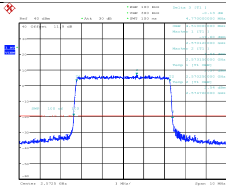
Band38-5MHz-64QAM-37775-25RB#0
