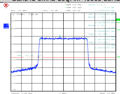
Band41-5MHz-16QAM-40065-25RB#0
