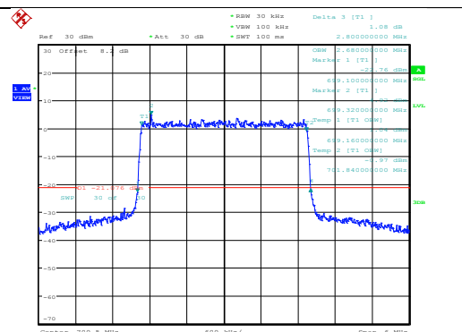
Band12-3MHz-64QAM-23025-15RB#0
