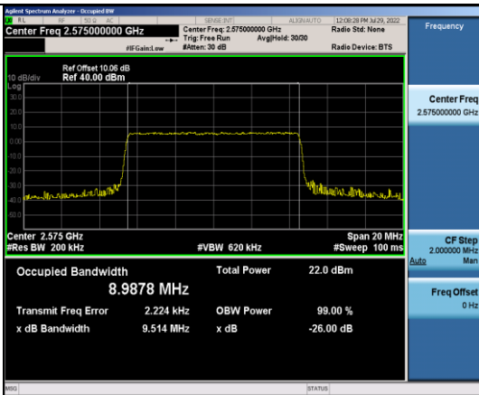
Band38-10MHz-16QAM-37800-50RB#0
