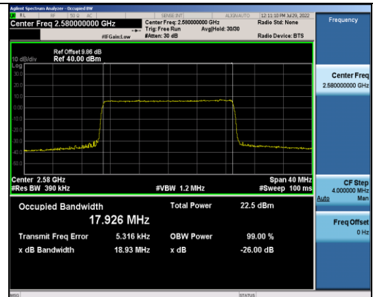
Band38-20MHz-QPSK-37850-100RB#0
