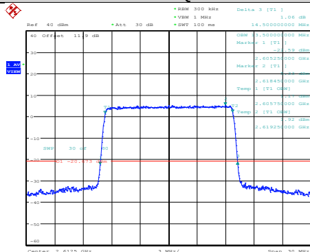
Band38-15MHz-64QAM-38000-75RB#0
