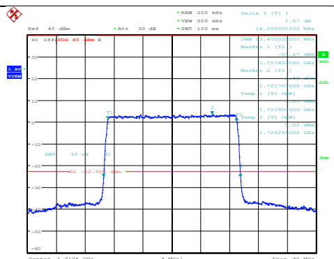
Band4-15MHz-64QAM-20025-75RB#0
