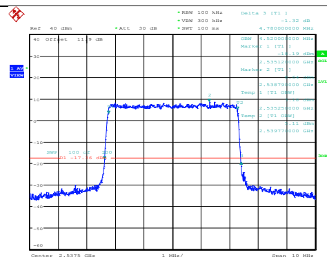
Band41-5MHz-16QAM-40065-25RB#0
