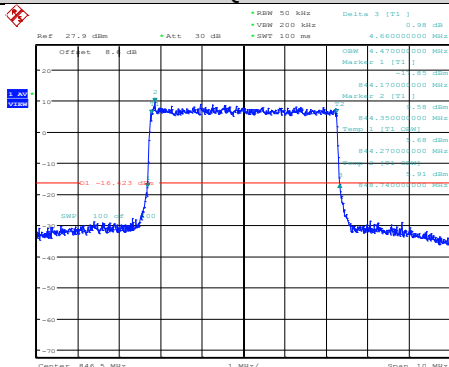
Band5-5MHz-QPSK-20525-25RB#0
