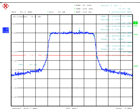
Band26-1.4MHz-64QAM-26697-6RB#0
