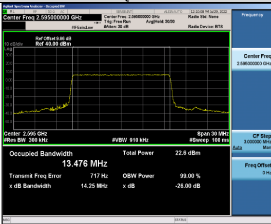
Band38-15MHz-QPSK-38000-75RB#0
