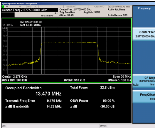
Band38-15MHz-QPSK-37825-75RB#0
