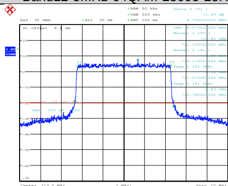
Band12-5MHz-64QAM-23095-25RB#0
