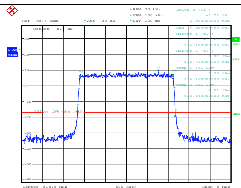
Band26-3MHz-QPSK-26705-15RB#0
