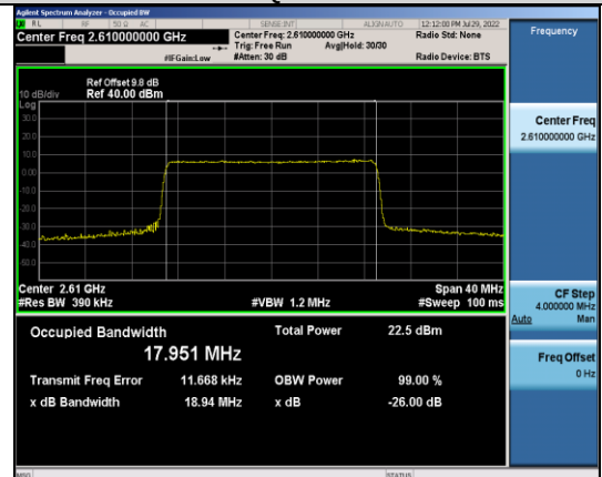
Band38-20MHz-QPSK-38150-100RB#0
