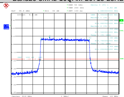
Band26-5MHz-16QAM-26715-25RB#0
