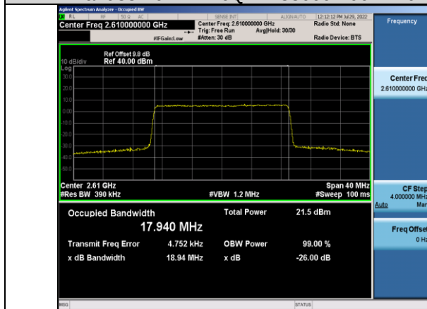
Band38-20MHz-16QAM-38150-100RB#0
