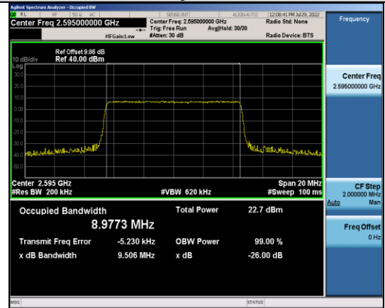
Band38-10MHz-QPSK-38000-50RB#0
