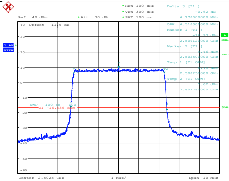
Band7-5MHz-QPSK-20775-25RB#0
