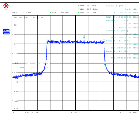
Band12-5MHz-64QAM-23035-25RB#0
