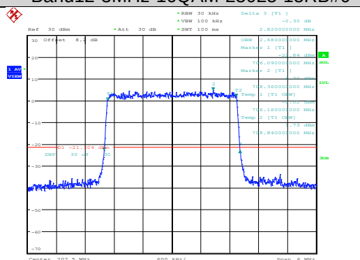
Band12-3MHz-16QAM-23025-15RB#0
