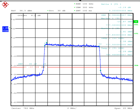
Band13-10MHz-16QAM-23230-50RB#0
