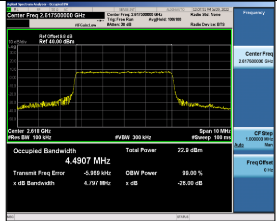
Band38-5MHz-16QAM-38225-25RB#0
