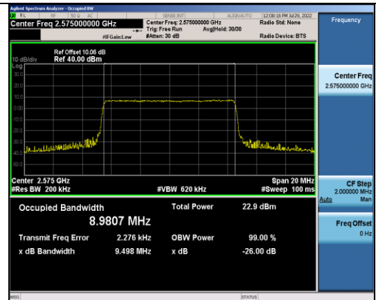
Band38-10MHz-QPSK-37800-50RB#0
