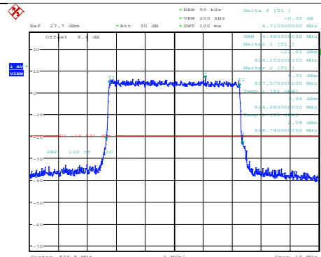
Band5-5MHz-16QAM-20425-25RB#0
