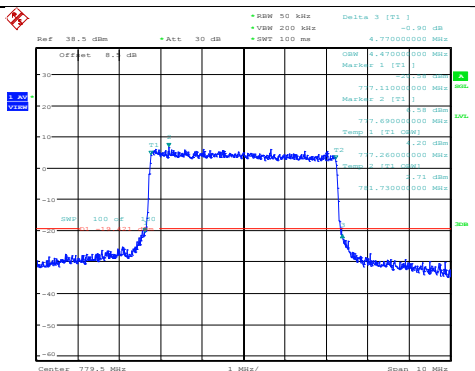
Band13-5MHz-64QAM-23205-25RB#0
