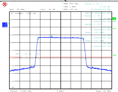
Band41-20MHz-16QAM-40590-100RB#0
