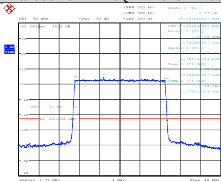
Band66-20MHz-16QAM-132322-100RB#0
