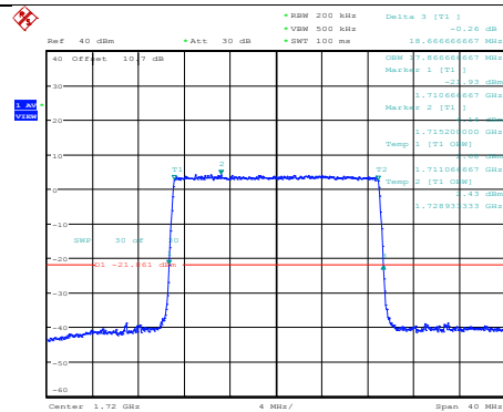
Band66-20MHz-QPSK-132072-100RB#0
