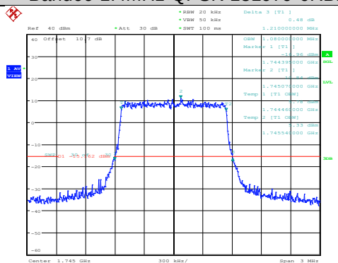
Band66-1.4MHz-QPSK-131979-6RB#0
