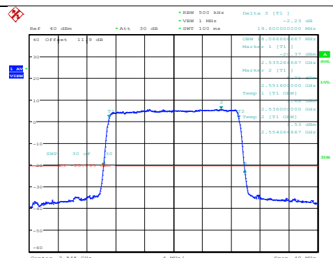
Band41-20MHz-64QAM-40140-100RB#0
