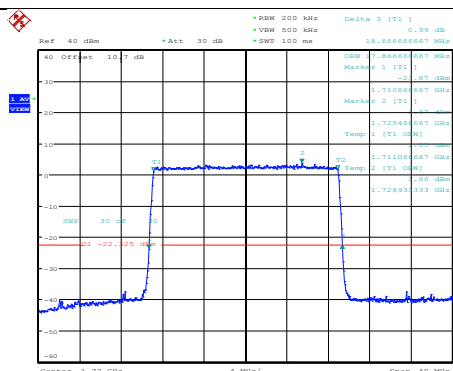
Band66-20MHz-16QAM-132072-100RB#0
