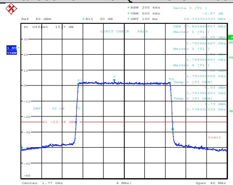
Band66-20MHz-64QAM-132322-100RB#0
