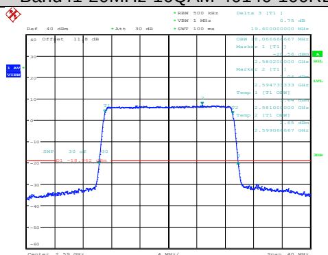
Band41-20MHz-16QAM-40140-100RB#0
