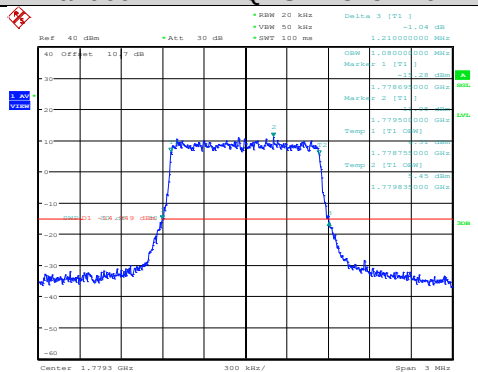
Band66-1.4MHz-QPSK-132322-6RB#0
