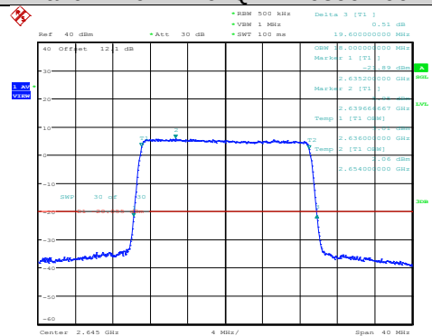
Band41-20MHz-64QAM-40590-100RB#0
