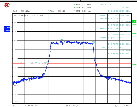
Band66-1.4MHz-16QAM-132322-6RB#0
