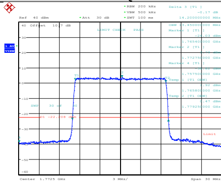
Band66-15MHz-64QAM-132322-75RB#0
