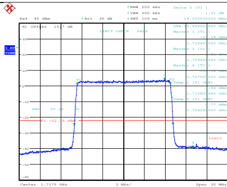
Band66-15MHz-64QAM-132047-75RB#0
