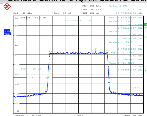
Band66-20MHz-64QAM-132072-100RB#0
