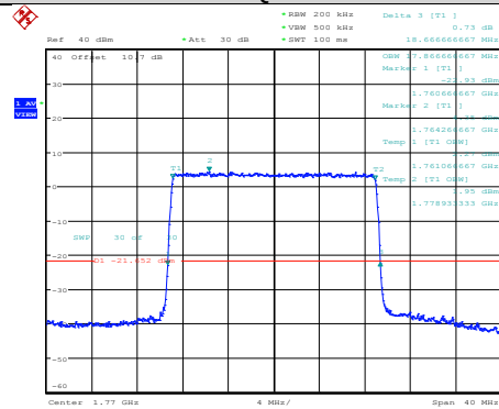
Band66-20MHz-QPSK-132322-100RB#0
