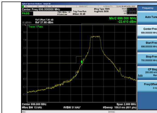
Band12-1.4MHz-QPSK-23017-1RB#0
