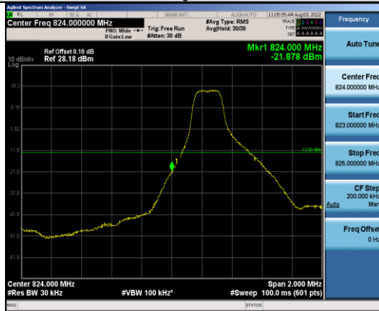
Band5-3MHz-64QAM-20415-1RB#0
