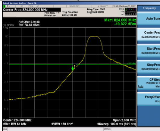
Band5-5MHz-64QAM-20425-1RB#0
