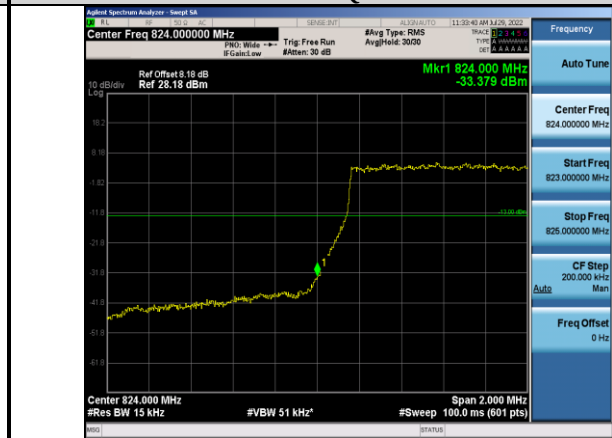
Band5-1.4MHz-16QAM-20407-6RB#0
