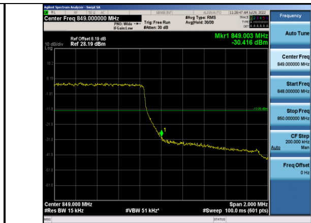
Band5-1.4MHz-QPSK-20643-6RB#0
