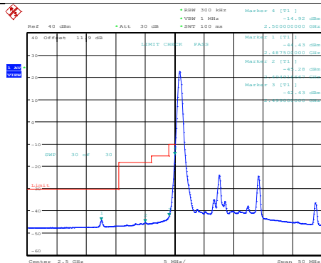
Band7-15MHz-QPSK-20825-1RB#0
