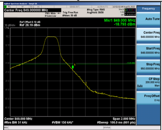
Band5-5MHz-64QAM-20625-1RB#24
