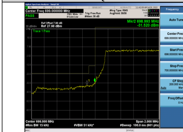
Band12-1.4MHz-QPSK-23017-6RB#0
