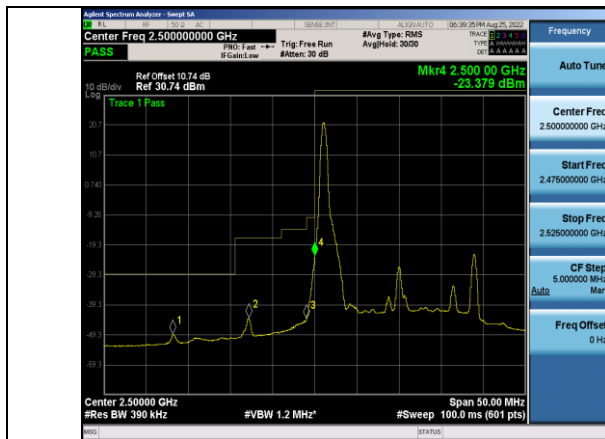
Band7-20MHz-QPSK-20850-1RB#0
