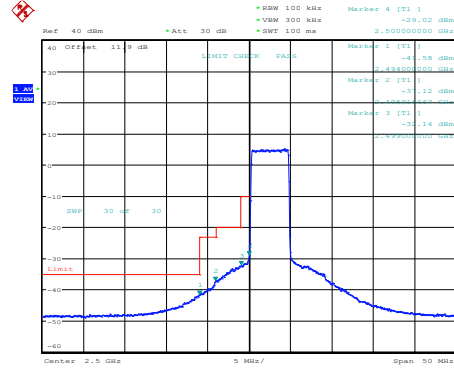
Band7-5MHz-16QAM-20775-1RB#0
