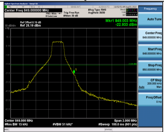
Band5-1.4MHz-64QAM-20643-1RB#5
