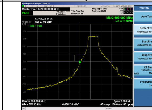
Band12-1.4MHz-16QAM-23017-1RB#0
