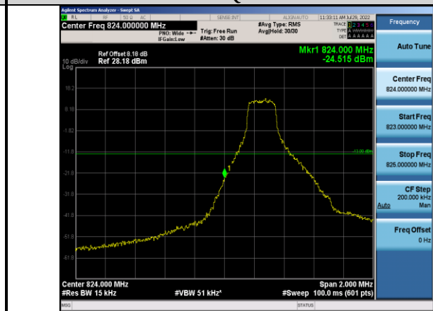
Band5-1.4MHz-16QAM-20407-1RB#0
