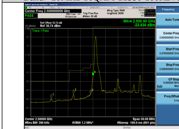
Band7-20MHz-64QAM-20850-1RB#0
