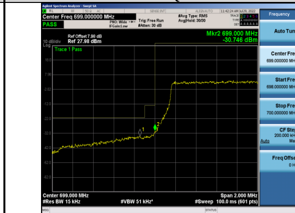
Band12-1.4MHz-16QAM-23017-6RB#0
