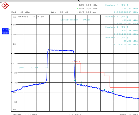
Band7-5MHz-16QAM-21425-1RB#24
