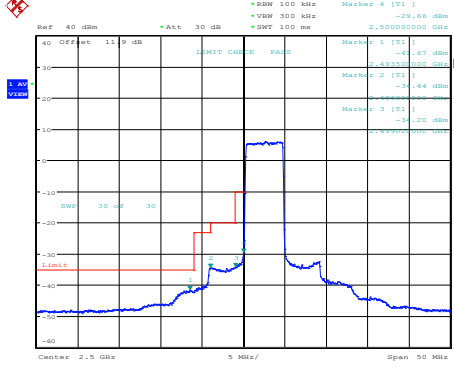
Band7-5MHz-QPSK-20775-1RB#0
