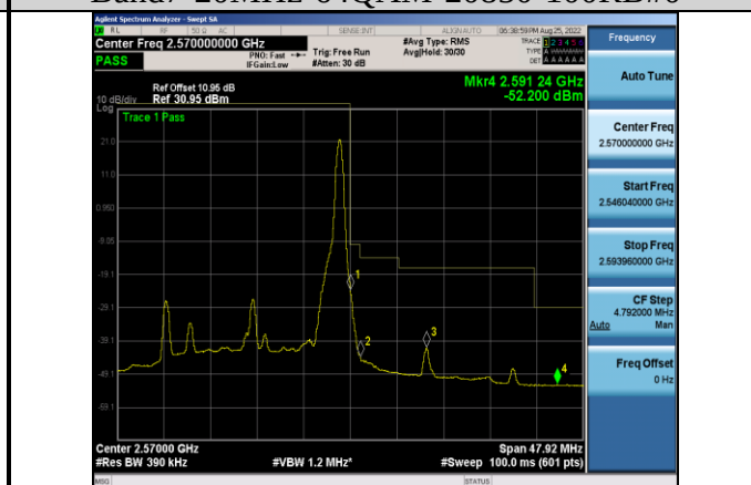
Band7-20MHz-64QAM-21350-1RB#99
