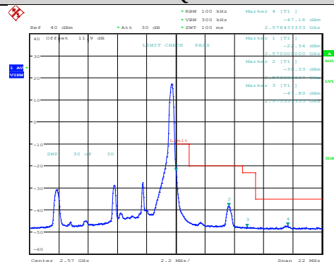
Band7-5MHz-64QAM-20775-25RB#0
