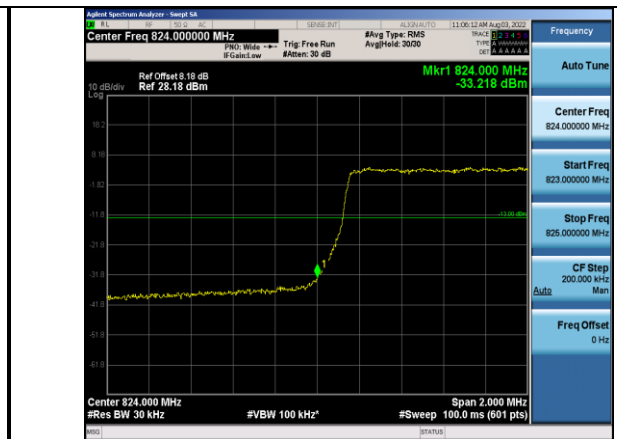
Band5-3MHz-64QAM-20415-15RB#0
