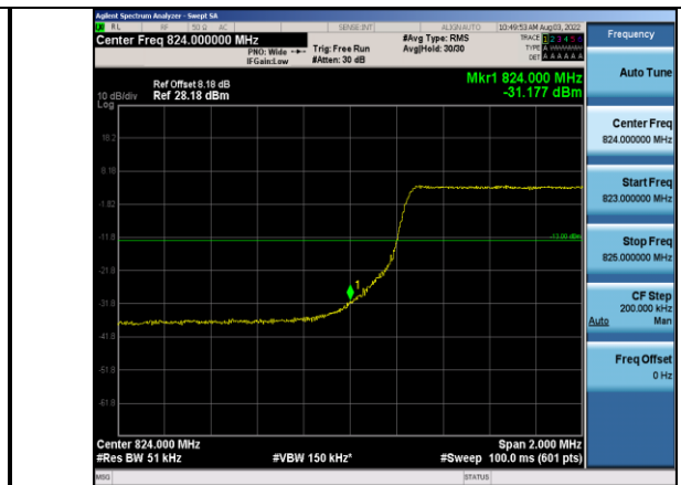
Band5-5MHz-64QAM-20425-25RB#0
