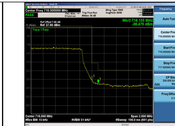
Band12-1.4MHz-QPSK-23173-6RB#0
