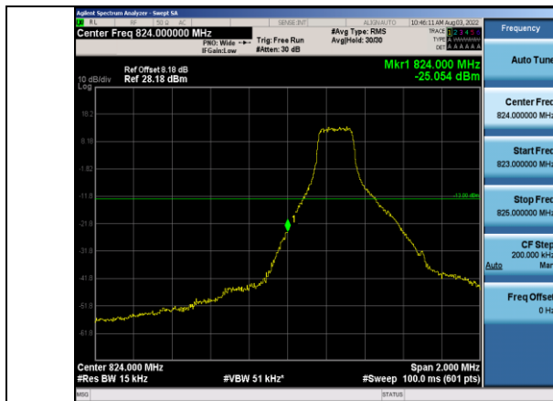
Band5-1.4MHz-QPSK-20407-1RB#0
