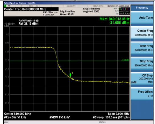
Band5-5MHz-64QAM-20625-25RB#0
