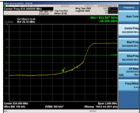
Band5-10MHz-64QAM-20450-50RB#0
