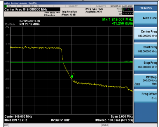
Band5-1.4MHz-64QAM-20643-6RB#0
