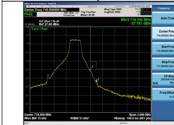
Band12-1.4MHz-QPSK-23173-1RB#5
