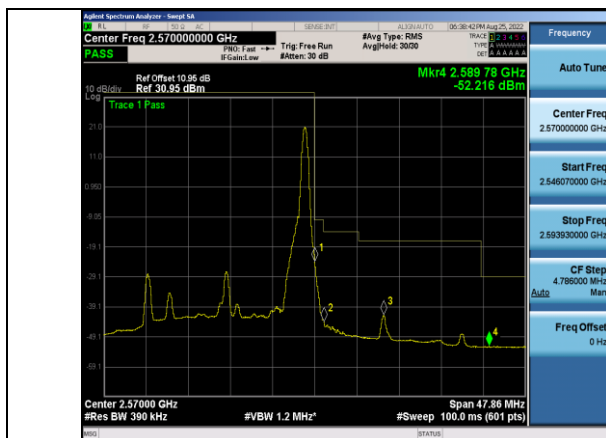
Band7-20MHz-16QAM-21350-1RB#99
