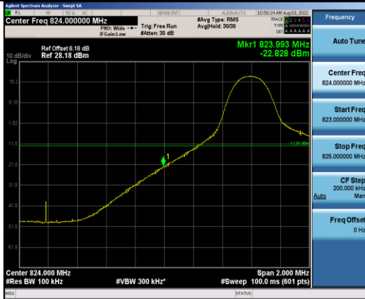
Band5-10MHz-64QAM-20450-1RB#0
