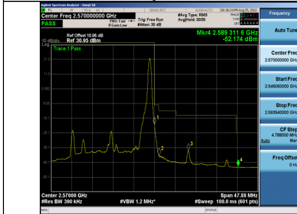
Band7-20MHz-QPSK-21350-1RB#99
