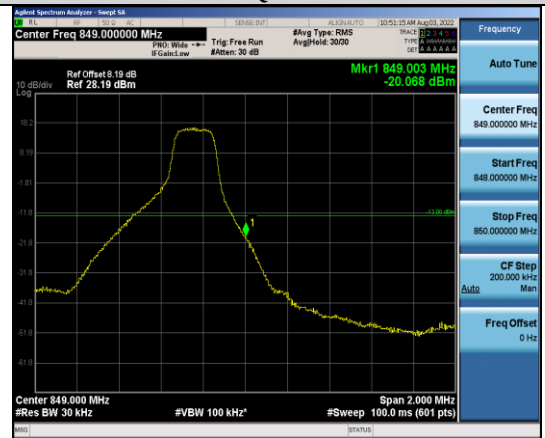
Band5-3MHz-64QAM-20635-1RB#14
