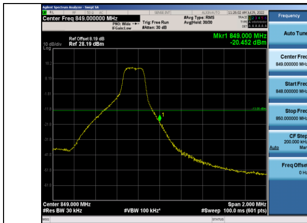
Band5-3MHz-16QAM-20635-1RB#14
