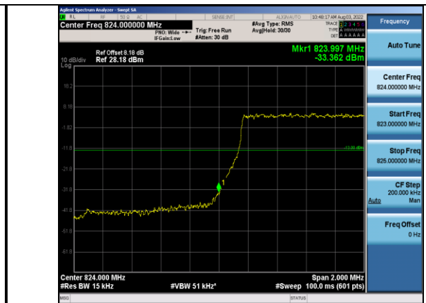
Band5-1.4MHz-64QAM-20407-6RB#0
