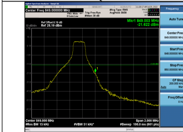
Band5-1.4MHz-QPSK-20643-1RB#5
