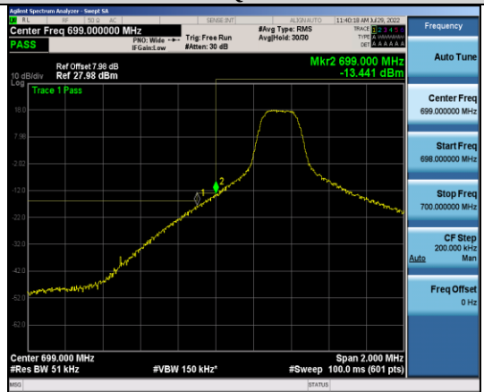
Band12-5MHz-QPSK-23035-1RB#0
