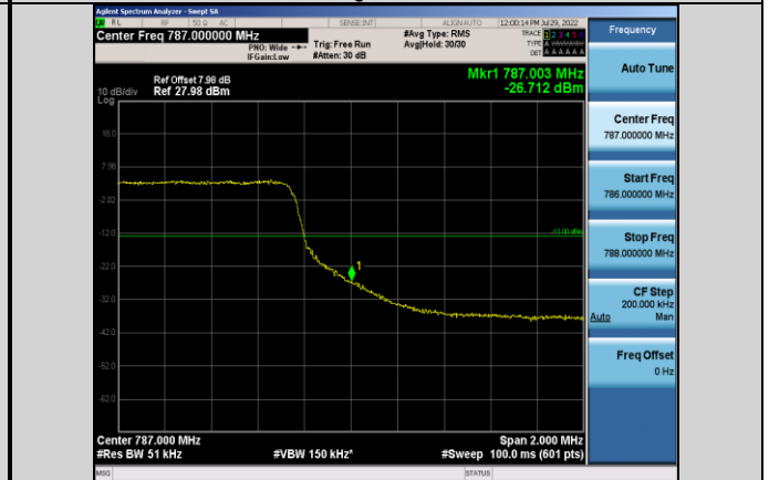
Band13-5MHz-QPSK-23255-25RB#0
