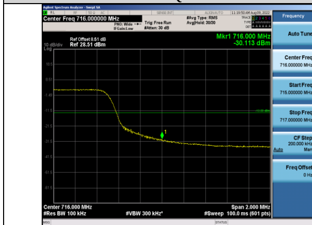
Band17-10MHz-64QAM-23800-50RB#0
