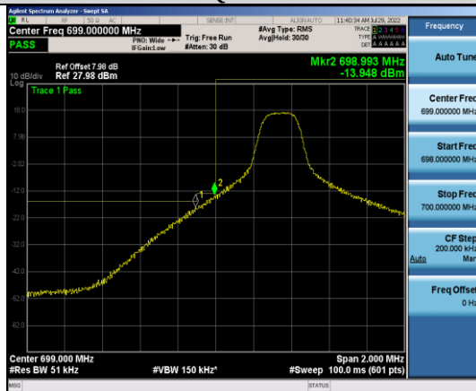
Band12-5MHz-16QAM-23035-1RB#0
