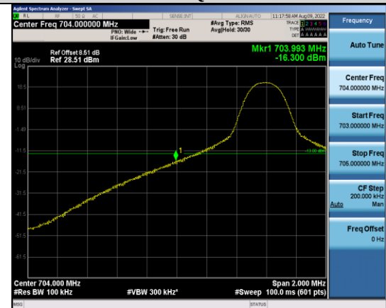
Band17-10MHz-64QAM-23780-1RB#0
