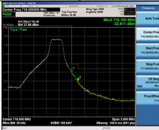
Band12-3MHz-16QAM-23165-1RB#14
