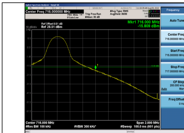
Band17-10MHz-64QAM-23800-1RB#49
