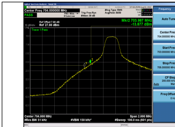
Band17-5MHz-16QAM-23755-1RB#0
