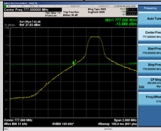
Band13-5MHz-QPSK-23205-1RB#0
