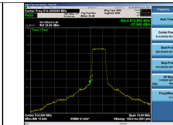
Band26-1.4MHz-QPSK-26697-6RB#0
