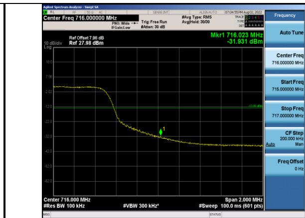
Band17-10MHz-16QAM-23800-50RB#0
