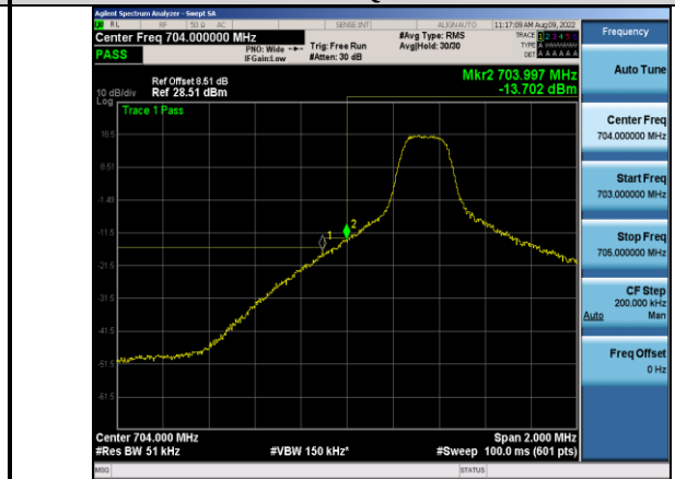
Band17-5MHz-64QAM-23755-1RB#0
