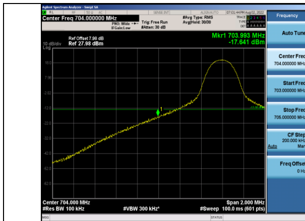
Band17-10MHz-16QAM-23780-1RB#0
