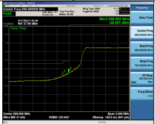
Band12-5MHz-QPSK-23035-25RB#0
