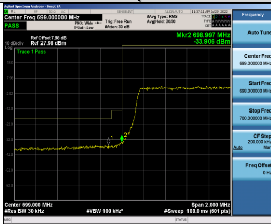
Band12-3MHz-16QAM-23025-15RB#0
