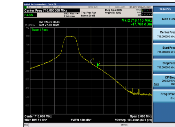
Band12-5MHz-QPSK-23155-1RB#24
