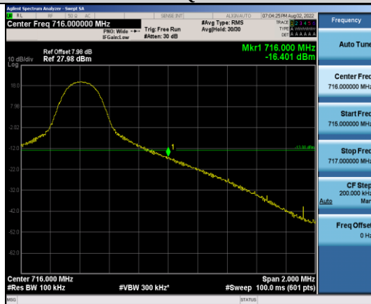
Band17-10MHz-16QAM-23800-1RB#49
