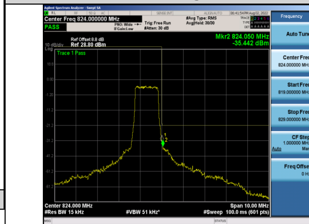
Band26-1.4MHz-QPSK-26783-6RB#0
