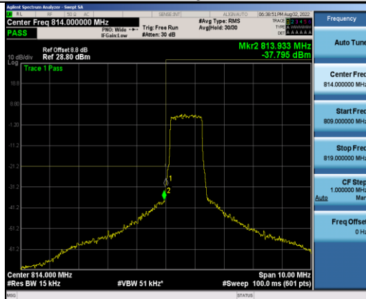
Band26-1.4MHz-16QAM-26697-6RB#0
