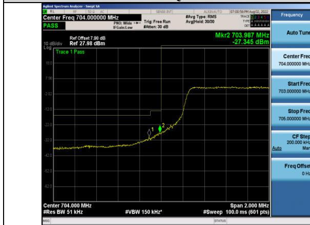
Band17-5MHz-16QAM-23755-25RB#0
