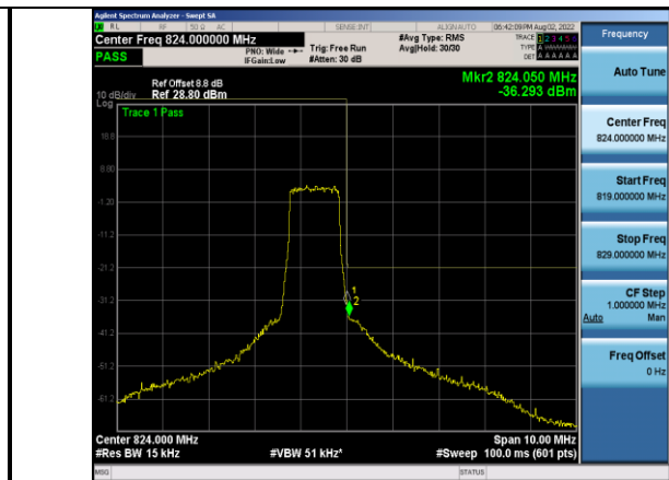
Band26-1.4MHz-16QAM-26783-6RB#0
