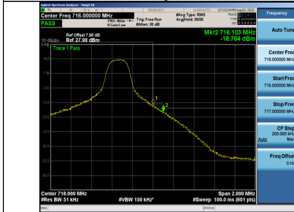
Band17-5MHz-16QAM-23825-1RB#24
