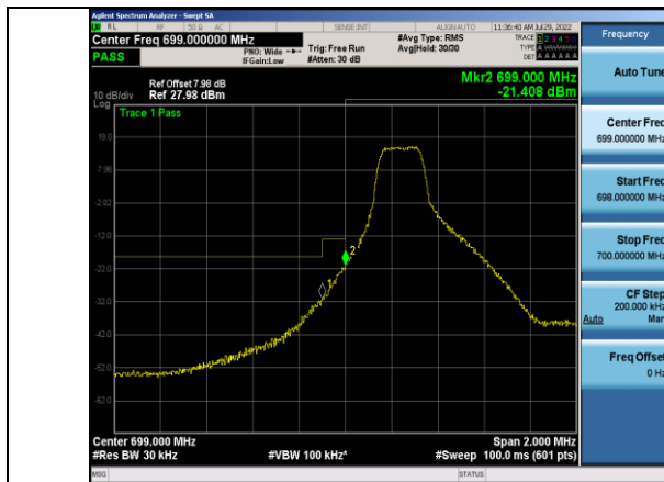
Band12-3MHz-16QAM-23025-1RB#0
