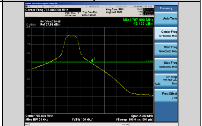
Band13-5MHz-QPSK-23255-1RB#24
