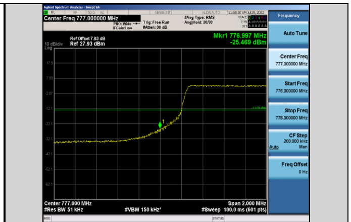
Band13-5MHz-QPSK-23205-25RB#0
