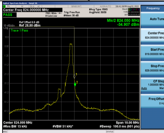
Band26-1.4MHz-16QAM-26783-1RB#5
