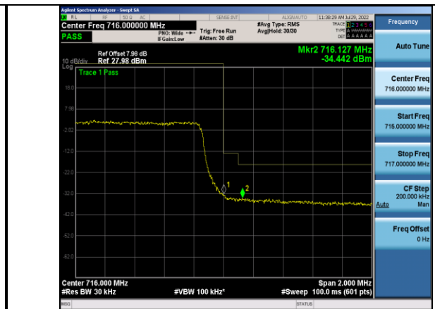
Band12-3MHz-16QAM-23165-15RB#0
