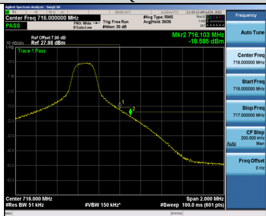
Band12-5MHz-16QAM-23155-1RB#24
