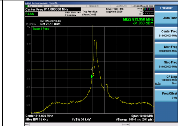
Band26-1.4MHz-64QAM-26697-1RB#0
