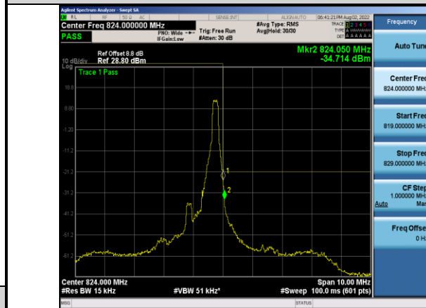
Band26-1.4MHz-QPSK-26783-1RB#5
