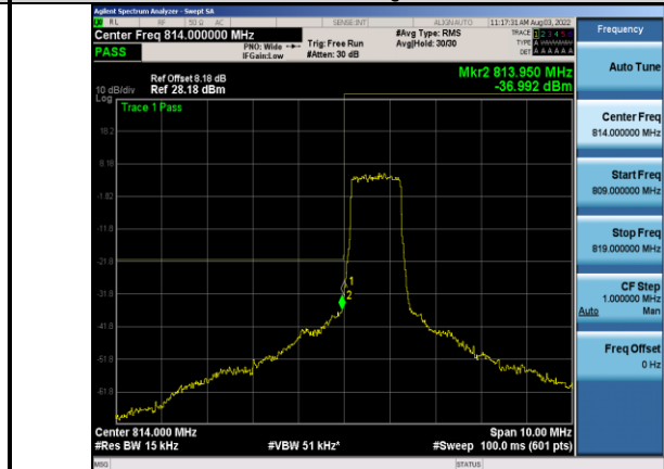
Band26-1.4MHz-64QAM-26697-6RB#0
