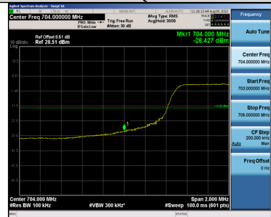
Band17-10MHz-64QAM-23780-50RB#0
