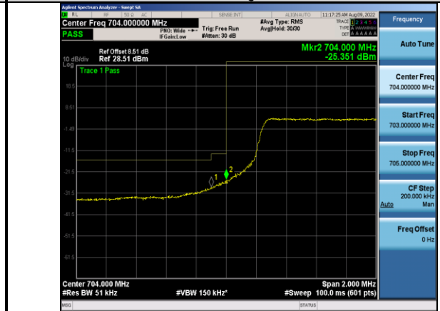
Band17-5MHz-64QAM-23755-25RB#0
