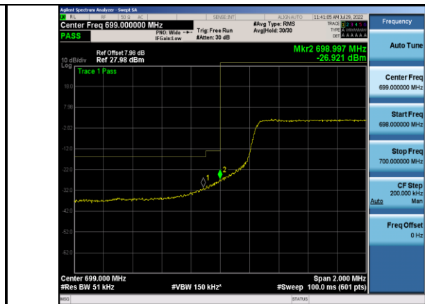
Band12-5MHz-16QAM-23035-25RB#0
