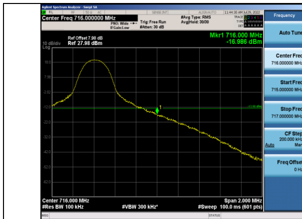
Band12-10MHz-16QAM-23130-1RB#49
