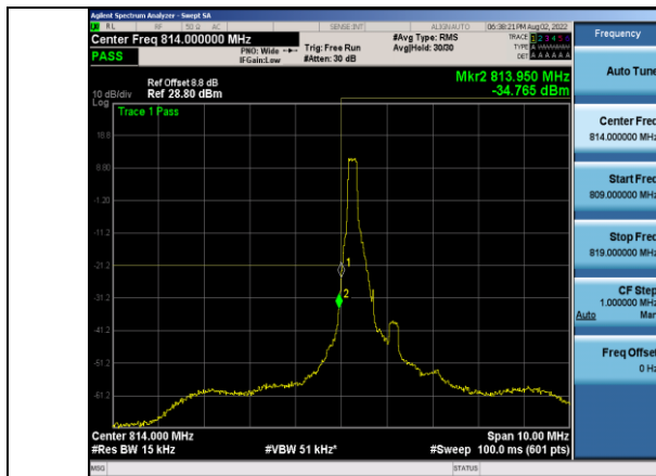
Band26-1.4MHz-16QAM-26697-1RB#0
