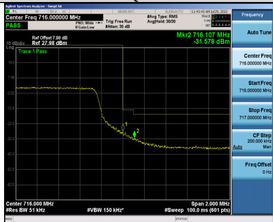
Band12-5MHz-16QAM-23155-25RB#0
