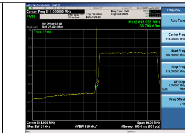
Band26-5MHz-QPSK-26715-25RB#0
