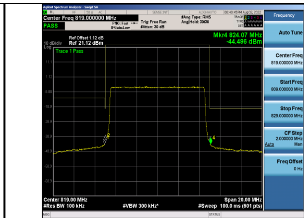
Band26-10MHz-16QAM-26740_Right-50RB#0
