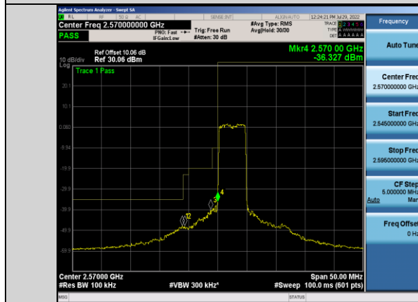
Band38-5MHz-16QAM-37775-25RB#0
