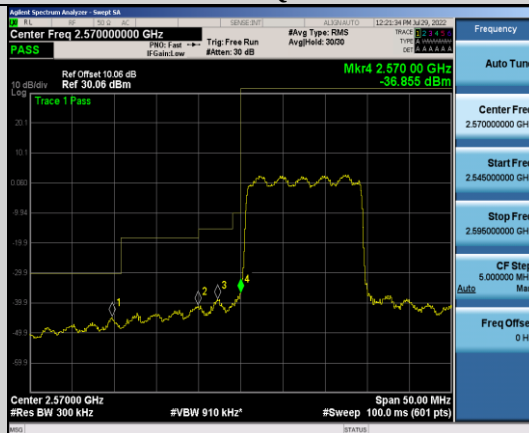
Band38-15MHz-16QAM-37825-75RB#0
