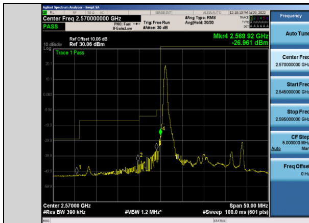
Band38-20MHz-16QAM-37850-1RB#0
