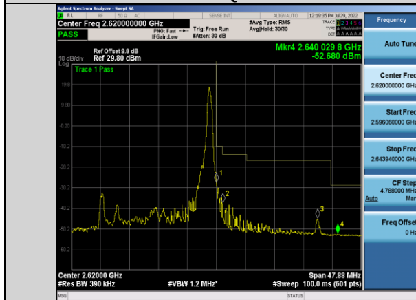
Band38-20MHz-16QAM-38150-1RB#99
