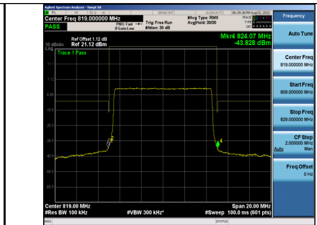
Band26-10MHz-QPSK-26740_Left-50RB#0
