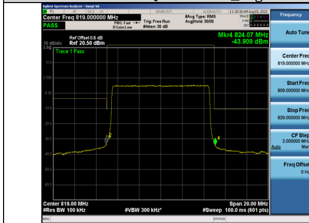
Band26-10MHz-64QAM-26740_Right-50RB#0
