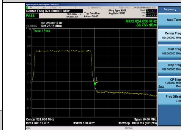
Band26-5MHz-QPSK-26765-25RB#0
