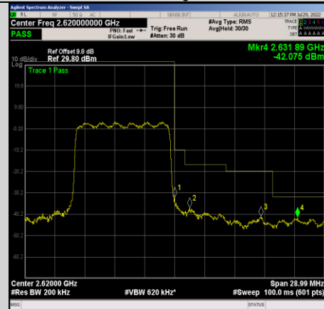
Band38-10MHz-QPSK-38200-50RB#0
