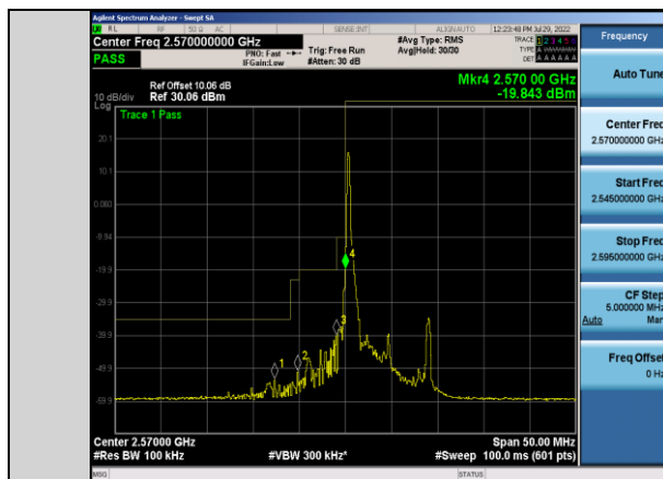
Band38-5MHz-16QAM-37775-1RB#0
