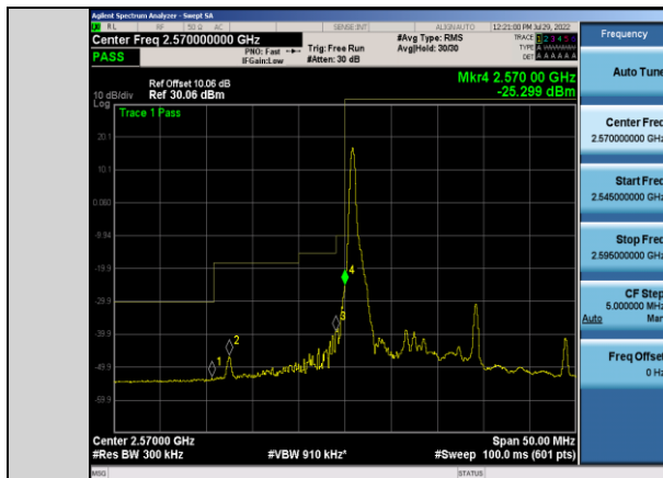
Band38-15MHz-16QAM-37825-1RB#0
