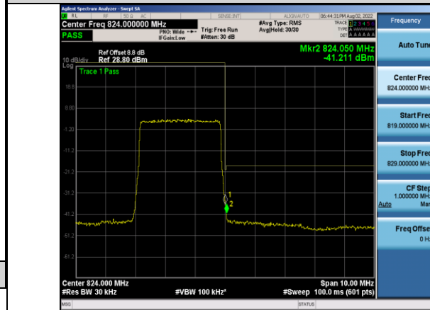
Band26-3MHz-QPSK-26775-15RB#0
