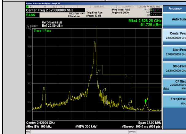
Band38-5MHz-16QAM-38225-1RB#24
