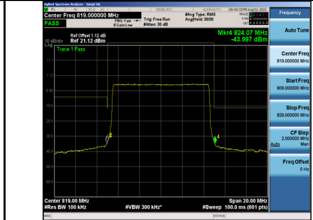
Band26-10MHz-QPSK-26740_Right-50RB#0
