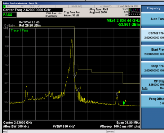
Band38-15MHz-16QAM-38175-1RB#74
