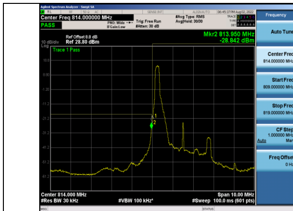
Band26-3MHz-16QAM-26705-1RB#0
