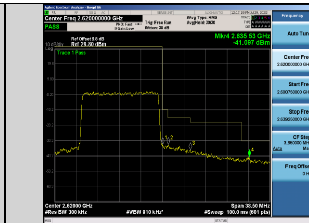
Band38-15MHz-16QAM-38175-75RB#0
