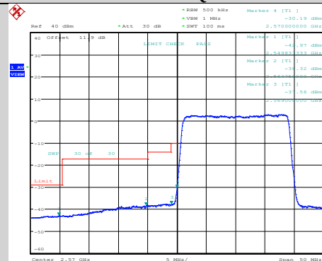
Band38-20MHz-64QAM-37850-1RB#0
