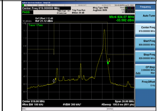
Band26-10MHz-QPSK-26740_Right-1RB#49
