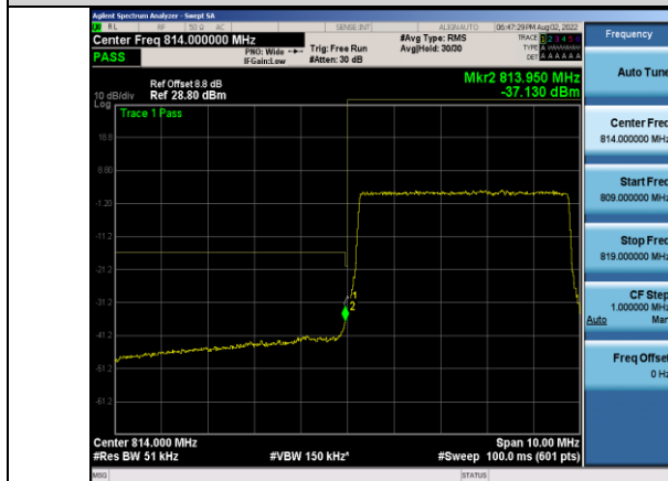
Band26-5MHz-16QAM-26715-25RB#0
