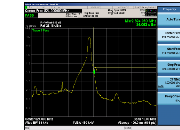
Band26-5MHz-64QAM-26765-1RB#24
