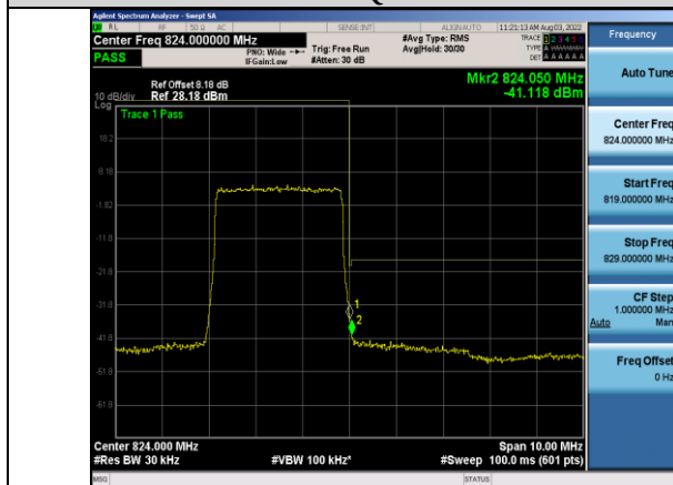
Band26-3MHz-64QAM-26775-15RB#0
