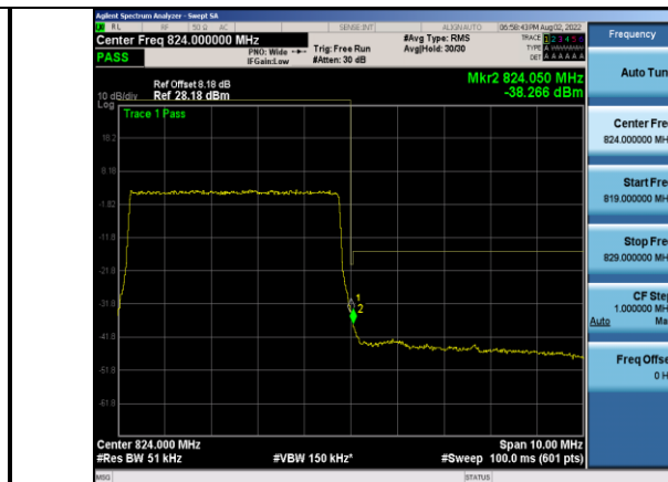
Band26-5MHz-16QAM-26765-25RB#0
