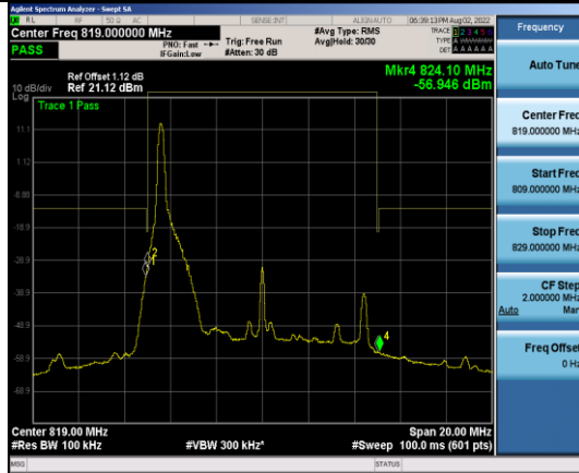
Band26-10MHz-QPSK-26740_Left-1RB#0
