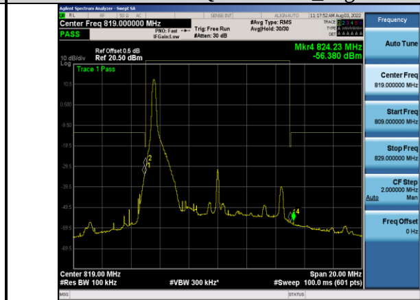
Band26-10MHz-64QAM-26740_Left-1RB#0
