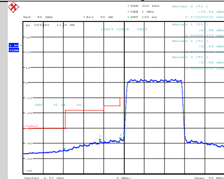
Band38-15MHz-64QAM-37825-1RB#0
