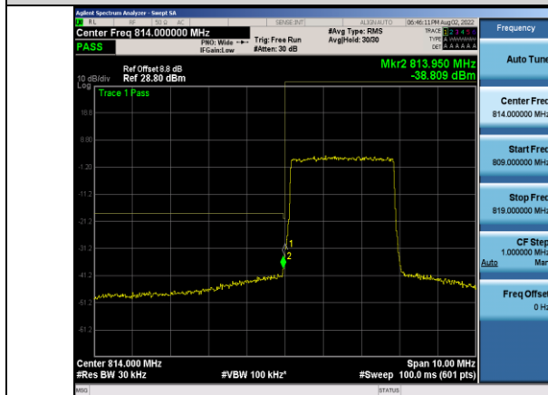
Band26-3MHz-16QAM-26705-15RB#0
