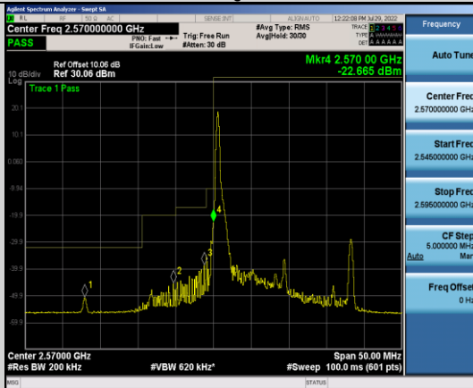
Band38-10MHz-QPSK-37800-1RB#0
