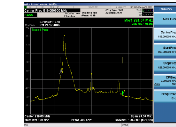
Band26-10MHz-16QAM-26740_Left-1RB#0
