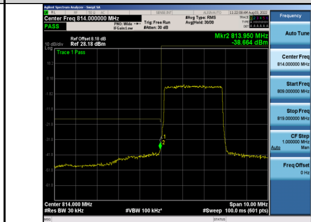
Band26-3MHz-64QAM-26705-15RB#0
