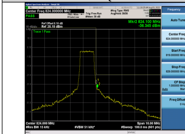
Band26-1.4MHz-64QAM-26783-6RB#0
