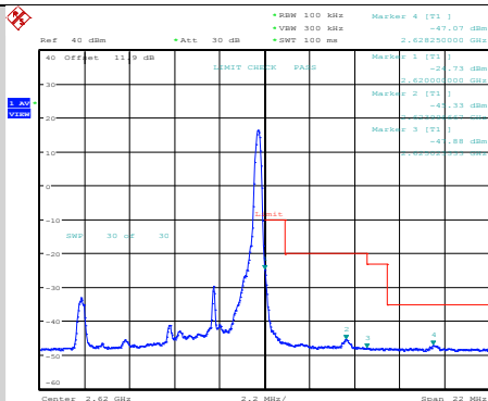
Band38-5MHz-64QAM-38225-1RB#24
