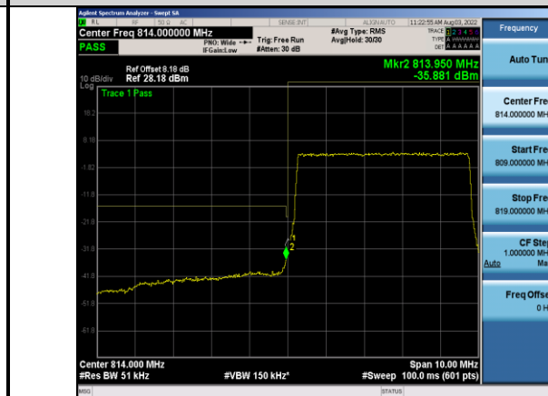
Band26-5MHz-64QAM-26715-25RB#0
