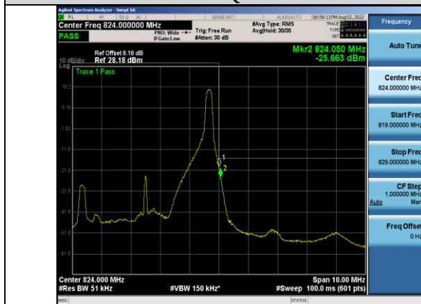
Band26-5MHz-16QAM-26765-1RB#24
