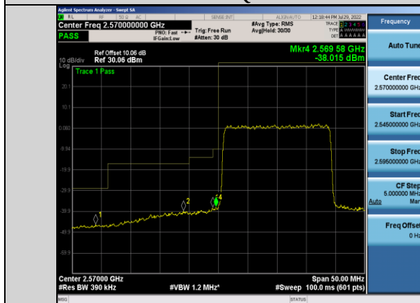
Band38-20MHz-16QAM-37850-100RB#0
