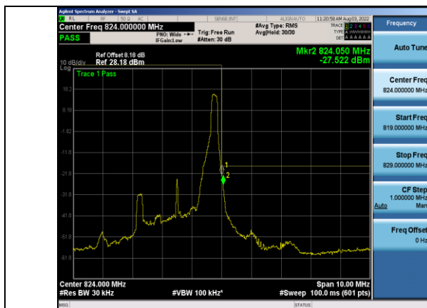
Band26-3MHz-64QAM-26775-1RB#14
