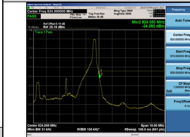
Band26-5MHz-QPSK-26765-1RB#24
