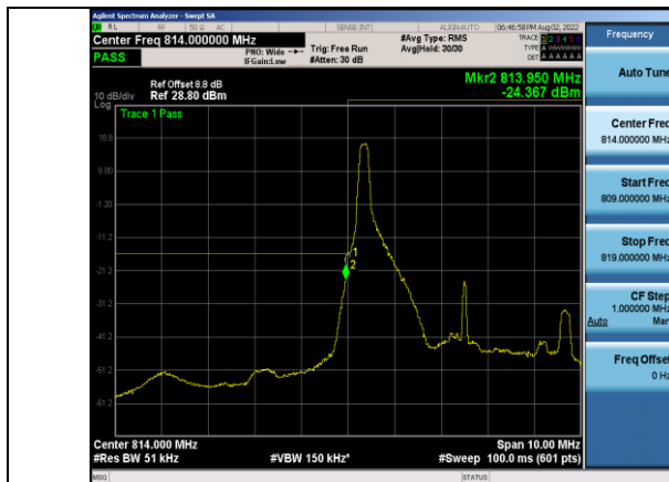
Band26-5MHz-16QAM-26715-1RB#0
