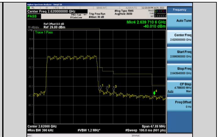
Band38-20MHz-16QAM-38150-100RB#0
