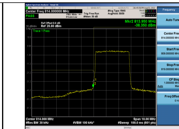
Band26-3MHz-QPSK-26705-15RB#0
