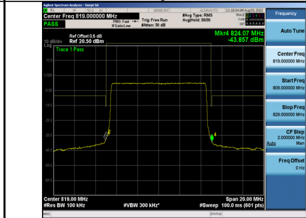
Band26-10MHz-64QAM-26740_Left-50RB#0
