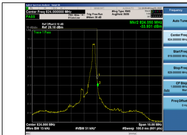
Band26-1.4MHz-64QAM-26783-1RB#5
