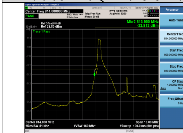
Band26-5MHz-QPSK-26715-1RB#0
