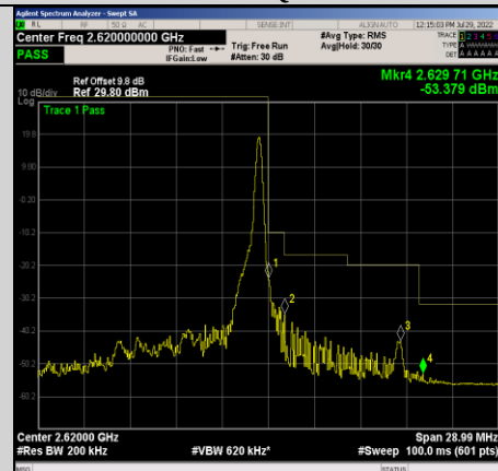
Band38-10MHz-QPSK-38200-1RB#49
