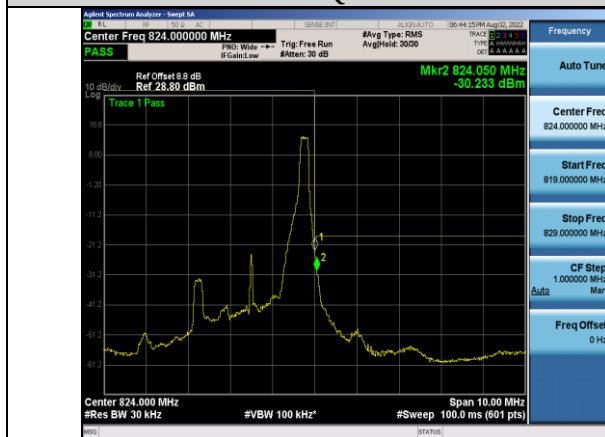
Band26-3MHz-16QAM-26775-1RB#14
