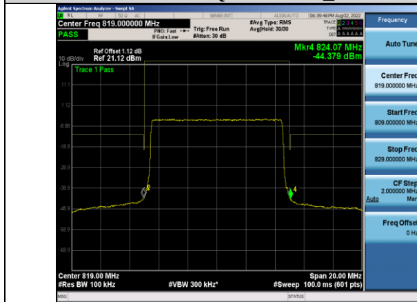
Band26-10MHz-16QAM-26740_Left-50RB#0
