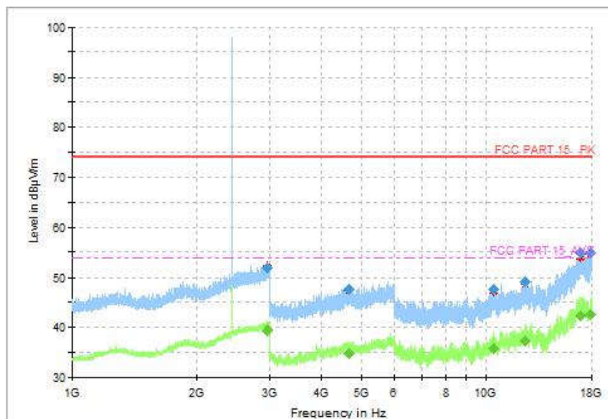
Fig.44 Radiated Spurious Emission (CH19, 1GHz ~18GHz), LE 2M
