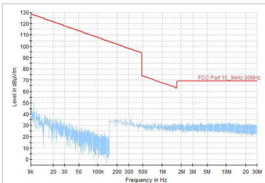
Fig.40 Radiated Spurious Emission (All Channels, 9kHz-30MHz), LE 1M
