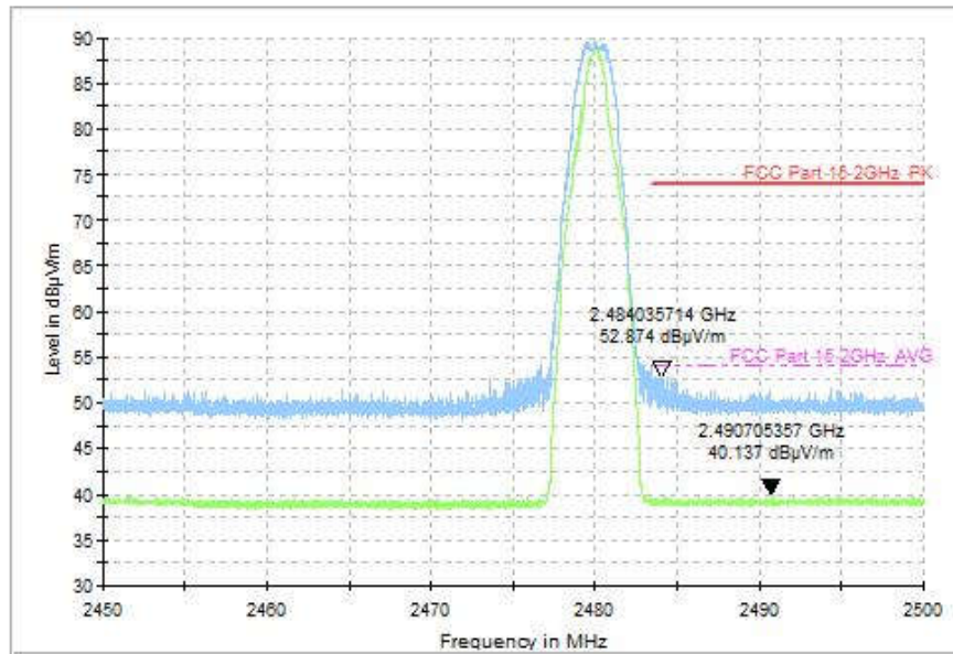
Fig.47 Radiated Band Edges (CH39, 2.45GHz~2.50GHz), LE 2M
