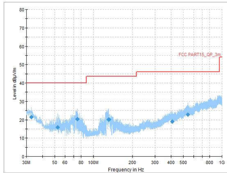
Fig.49 Radiated Spurious Emission (All Channels, 30MHz-1GHz), LE 2M
