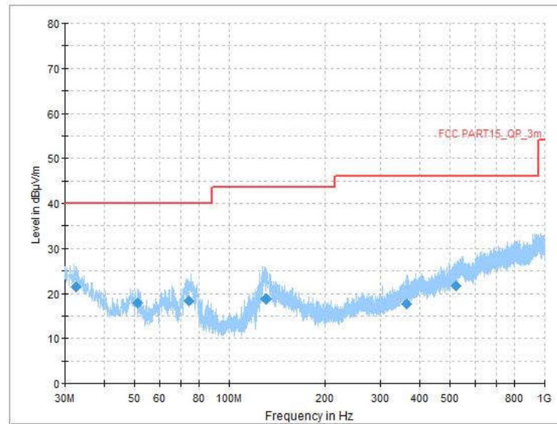
Fig.41 Radiated Spurious Emission (All Channels, 30MHz-1GHz), LE 1M
