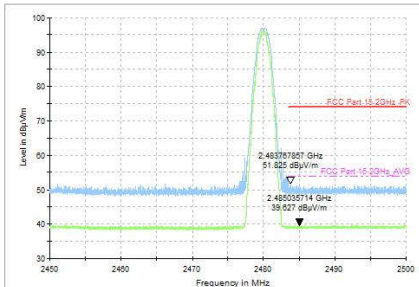
Fig.39 Radiated Band Edges (CH39, 2.45GHz~2.50GHz), LE 1M
