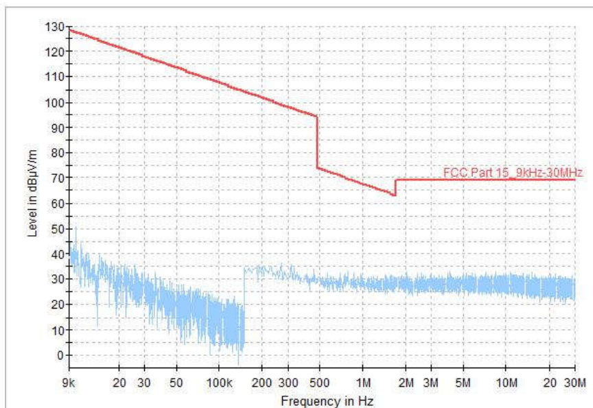
Fig.48 Radiated Spurious Emission (All Channels, 9kHz-30MHz), LE 2M
