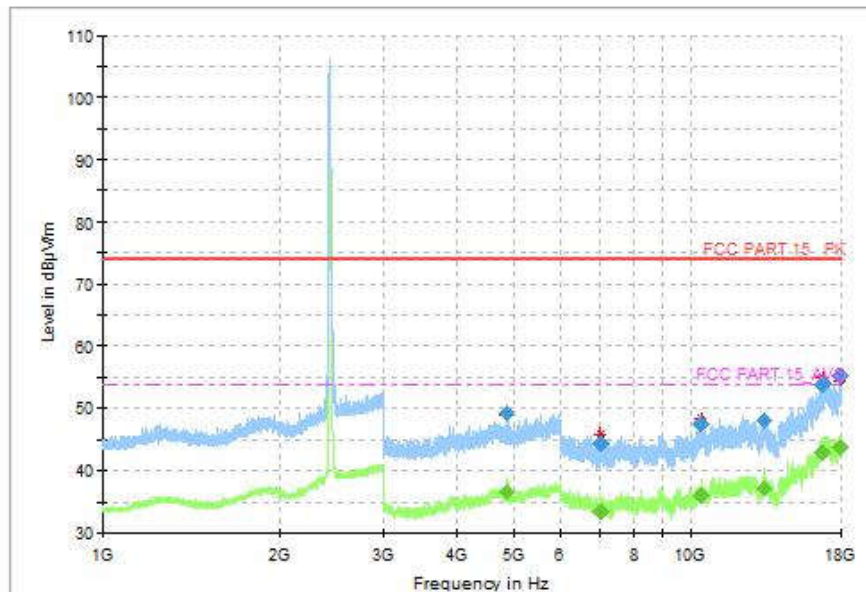
Fig.114 Radiated Spurious Emission (802.11n-HT20, CH6, 1GHz-18GHz)
