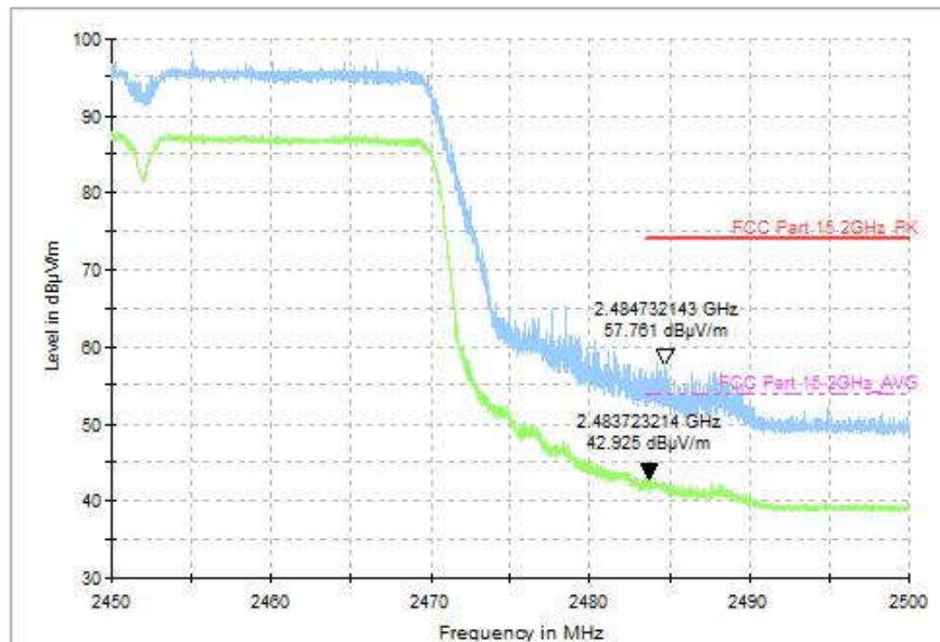
Fig.132 Radiated Spurious Emission (802.11-VHT40, CH9, 2.45GHz~2.50GHz)
