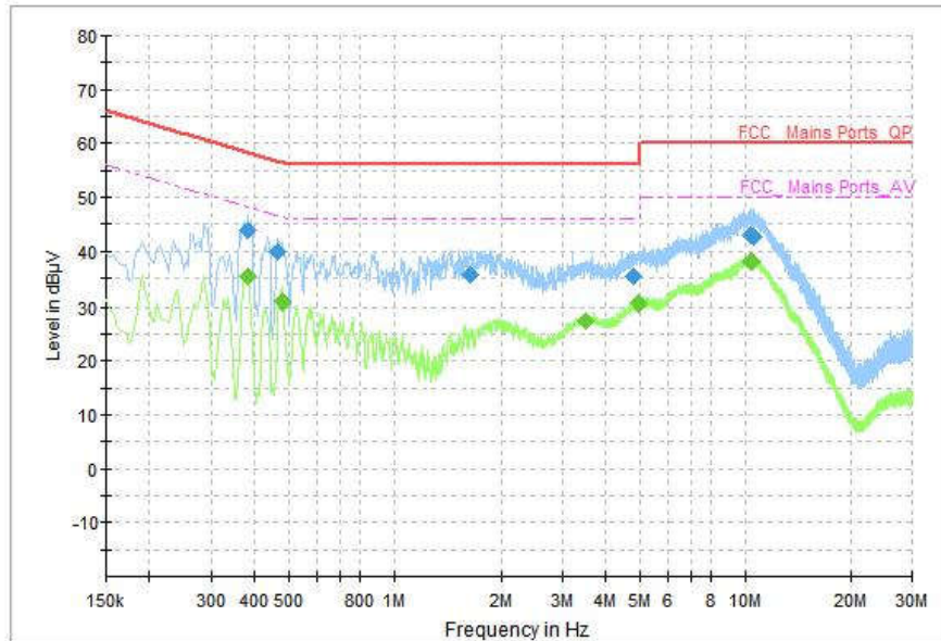
Fig.136 AC Power line Conducted Emission (Traffic)
