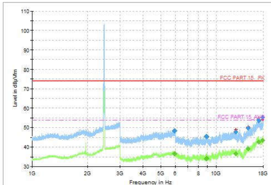
Fig.110 Radiated Spurious Emission (802.11g, CH11, 1GHz-18GHz)
