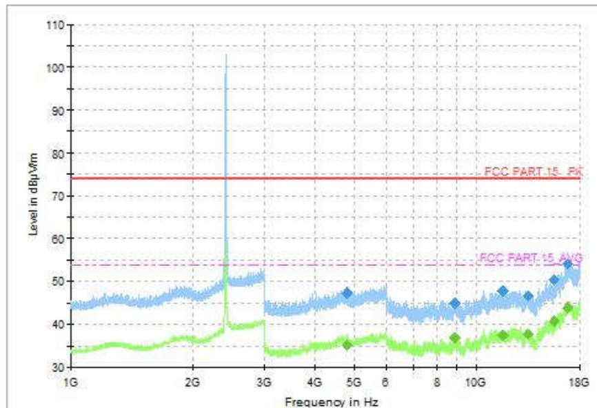
Fig.108 Radiated Spurious Emission (802.11g, CH1, 1GHz-18GHz)
