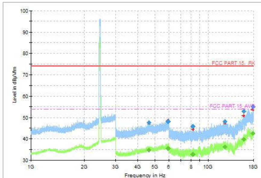
Fig.130 Radiated Spurious Emission (802.11-VHT40, CH9, 1GHz-18GHz)
