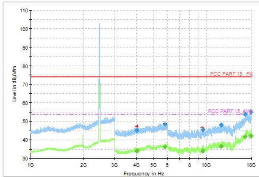
Fig.115 Radiated Spurious Emission (802.11n-HT20, CH11, 1GHz-18GHz)
