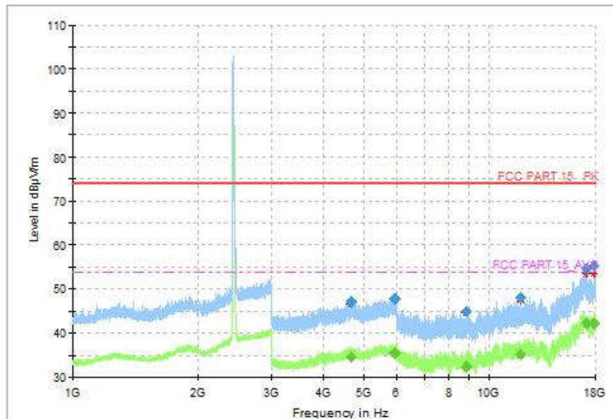
Fig.124 Radiated Spurious Emission (802.11-VHT20, CH6, 1GHz-18GHz)
