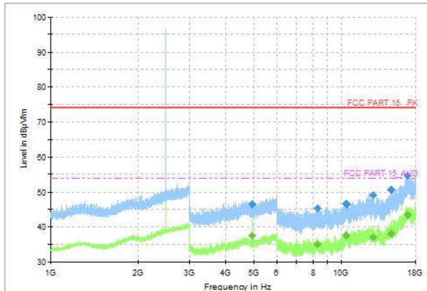
Fig. 52 Radiated Spurious Emission (8DPSK, CH78, 1GHz ~18GHz)
