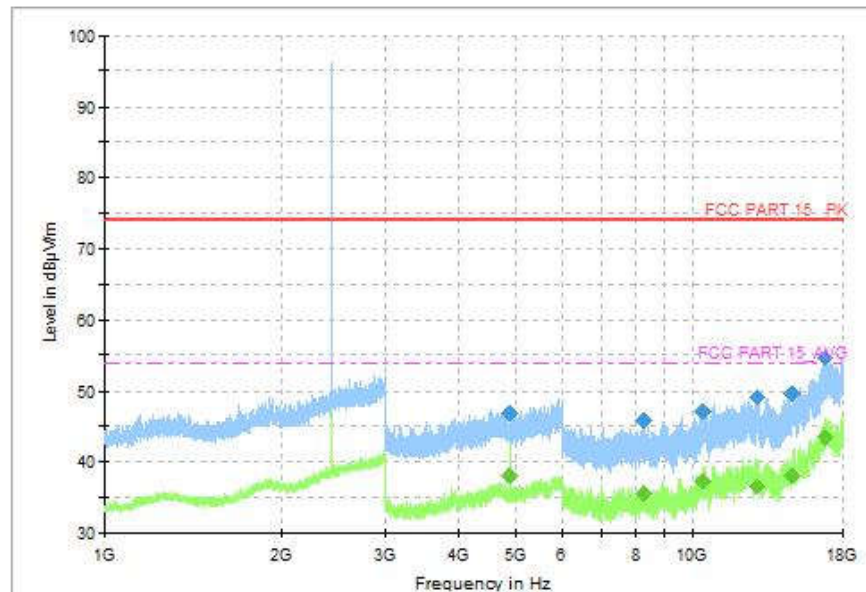
Fig. 51 Radiated Spurious Emission (8DPSK, CH39, 1GHz ~18GHz)
