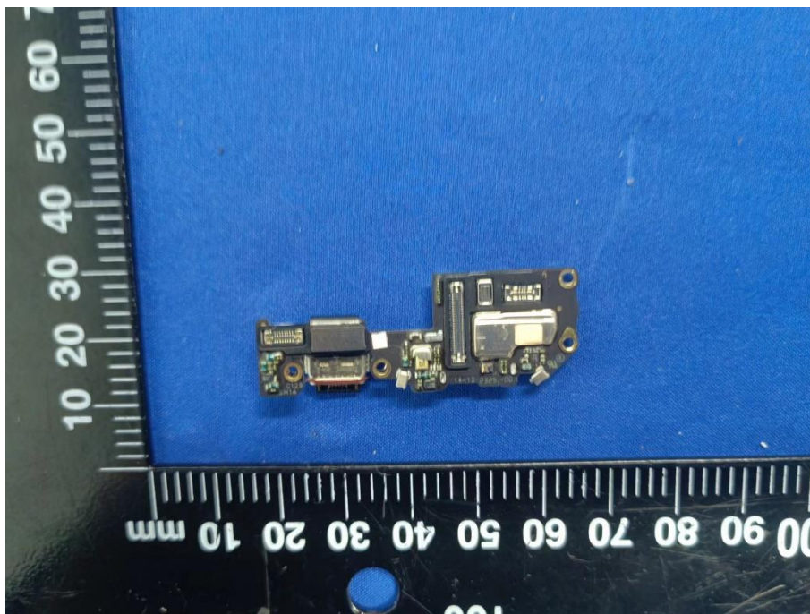
SECONDARY BOARD REAR VIEW (WITH SHIELDING)
