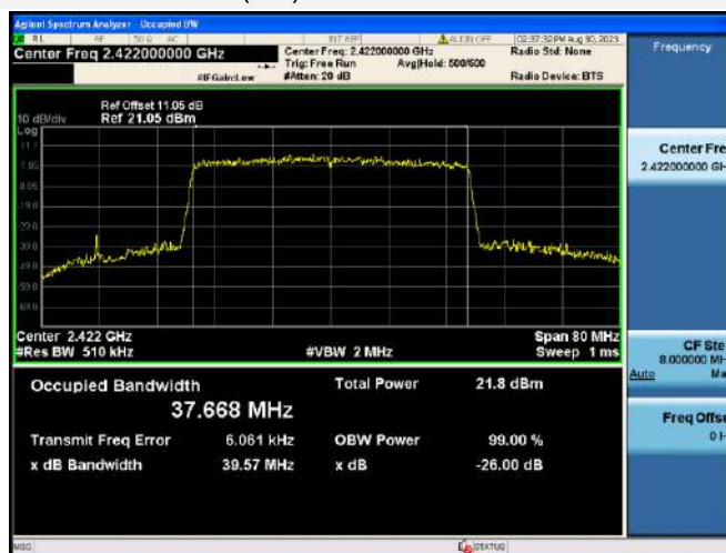
802.11ax-40 MHz(SU) CHANNEL 3
