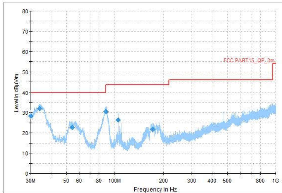
Fig. 106 Transmitter Spurious Emission (All channel, 30MHz~1GHz)
