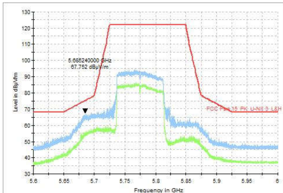
Fig. 79 Band Edges (802.11ac-VHT80, CH155 5775MHz)
