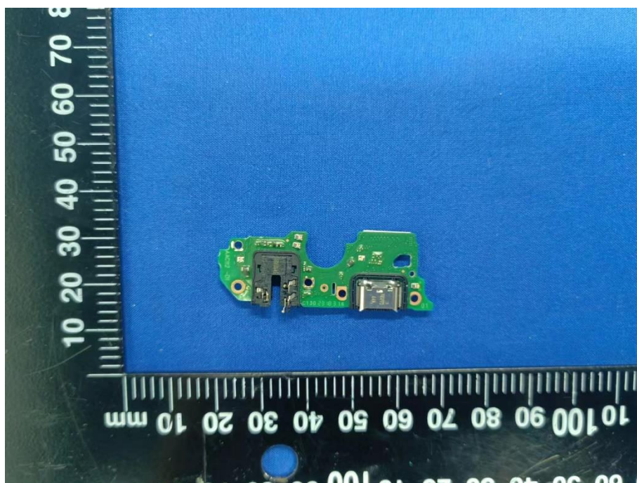
SUB BOARD REAR VIEW (WITHOUT SHIELDING)
