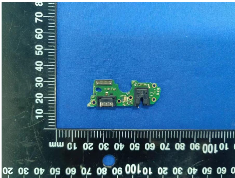
SUB BOARD TOP VIEW (WITHOUT SHIELDING)
