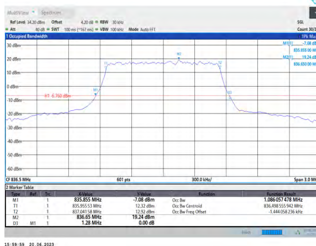
Band26-1.4MHz-QPSK-26915-6RB#0
