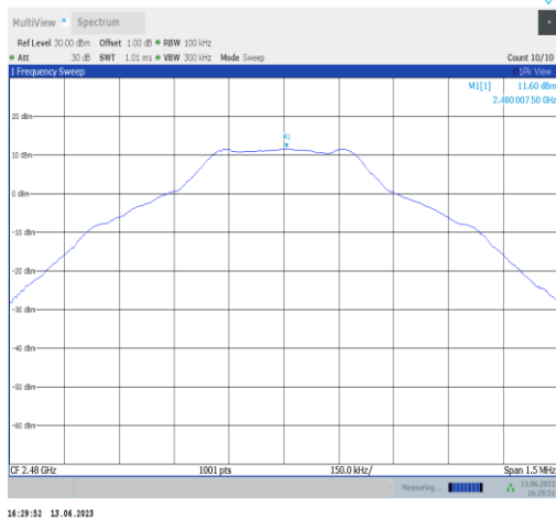
DH5-Ant2-2480-0~Reference
