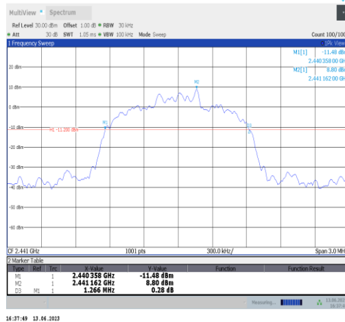
3DH5-Ant2-2441
