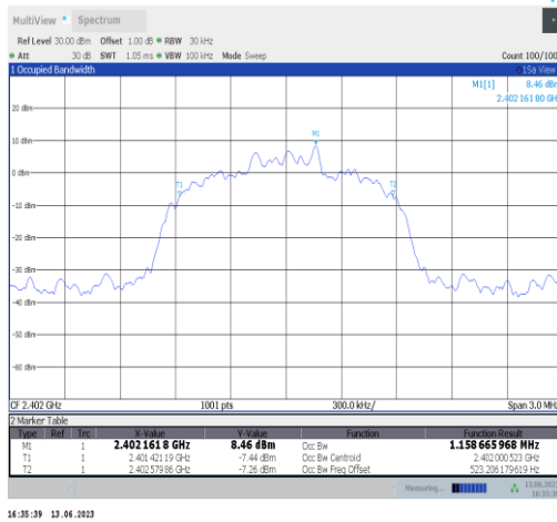
3DH5-Ant2-2402
