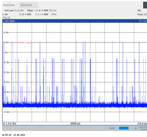
2DH3-Ant2-Hop
