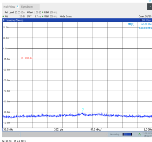
2DH5-Ant2-2402-30~1000
