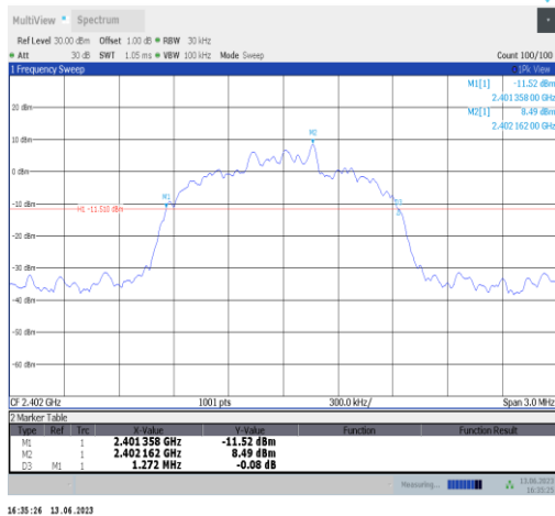
3DH5-Ant2-2402
