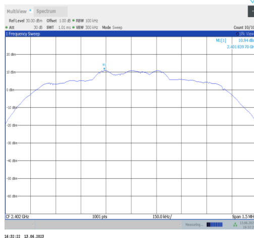
2DH5-Ant2-2402-0~Reference
