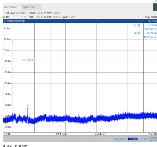
2DH5-Ant2-2480-1000~26500
