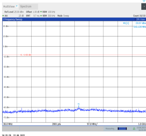
DH5-Ant2-2441-30~1000
