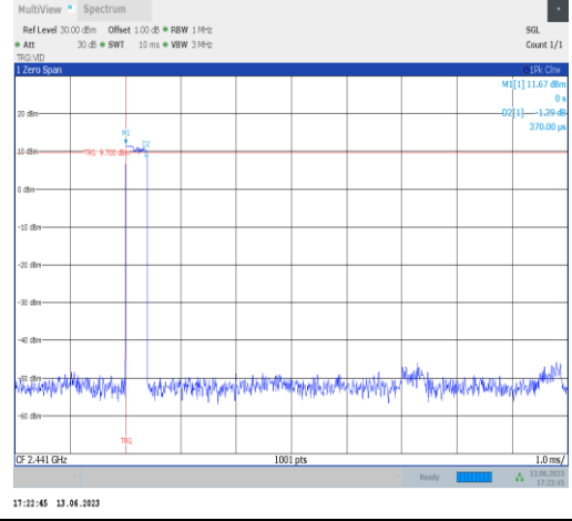
3DH1-Ant2-Hop
