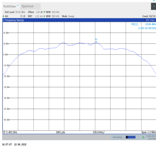
3DH5-Ant2-2402-0~Reference
