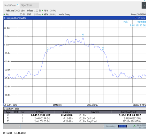
3DH5-Ant2-2441
