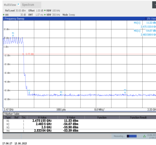
2DH5-Ant2-Hop_2480
