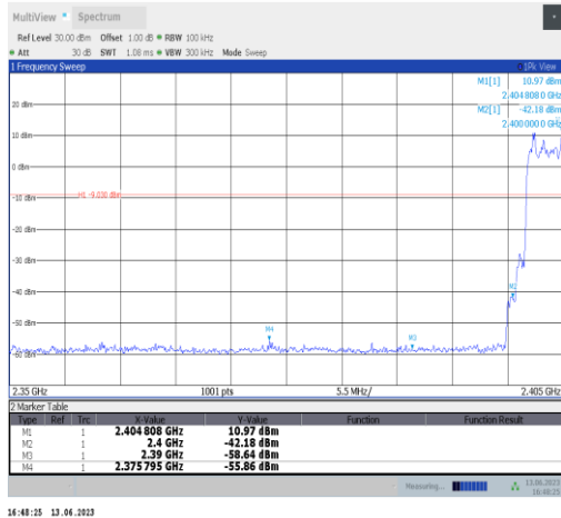
2DH5-Ant2-Hop_2402
