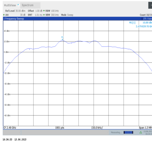
2DH5-Ant2-2480-0~Reference
