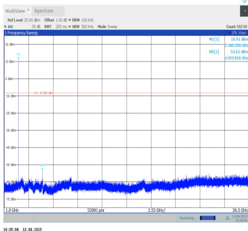
DH5-Ant2-2480-1000~26500
