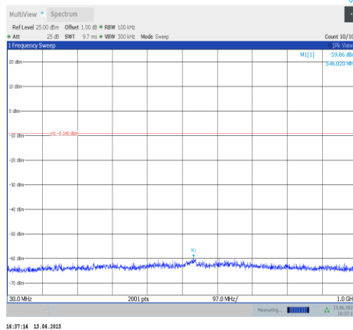
3DH5-Ant2-2402-30~1000
