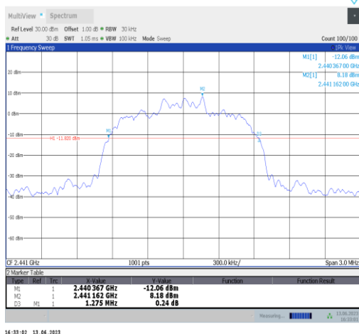
2DH5-Ant2-2441
