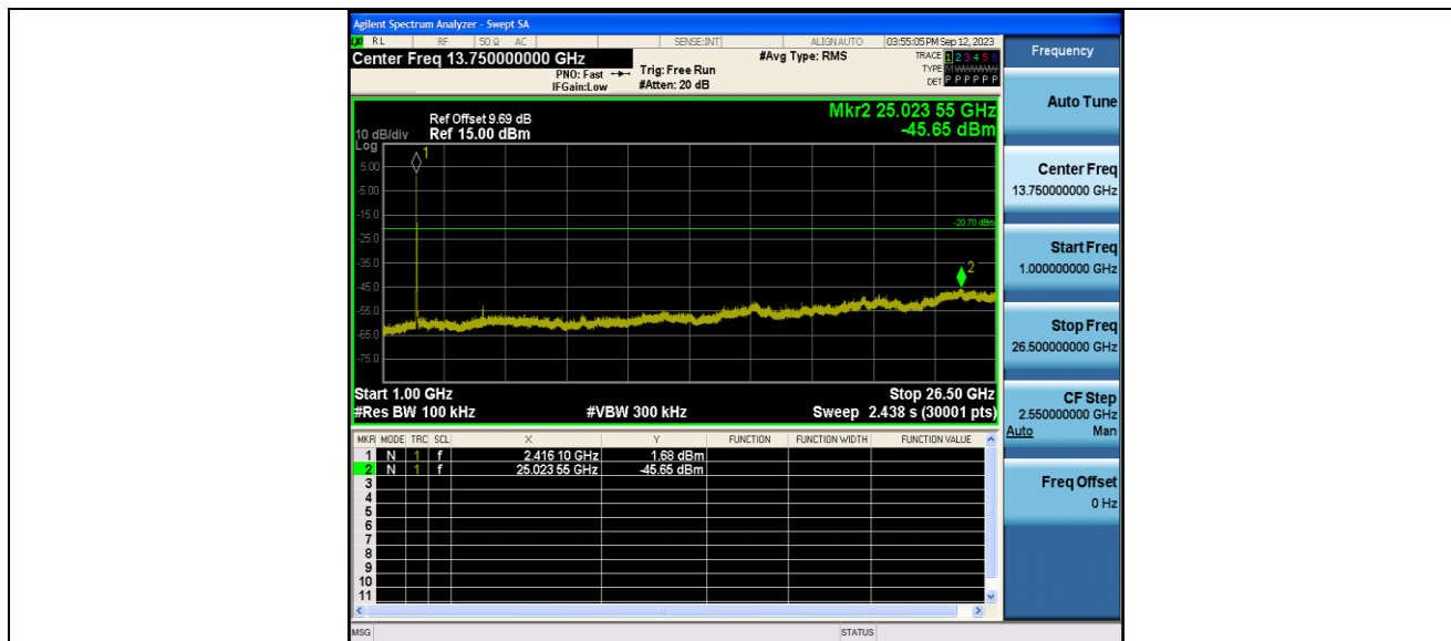
11n20MIMO Ant10_2412_0~Reference
