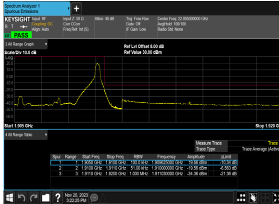
N2(5M)_DFT-s- OFDM_QPSK_Edge_1RB_Right_High_CH
