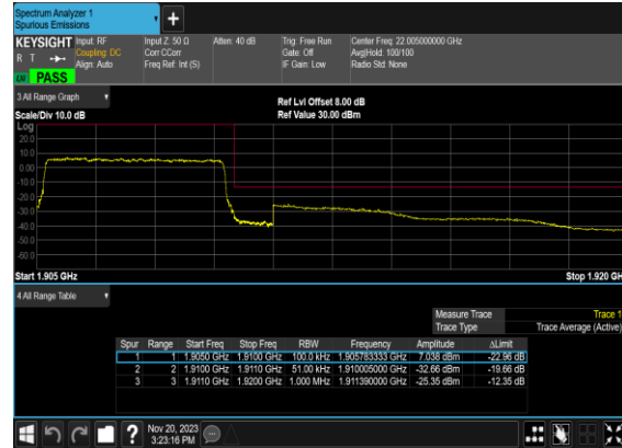
N2(5M)_DFT-s- OFDM_QPSK_Outer_Full_High_CH
