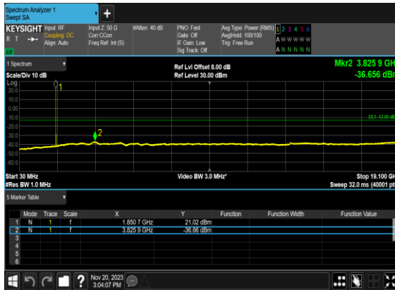
N2(5M)_DFT-s- OFDM_QPSK_Edge_1RB_Left_Low_CH
