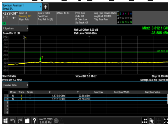
N2(10M)_DFT-s- OFDM_QPSK_Edge_1RB_Left_Mid_CH
