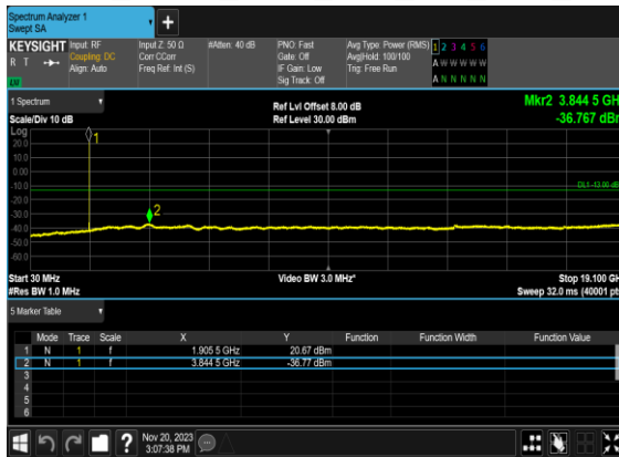
N2(5M)_DFT-s- OFDM_QPSK_Edge_1RB_Left_High_CH
