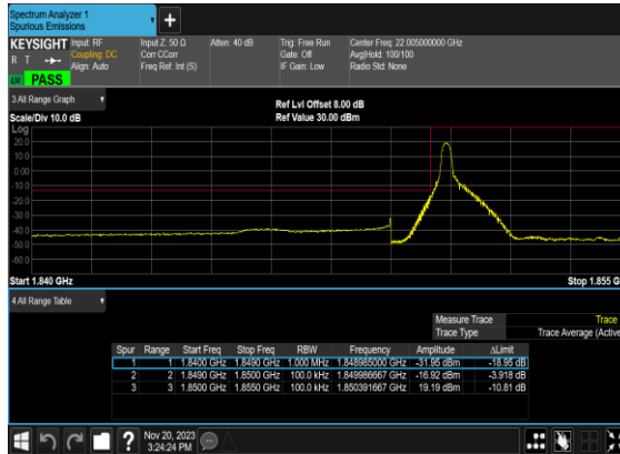
N2(10M)_DFT-s- OFDM_QPSK_Edge_1RB_Left_Low_CH
