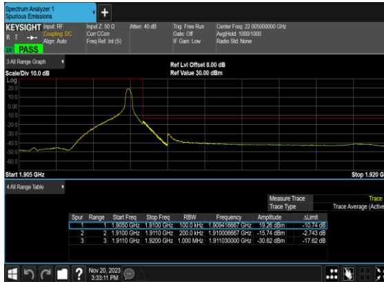
N2(20M)_DFT-s- OFDM_QPSK_Edge_1RB_Right_High_CH
