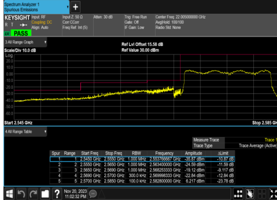
B4_N38(15M)_DFT-s- OFDM_QPSK_Outer_Full_Low_CH
