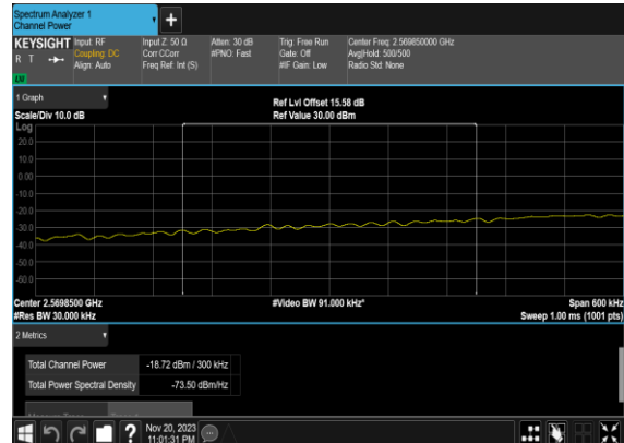
B4_N38(15M)_DFT-s- OFDM_QPSK_Edge_1RB_Left_Low_CH_PASS
