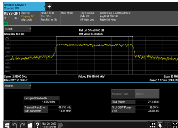
B4_N38(15M)_CP-OFDM_16 QAM_Outer_Full_Mid_CH
