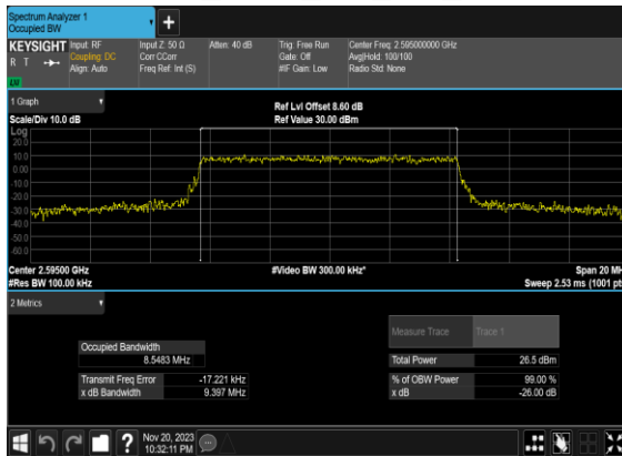
B4_N38(10M)_CP-OFDM_64 QAM_Outer_Full_Mid_CH
