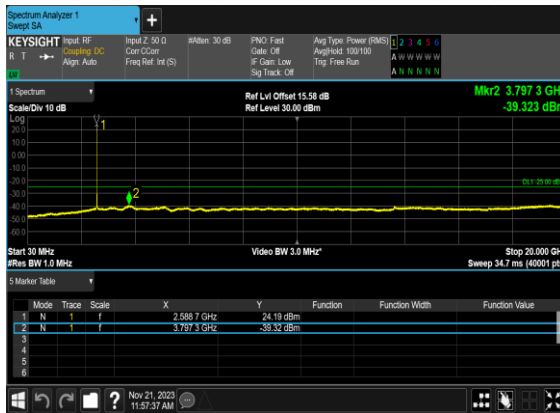
B4_N38(15M)_DFT-s-OFDM_QPSK_Edge_1RB_Left_Mid_CH
