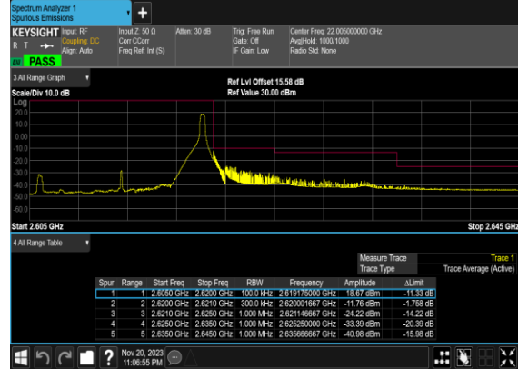
B4_N38(15M)_DFT-s- OFDM_QPSK_Edge_1RB_Right_High_CH
