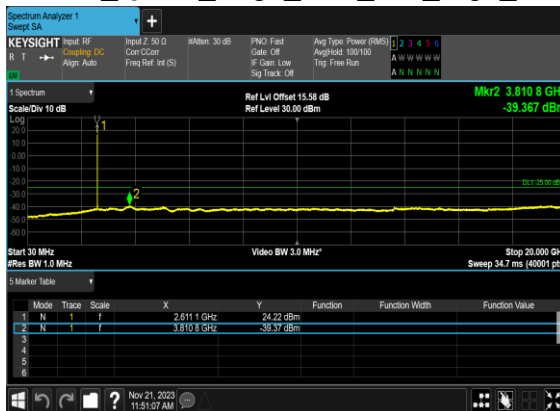
B4_N38(10M)_DFT-s-OFDM_QPSK_Edge_1RB_Left_High_CH
