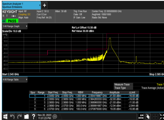
B4_N38(15M)_DFT-s- OFDM_QPSK_Edge_1RB_Left_Low_CH
