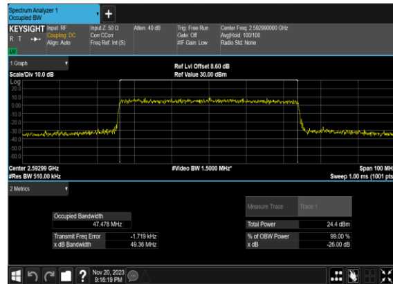
B4_N41(50M)_CP-OFDM_256 QAM_Outer_Full_Mid_CH
