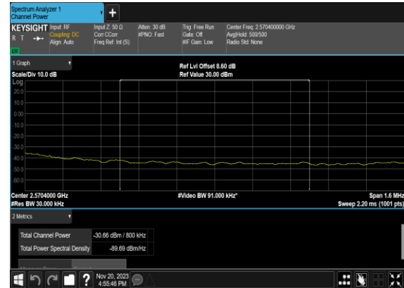
N7(40M)_DFT-s- OFDM_QPSK_Outer_Full_High_CH_CHP_PASS
