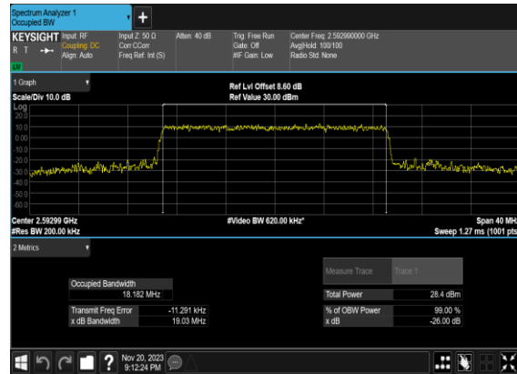
B4_N41(20M)_CP-OFDM_16 QAM_Outer_Full_Mid_CH
