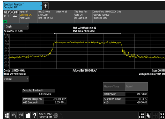
B4_N38(10M)_CP-OFDM_256 QAM_Outer_Full_Mid_CH
