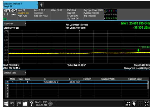
B4_N38(10M)_DFT-s-OFDM_QPSK_Edge_1RB_Left_Low_CH
