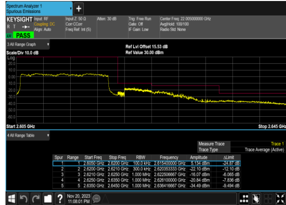
B4_N38(15M)_DFT-s- OFDM_QPSK_Outer_Full_High_CH
