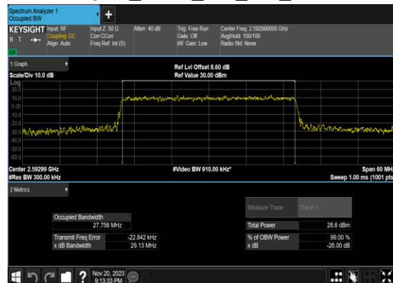
B4_N41(30M)_CP-OFDM_16 QAM_Outer_Full_Mid_CH
