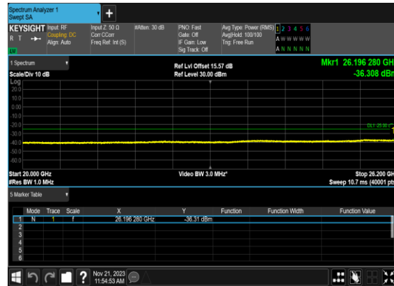
B4_N38(15M)_DFT-s-OFDM_QPSK_Edge_1RB_Left_Low_CH
