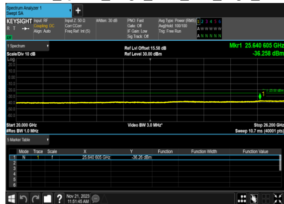
B4_N38(10M)_DFT-s-OFDM_QPSK_Edge_1RB_Left_High_CH
