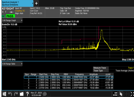
B4_N38(10M)_DFT-s- OFDM_QPSK_Edge_1RB_Left_Low_CH
