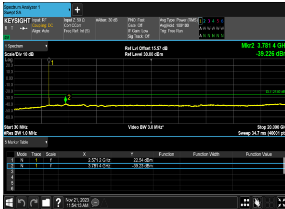
B4_N38(15M)_DFT-s-OFDM_QPSK_Edge_1RB_Left_Low_CH
