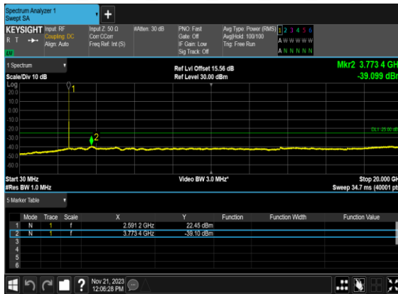
B4_N38(10M)_DFT-s-OFDM_QPSK_Edge_1RB_Left_Mid_CH
