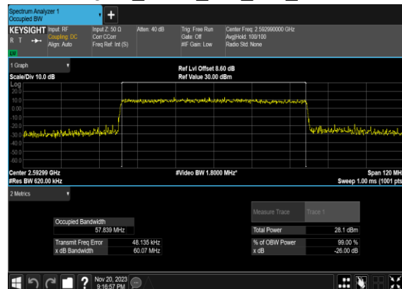
B4_N41(60M)_CP-OFDM_16 QAM_Outer_Full_Mid_CH
