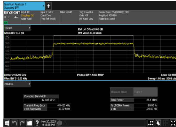
B4_N41(50M)_CP-OFDM_16 QAM_Outer_Full_Mid_CH
