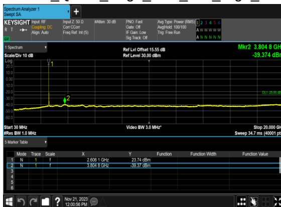
B4_N38(15M)_DFT-s-OFDM_QPSK_Edge_1RB_Left_High_CH
