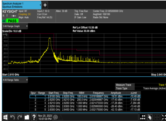
B4_N38(10M)_DFT-s- OFDM_QPSK_Edge_1RB_Right_High_CH
