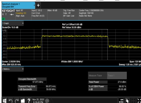
B4_N41(60M)_CP- OFDM_QPSK_Outer_Full_Mid_CH
