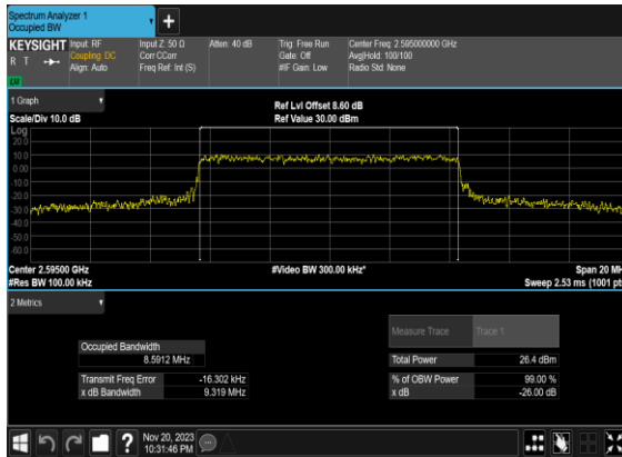
B4_N38(10M)_CP- OFDM_QPSK_Outer_Full_Mid_CH
