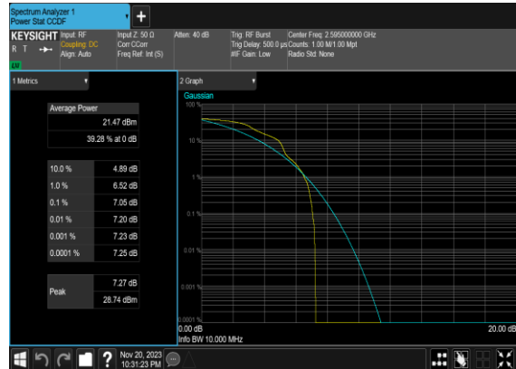
B4_N38(10M)_DFT-s-OFDM_QPSK_Edge_1RB_Left_Mid_CH
