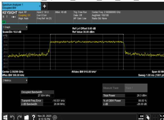
B4_N41(30M)_CP- OFDM_QPSK_Outer_Full_Mid_CH
