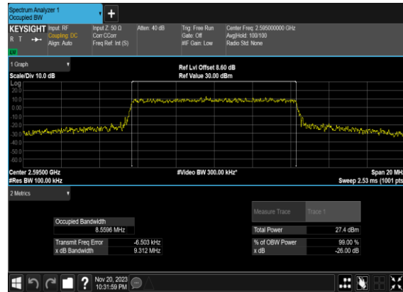
B4_N38(10M)_CP-OFDM_16 QAM_Outer_Full_Mid_CH
