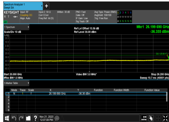
B4_N38(10M)_DFT-s-OFDM_QPSK_Edge_1RB_Left_Mid_CH
