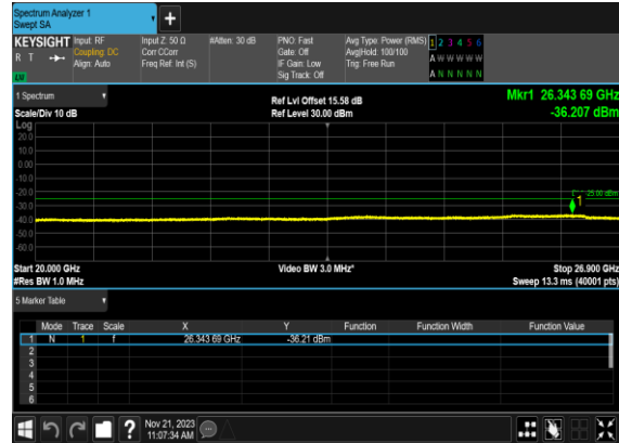
B4_N41(60M)_DFT-s-OFDM_QPSK_Edge_1RB_Left_Low_CH
