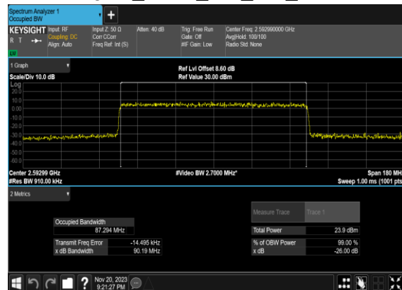
B4_N41(90M)_CP-OFDM_256 QAM_Outer_Full_Mid_CH
