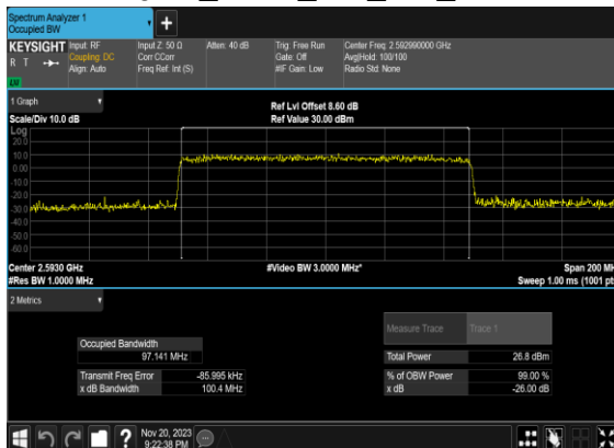
B4_N41(100M)_CP-OFDM_64 QAM_Outer_Full_Mid_CH
