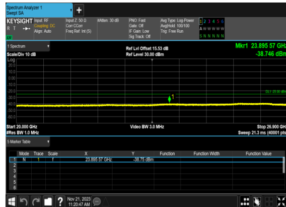
B4_N41(100M)_DFT-s-OFDM_QPSK_Edge_1RB_Left_Mid_CH
