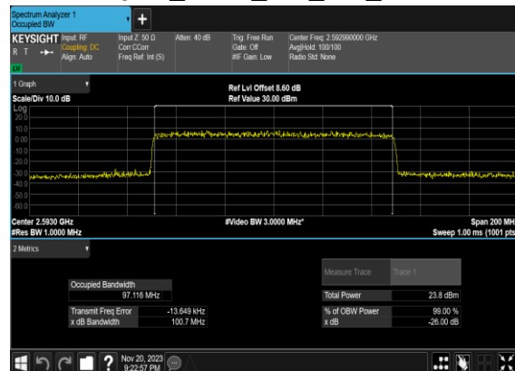
B4_N41(100M)_CP-OFDM_256 QAM_Outer_Full_Mid_CH
