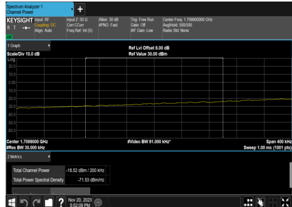
N66(20M)_DFT-s- OFDM_QPSK_Edge_1RB_Left_Low_CH_chp _PASS
