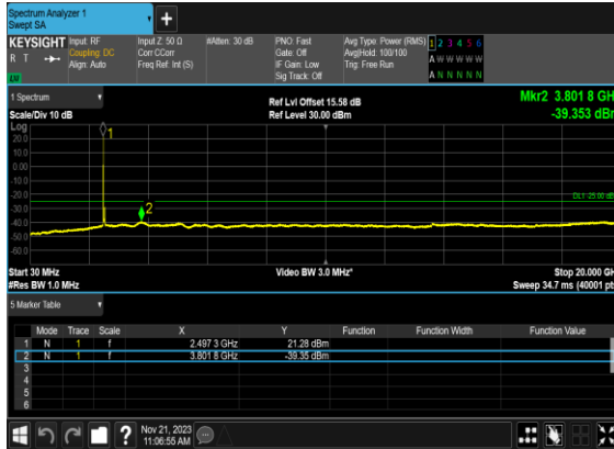
B4_N41(60M)_DFT-s-OFDM_QPSK_Edge_1RB_Left_Low_CH
