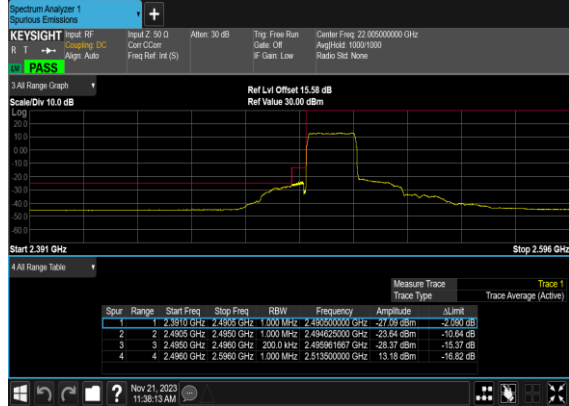
B4_N41(20M)_DFT-s- OFDM_QPSK_Outer_Full_Low_CH
