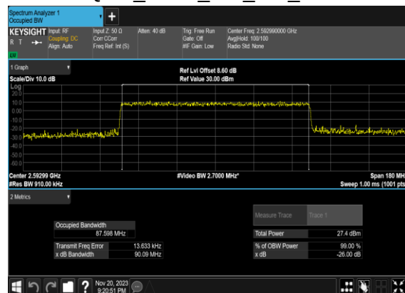
B4_N41(90M)_CP-OFDM_16 QAM_Outer_Full_Mid_CH
