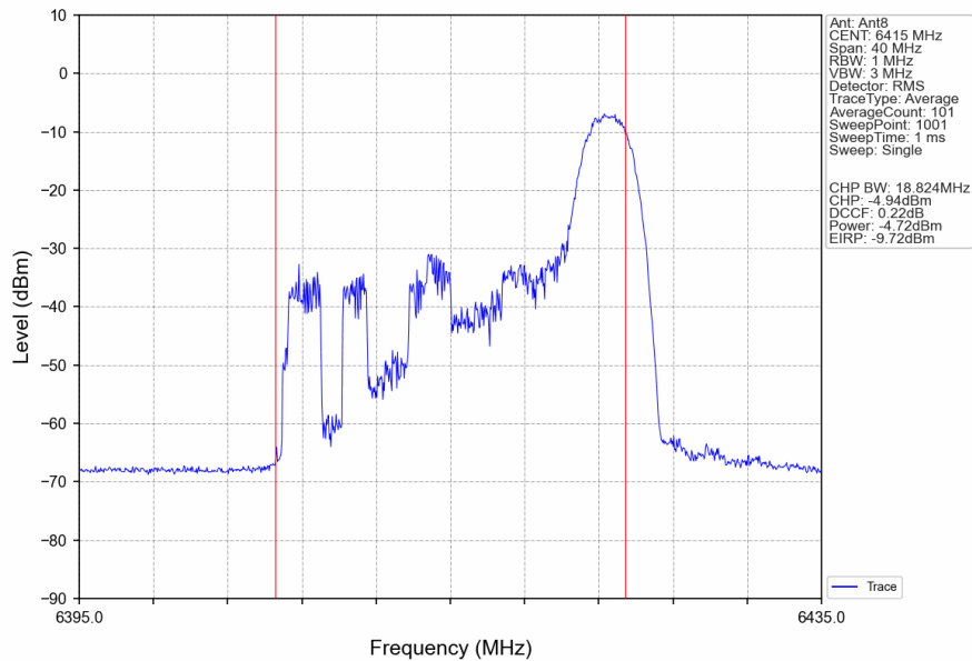
802.11ax(HEW20)_HCH_6415MHz_RU26_Right_Ant8_NTNV
