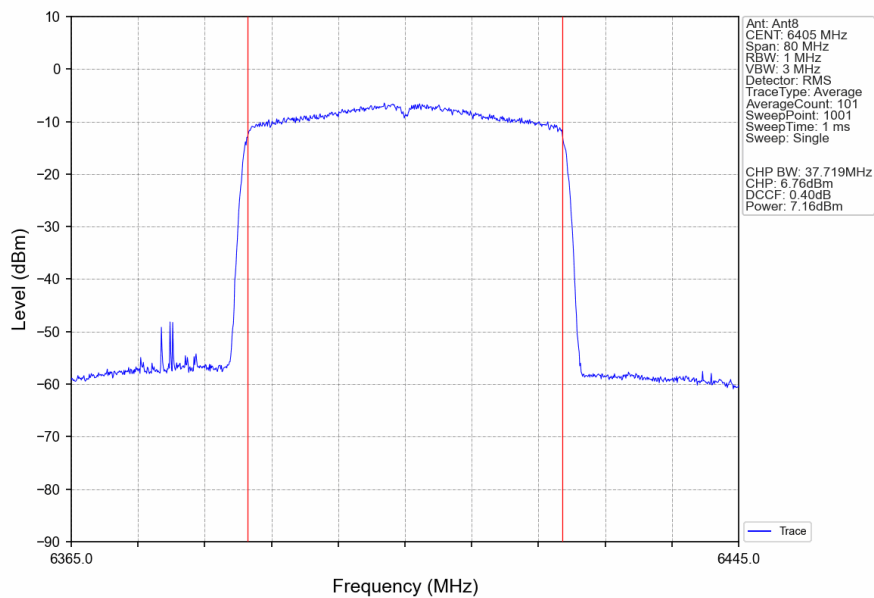
802.11ax(HEW40)_HCH_6405MHz_RU484_Left_Ant8_NTNV
