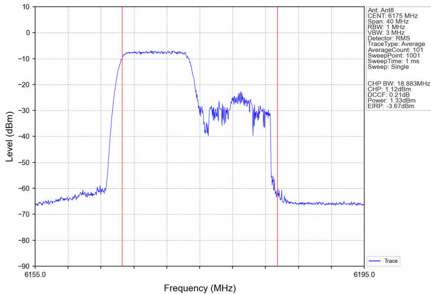
802.11ax(HEW20)_MCH_6175MHz_RU106_Left_Ant8_NTNV
