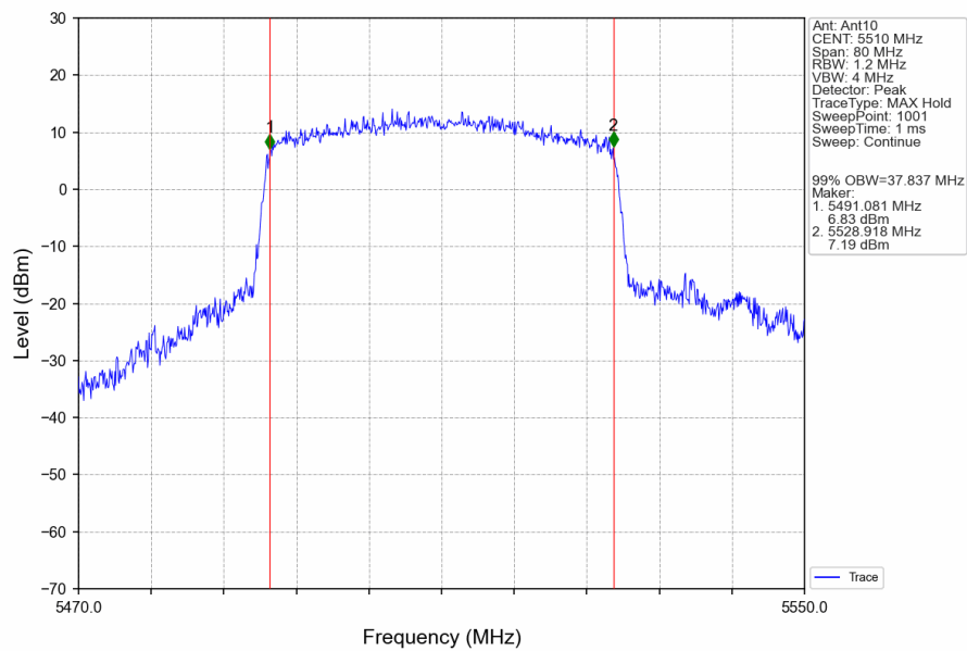
802.11ax(HEW40) LCH 5510MHz RU484 Left Ant10 NTN
