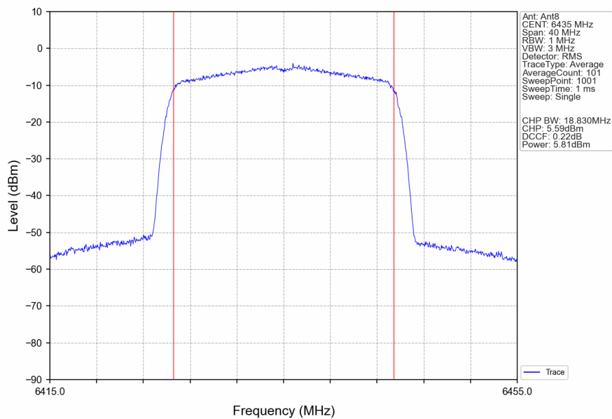
802.11ax(HEW20)_LCH_6435MHz_RU242_Left_Ant8_NTNV
