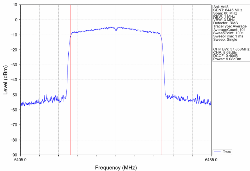
802.11ax(HEW40)_LCH_6445MHz_RU484_Left_Ant8_NTNV
