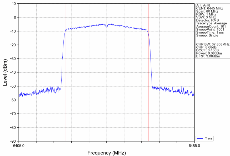
802.11ax(HEW40)_LCH_6445MHz_RU484_Left_Ant8_NTNV
