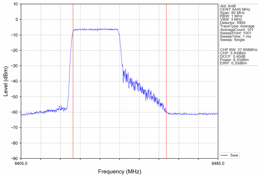
802.11ax(HEW40)_LCH_6445MHz_RU242_Left_Ant8_NTNV
