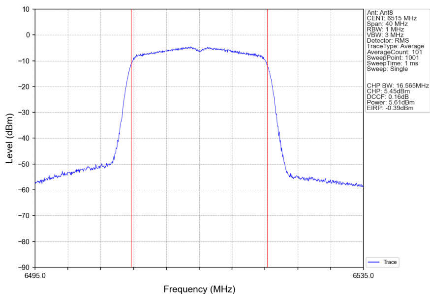
802.11a_HCH_6515MHz_Ant8_NTNV
