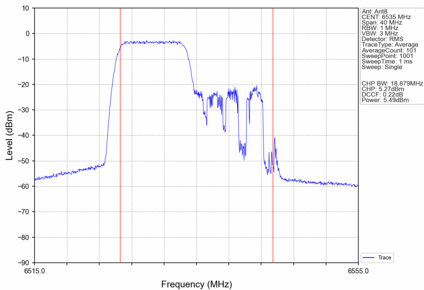
802.11ax(HEW20)_LCH_6535MHz_RU106_Left_Ant8_NTNV
