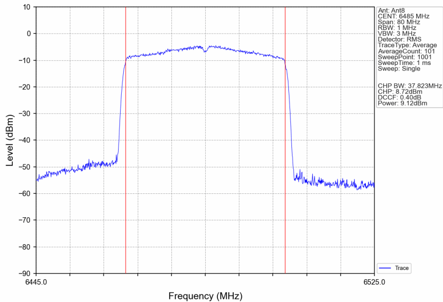
802.11ax(HEW40)_MCH_6485MHz_RU484_Left_Ant8_NTNV
