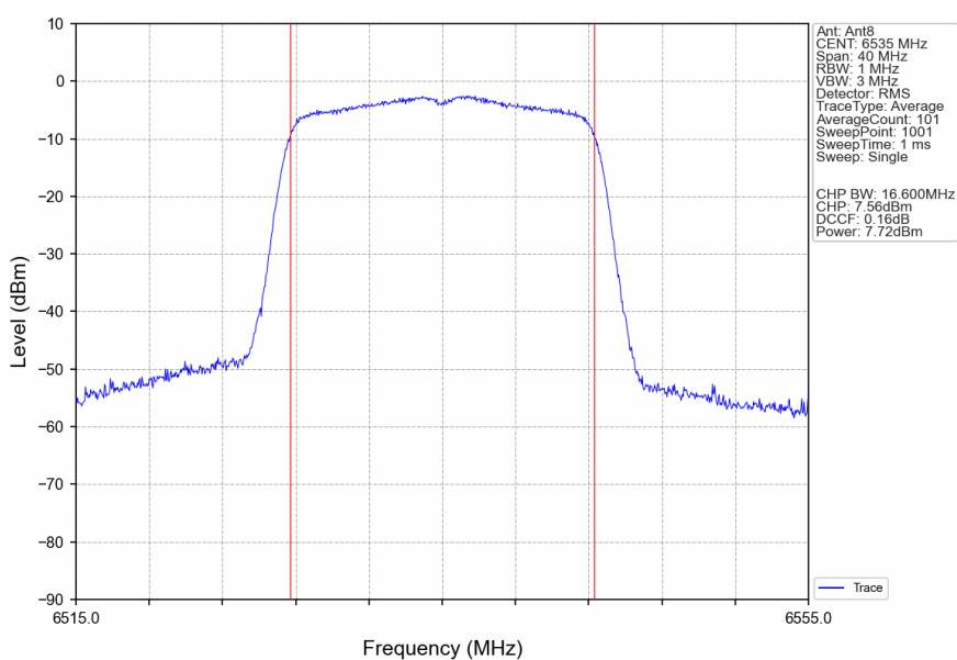
802.11a_LCH_6535MHz_Ant8_NTNV
