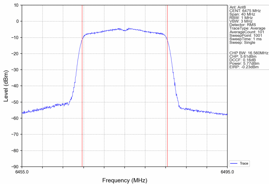
802.11a_MCH_6475MHz_Ant8_NTNV
