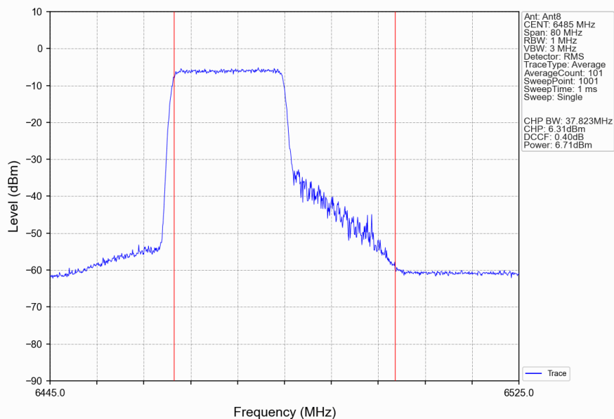
802.11ax(HEW40)_MCH_6485MHz_RU242_Left_Ant8_NTNV
