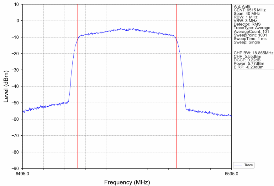
802.11ax(HEW20)_HCH_6515MHz_RU242_Left_Ant8_NTNV
