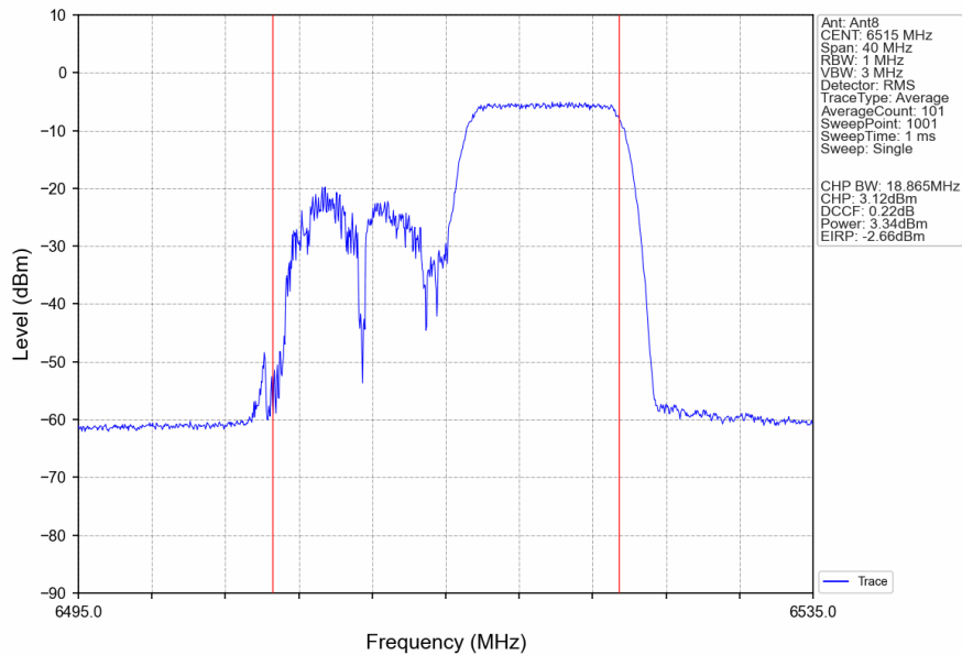
802.11ax(HEW20)_HCH_6515MHz_RU106_Right_Ant8_NTNV
